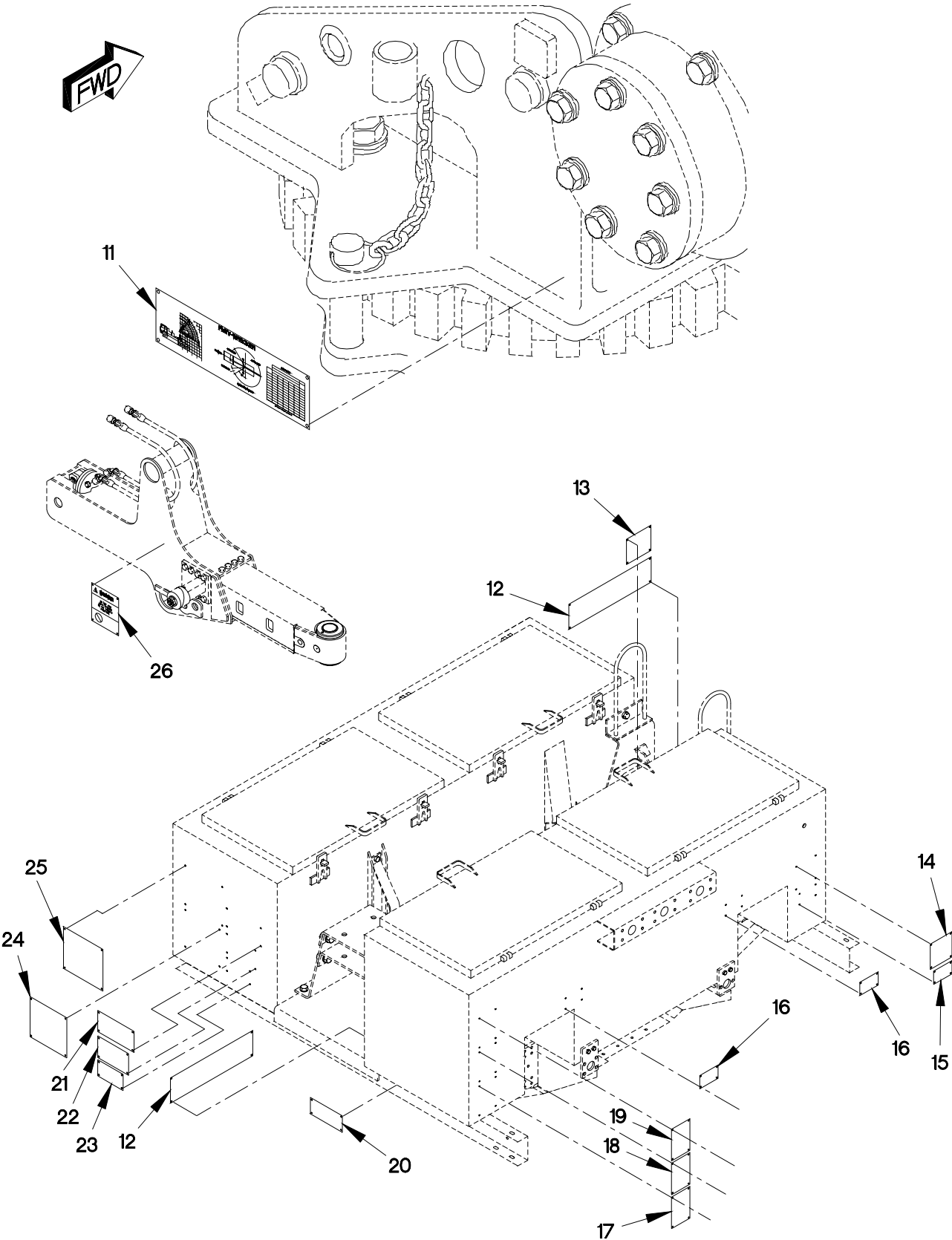
FIGURE 435. M1089 DECALS AND DATA PLATES (SHEET 2 OF 2)
