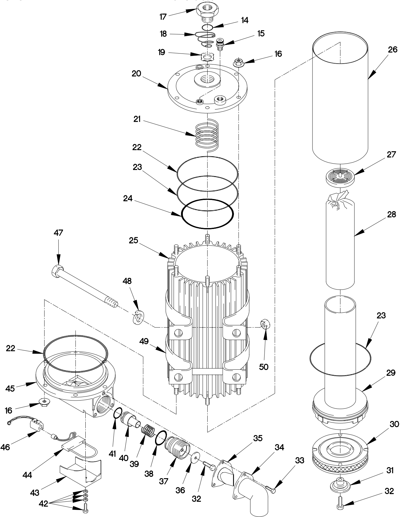
FIGURE 498. AIR DRYER, HOSES AND FITTINGS (SHEET 2 OF 2)
