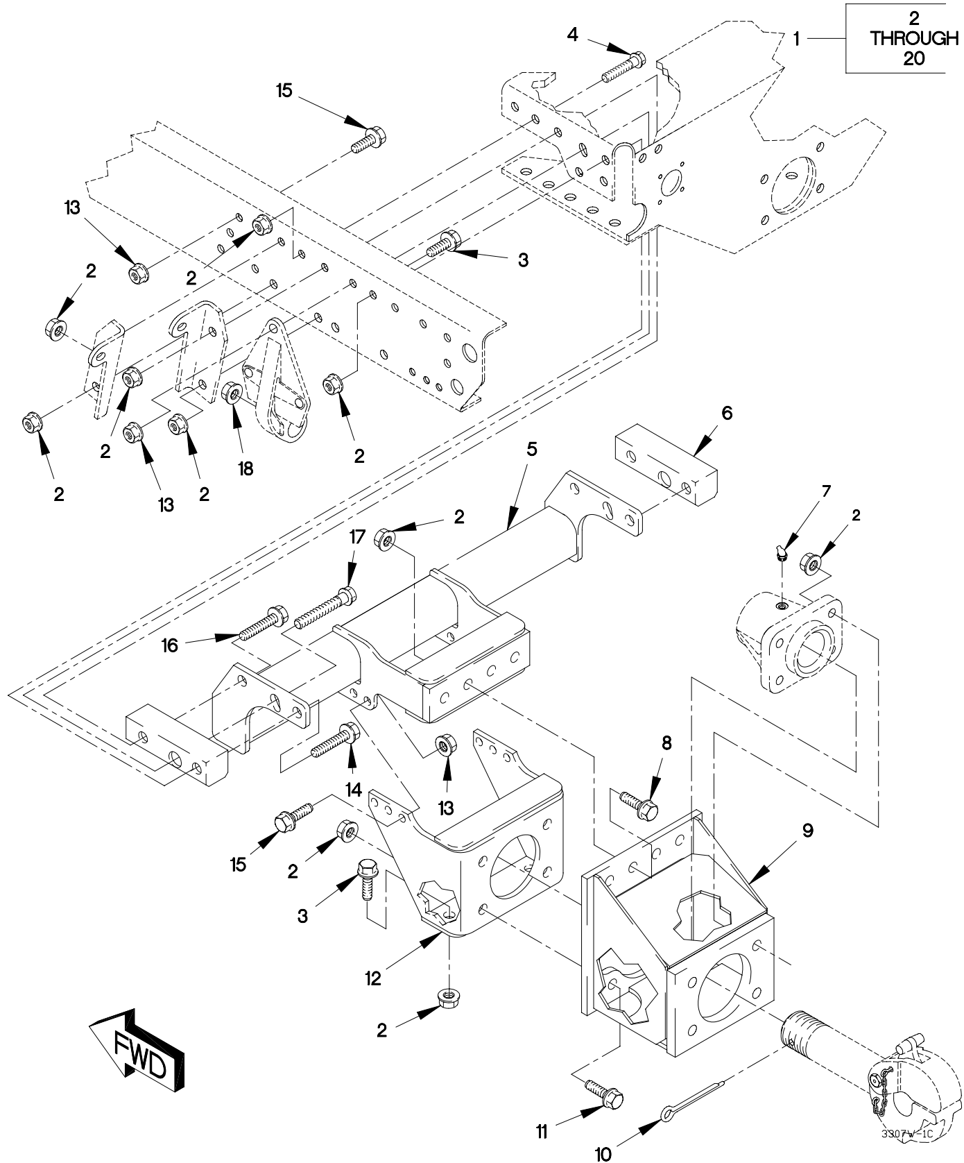
FIGURE 485. PINTLE HOOK EXTENSION KIT (SHEET 1 OF 2)
