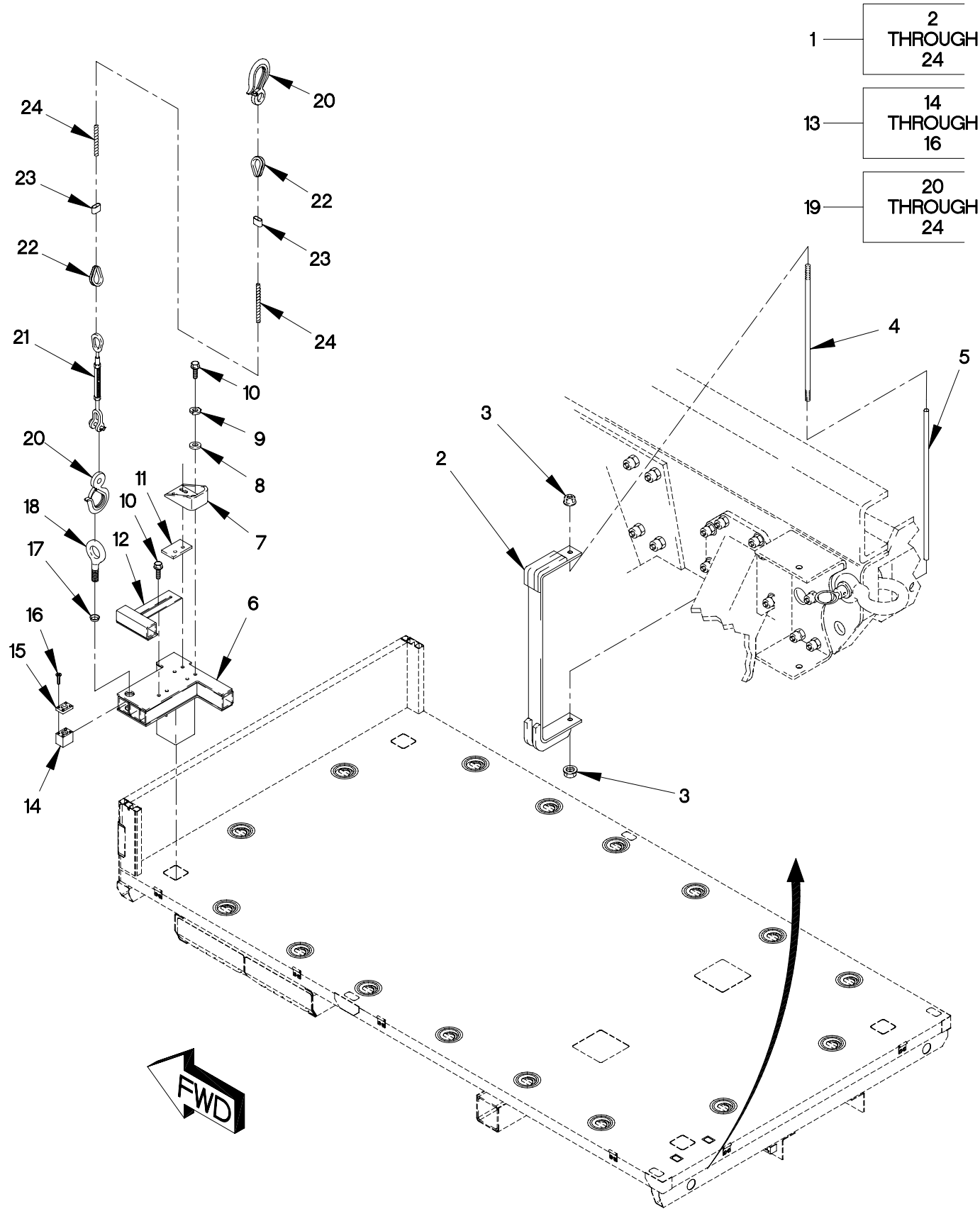
FIGURE 480. M1083 AND M1093 SHELTER TIEDOWN KIT
