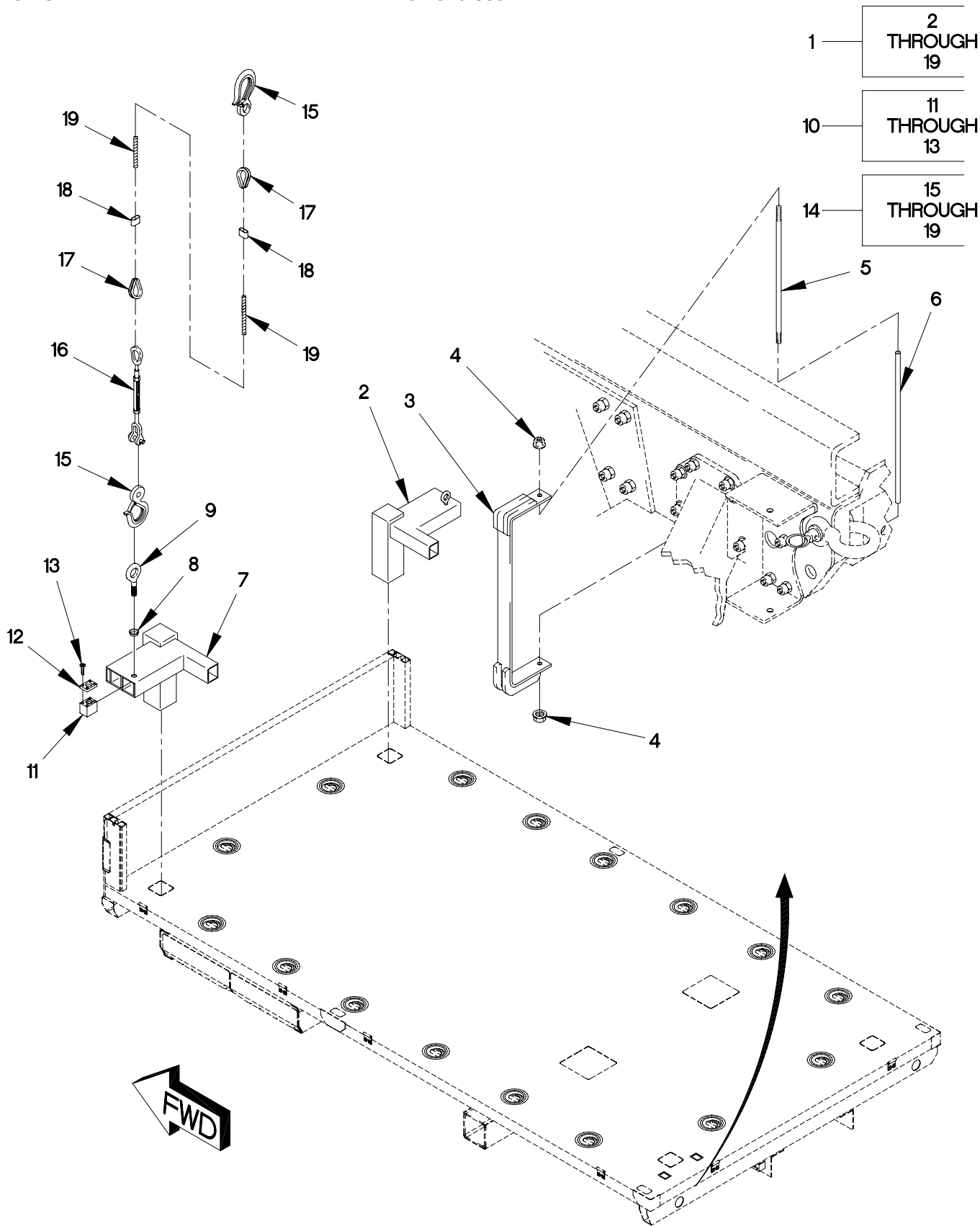
FIGURE 477. SHELTER TIE-DOWN KIT
