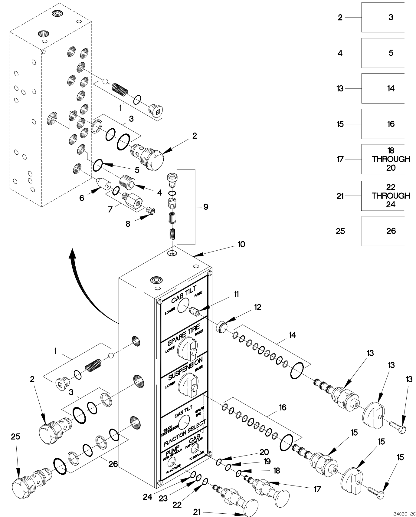
FIGURE 442. HYDRAULIC MANIFOLD ASSEMBLY
