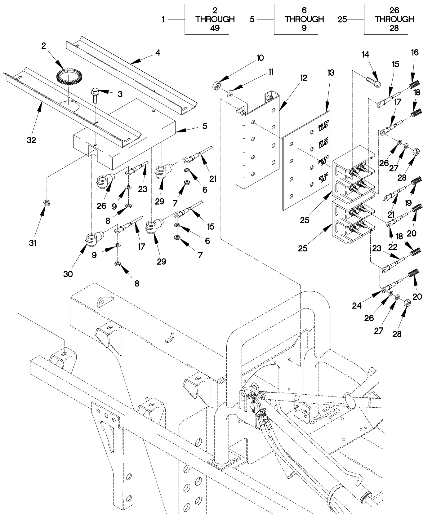
FIGURE 465. 200AMP POLARITY PROTECTION DEVICE, TERMINAL BLOCK, CABLES AND BRACKETS (SHEET 1 OF 2)
