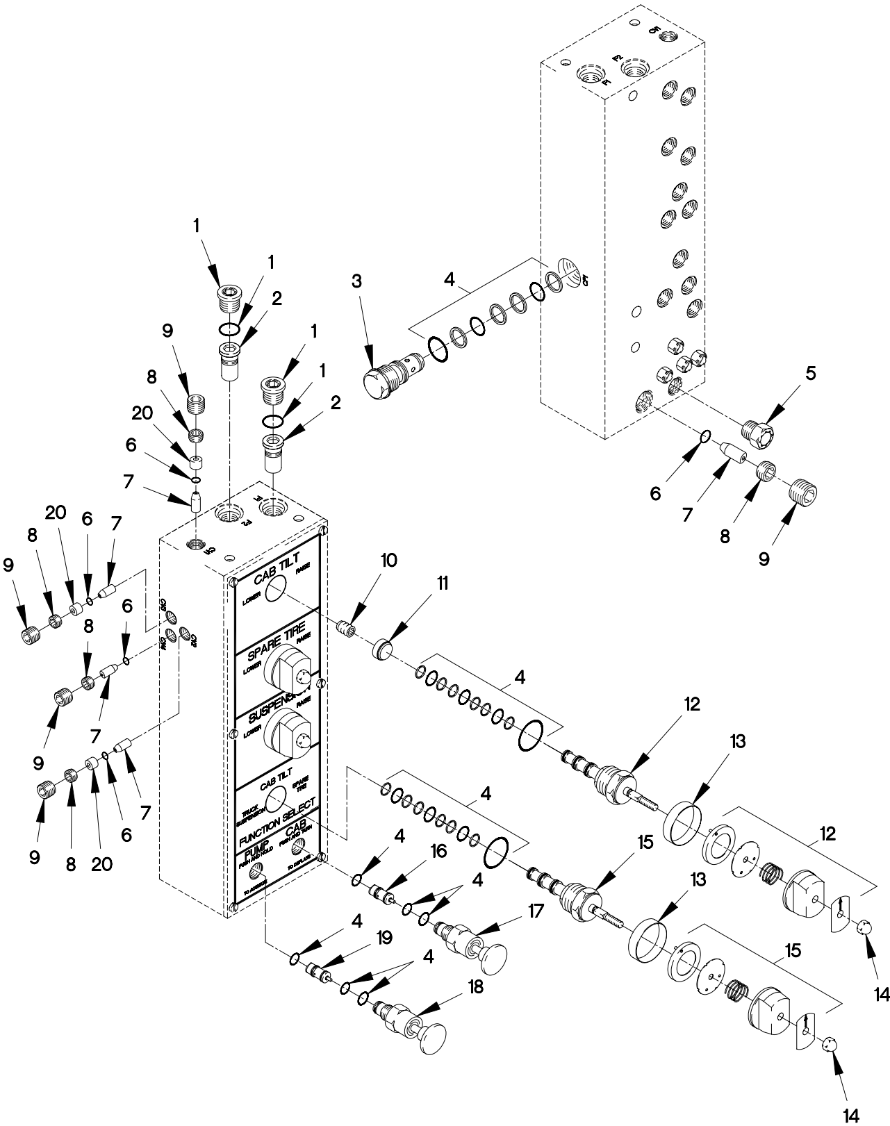
FIGURE 441. HYDRAULIC MANIFOLD ASSEMBLY
