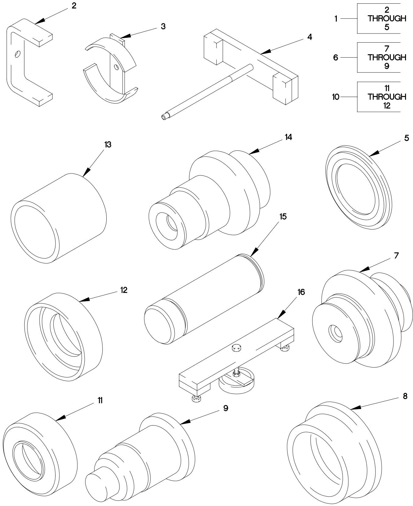
FIGURE 503. GENERAL SUPPORT MAINTENANCE SPECIAL TOOLS (SHEET 1 OF 2)
