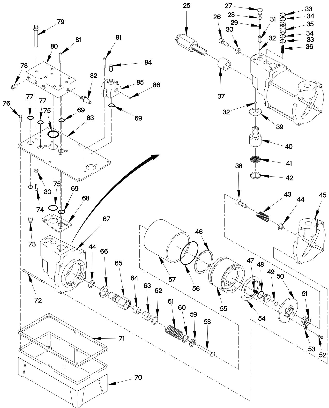
FIGURE 437. AIR/HYDRAULIC POWER UNIT, HOSES AND FITTINGS (SHEET 2 OF 2)
