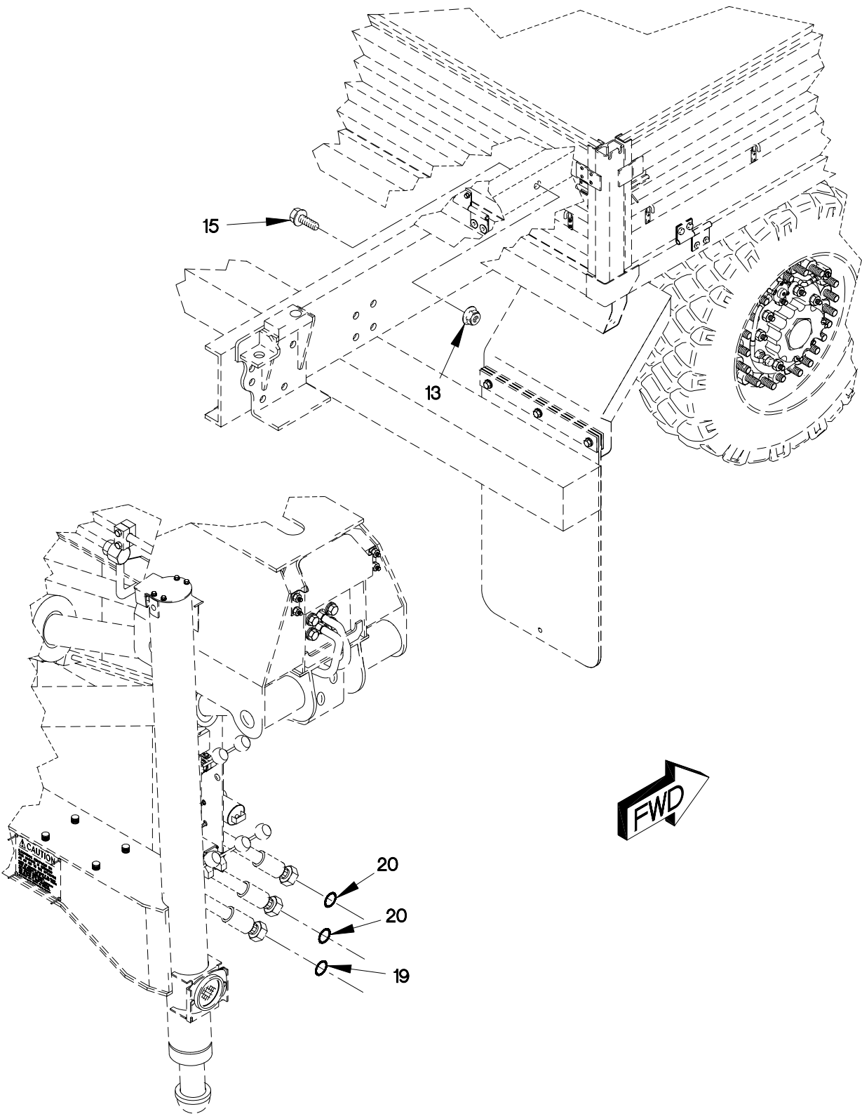
FIGURE 485. PINTLE HOOK EXTENSION KIT (SHEET 2 OF 2)
