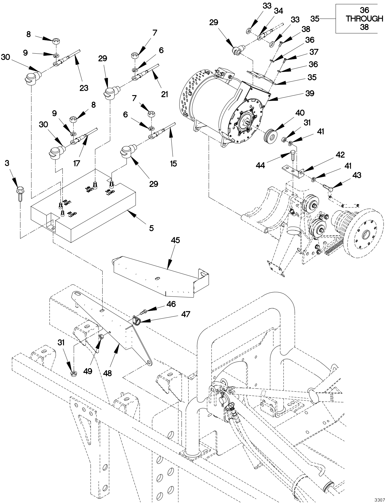
FIGURE 465. 200AMP POLARITY PROTECTION DEVICE, TERMINAL BLOCK, CABLES AND BRACKETS (SHEET 2 OF 2)
