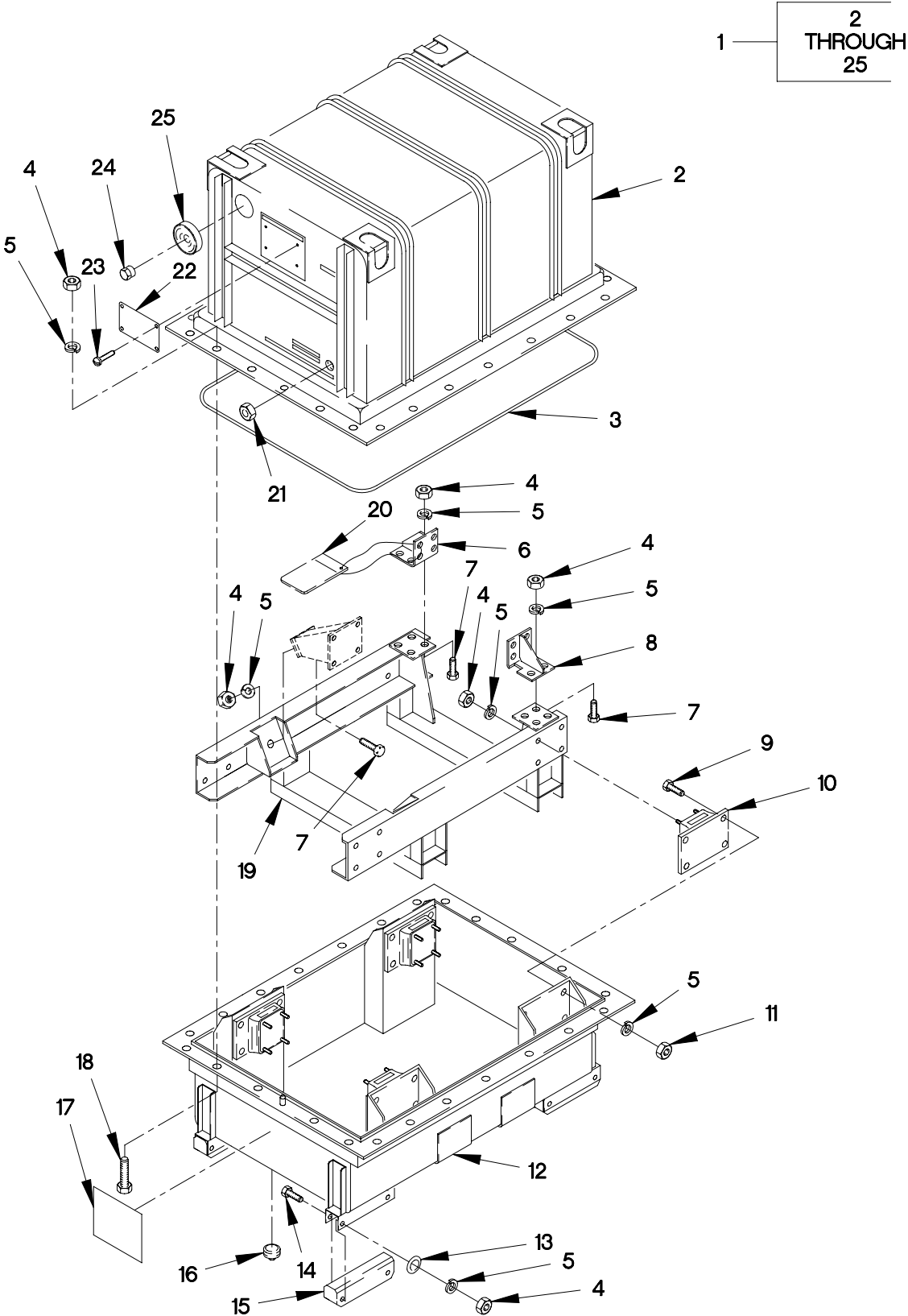
FIGURE 454. ENGINE CONTAINER
