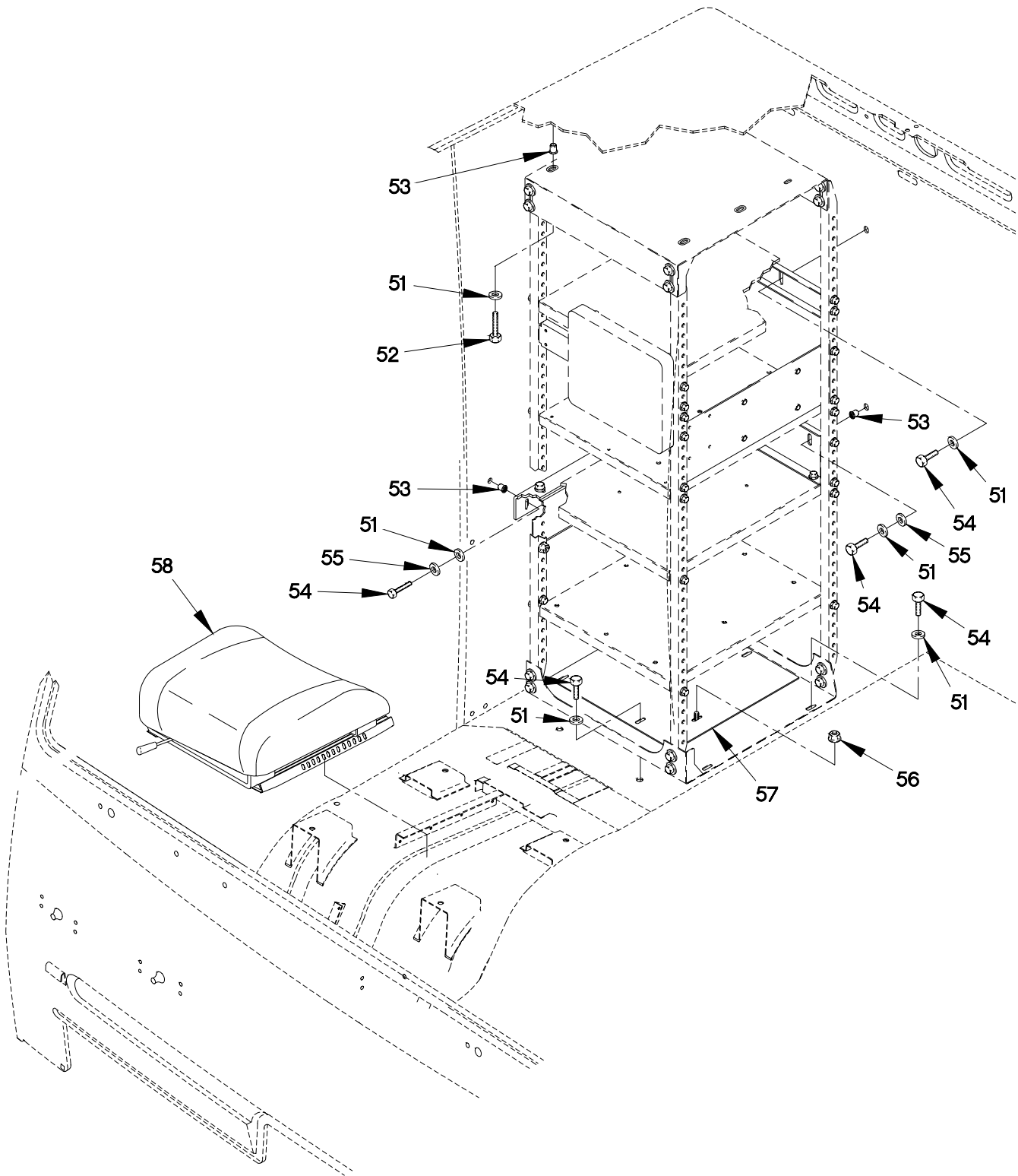
FIGURE 482. DIGITIZATION RACK/STORAGE KIT (SHEET 4 OF 5)
