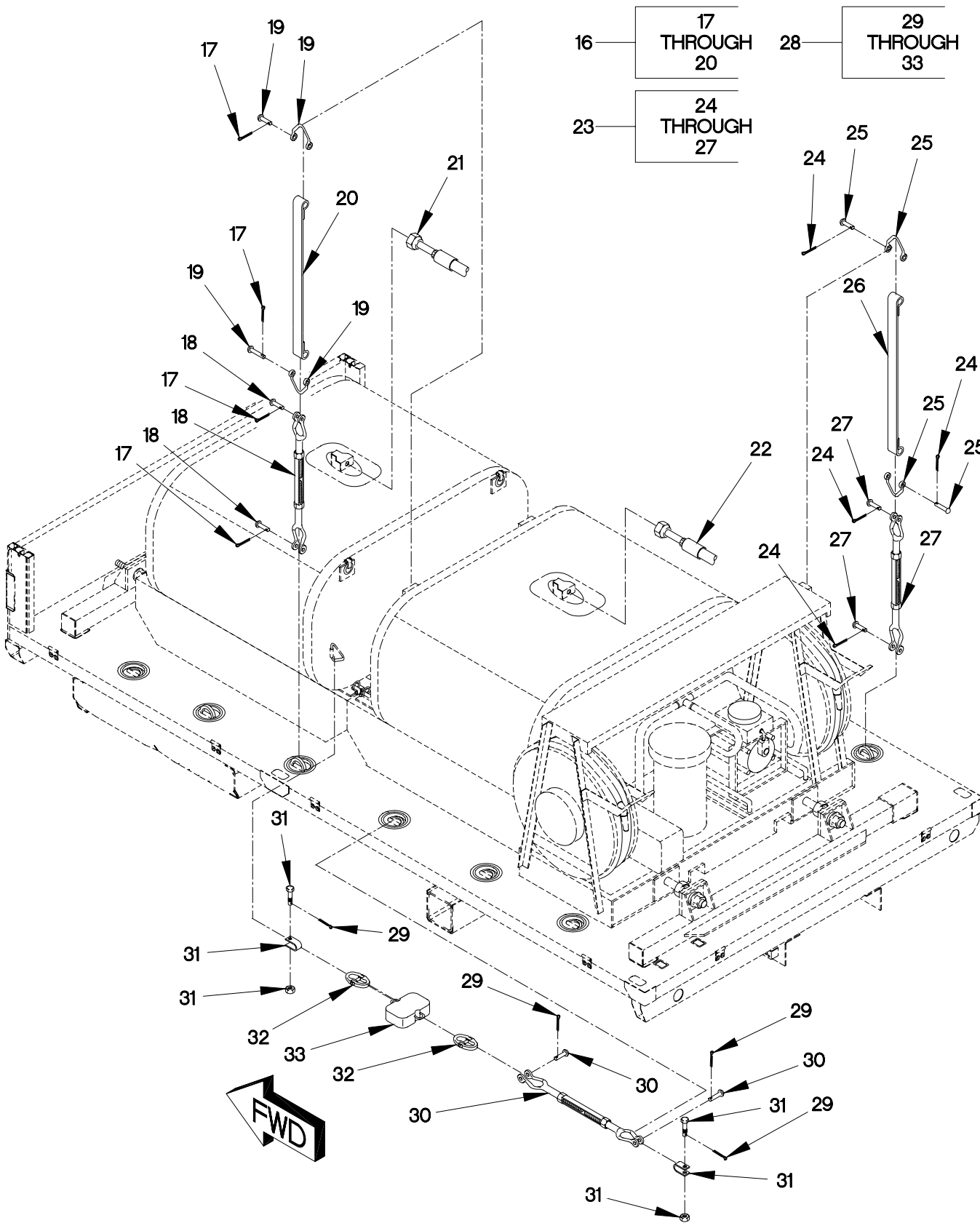
FIGURE 483. TANK AND PUMP UNIT TIEDOWN KIT (SHEET 2 OF 2)
