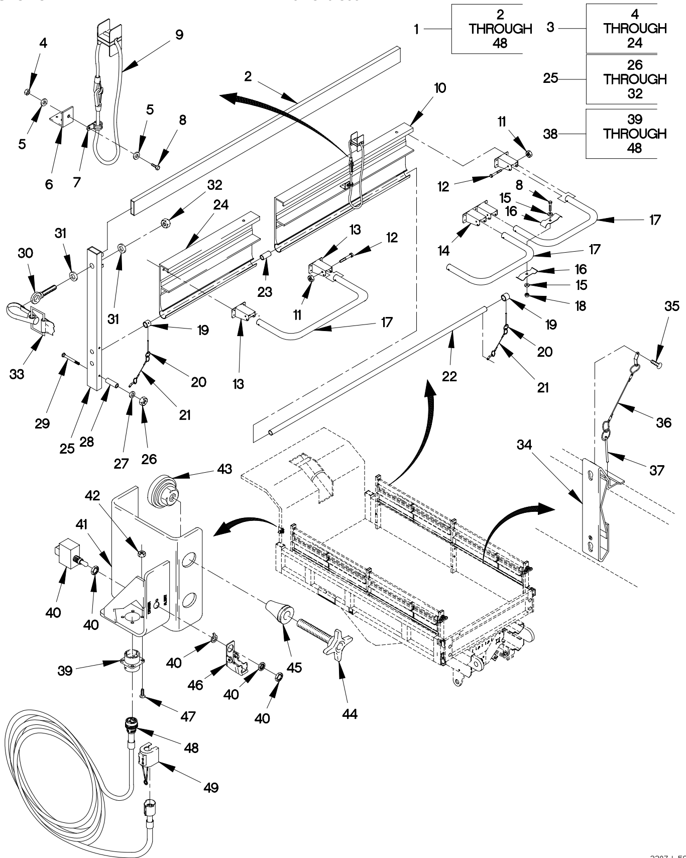
FIGURE 461. M1090 AND M1094 TROOPSEAT KIT
