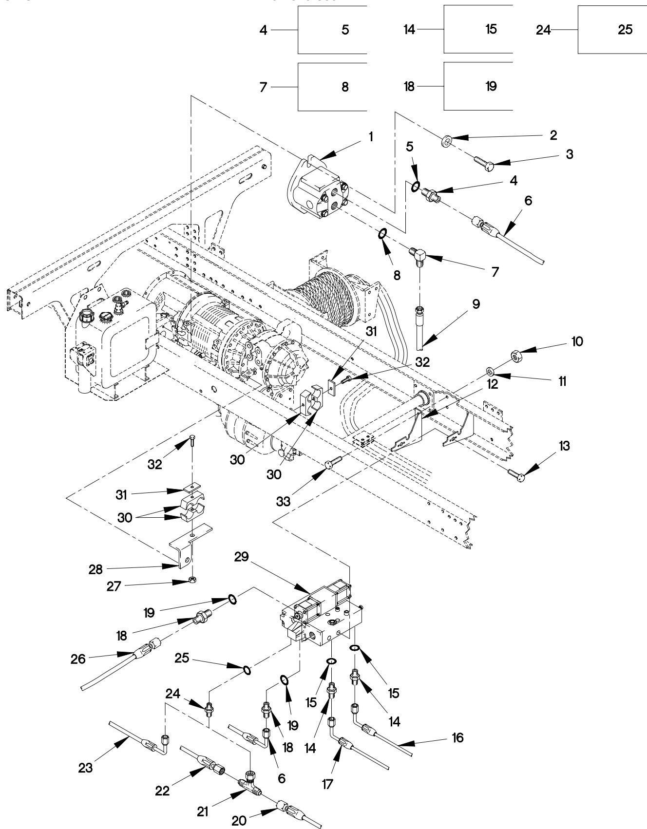
FIGURE 446. HYDRAULIC ROTARY PUMP, WINCH CONTROL VALVE, HOSES AND FITTINGS (SHEET 1 OF 3)
