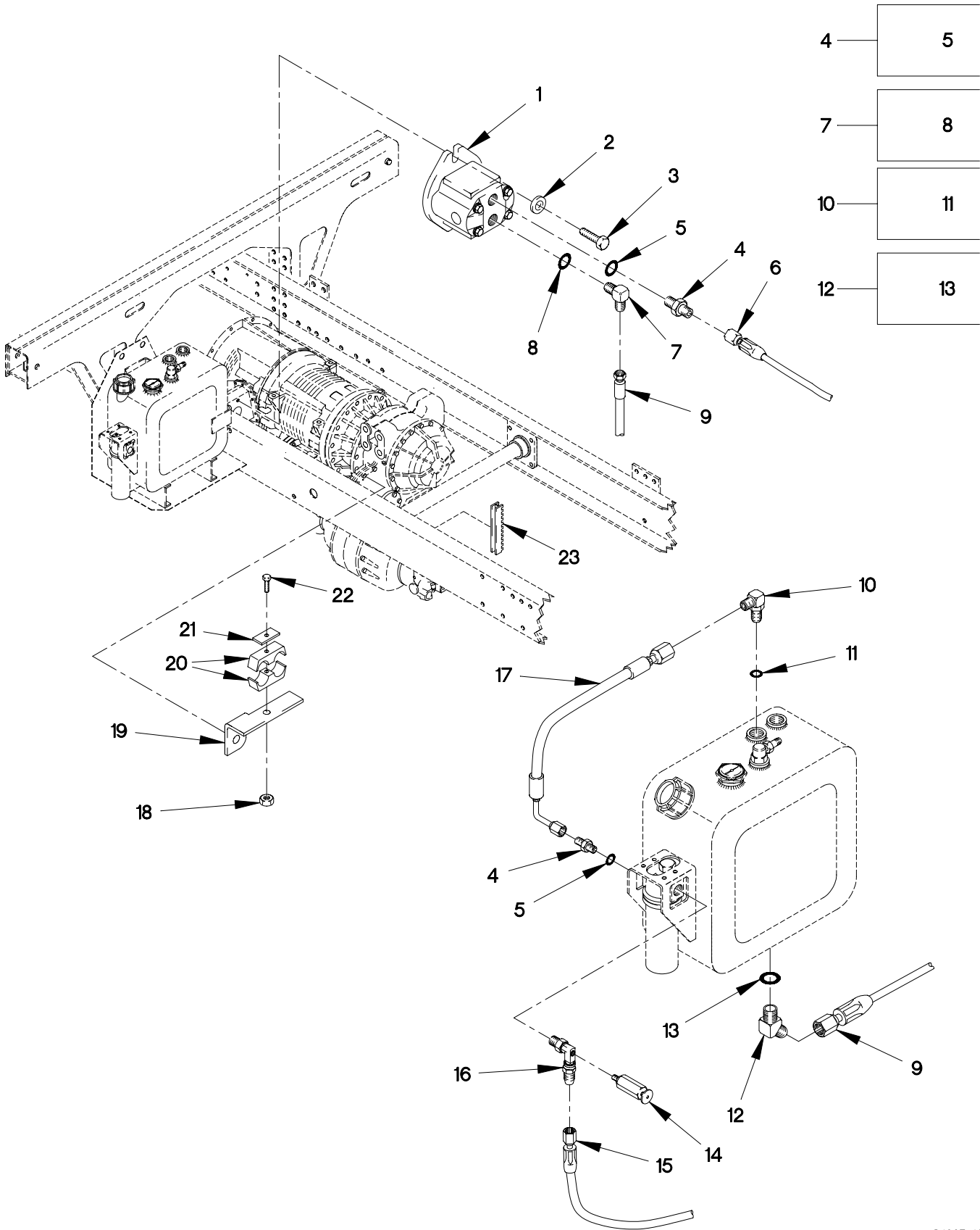
FIGURE 449. M1090 AND M1094 HYDRAULIC ROTARY PUMP, HOSES AND FITTINGS (SHEET 1 OF 3)
