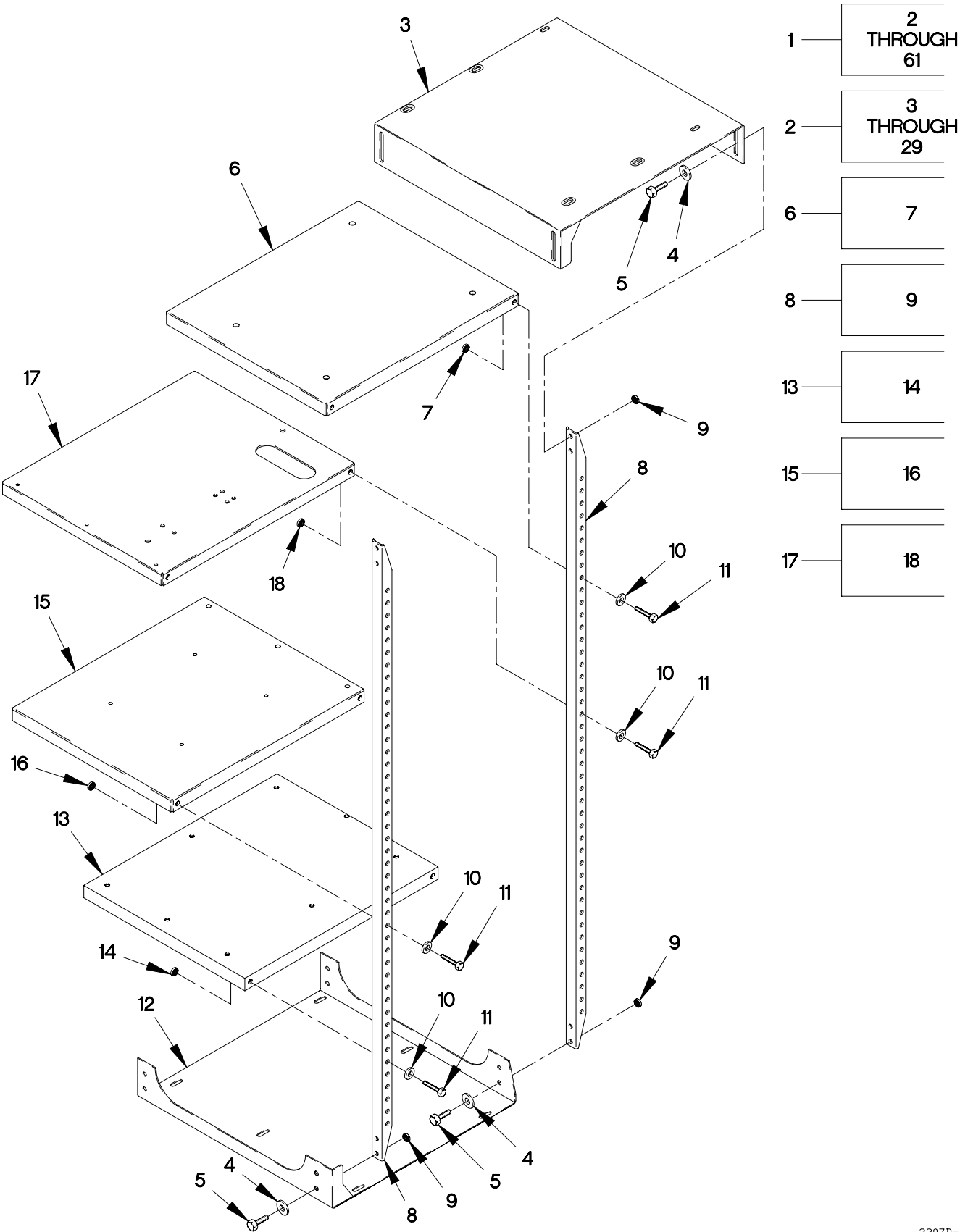
FIGURE 482. DIGITIZATION RACK/STORAGE KIT (SHEET 1 OF 5)
