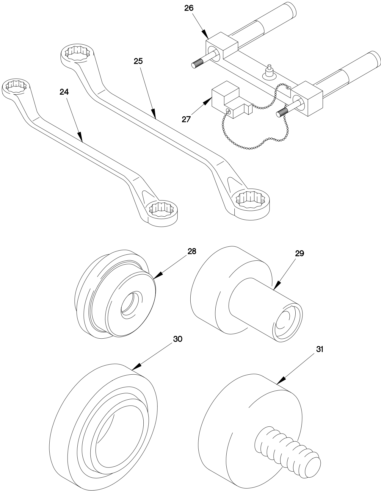
FIGURE 502. DIRECT SUPPORT MAINTENANCE SPECIAL TOOLS (SHEET 3 OF 3)
