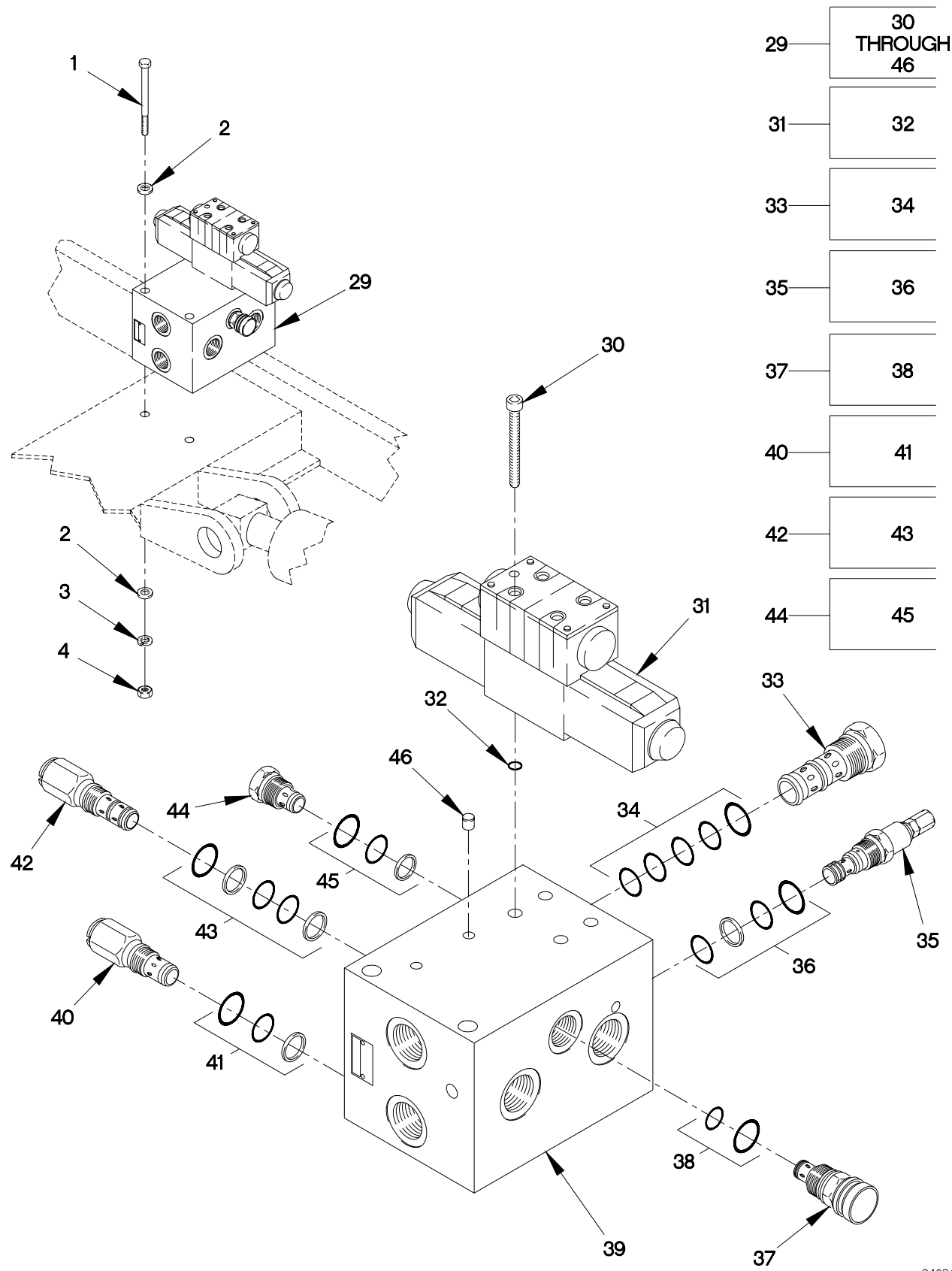
FIGURE 439. FOUR WAY RELIEF VALVE (SHEET 2 OF 2)
