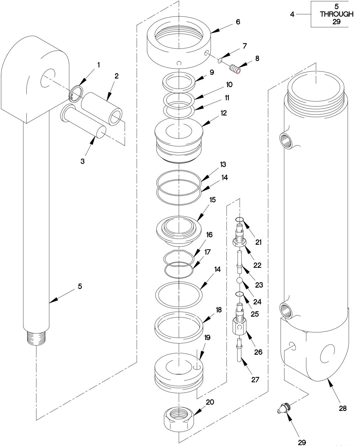
FIGURE 445. M1090 AND M1094 DUMP BODY LIFT CYLINDER
