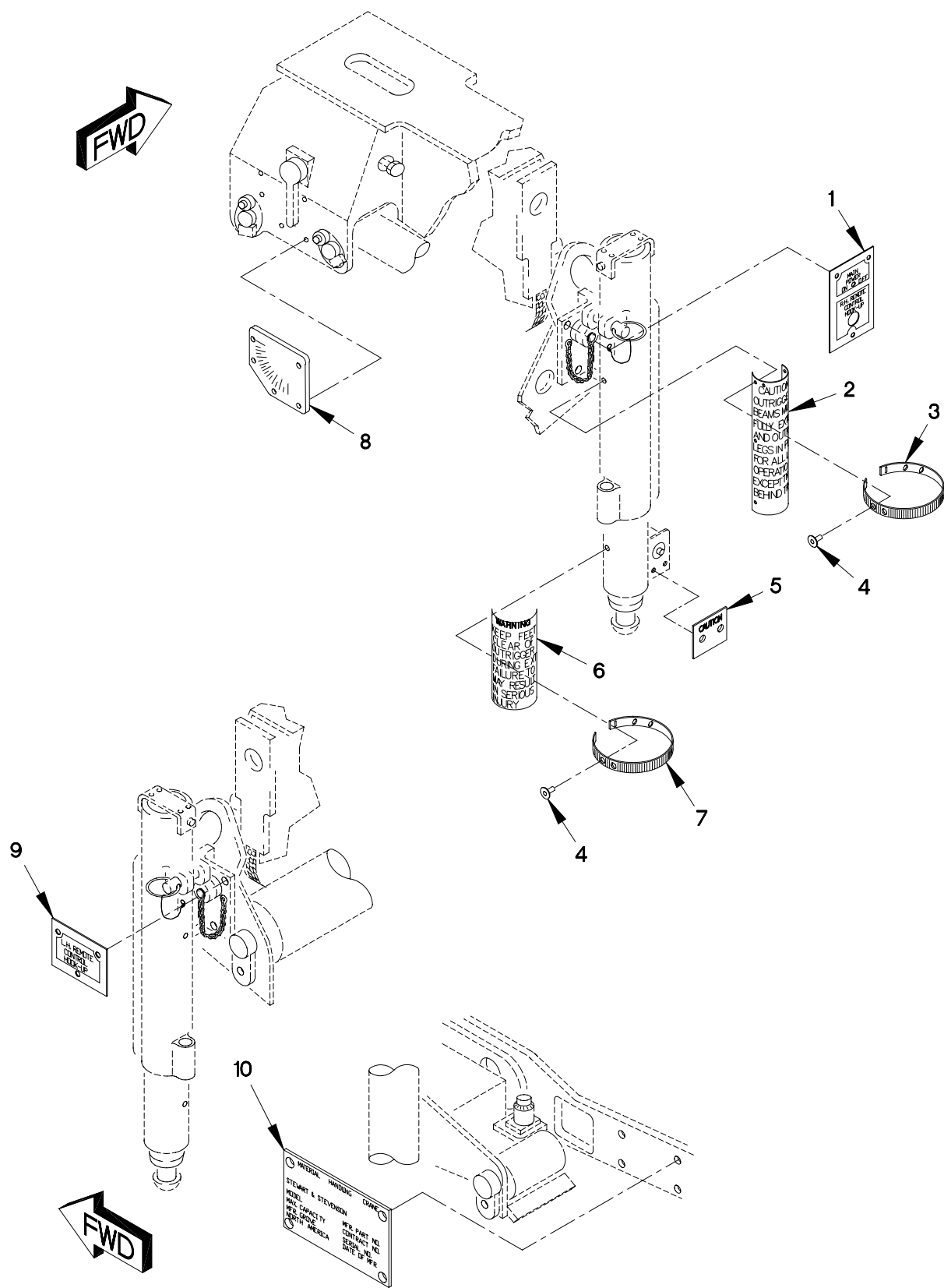
FIGURE 435. M1089 DECALS AND DATA PLATES (SHEET 1 OF 2)
