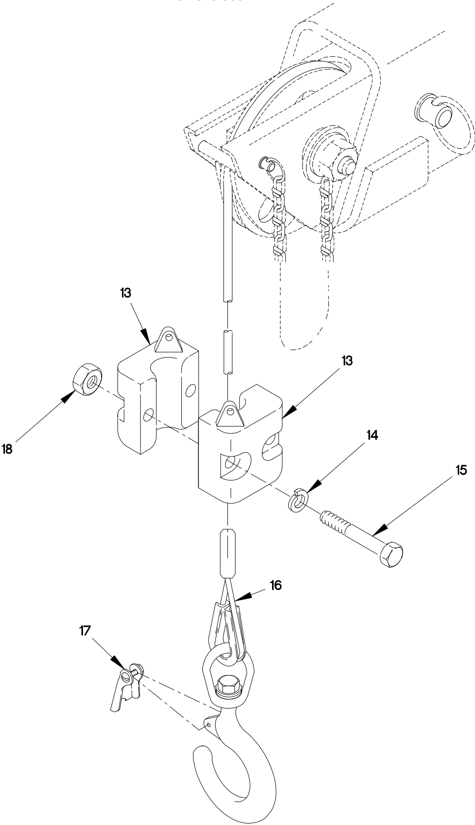
FIGURE 468. LIGHT MATERIAL HANDLING CRANE KIT (SHEET 2 OF 2)
