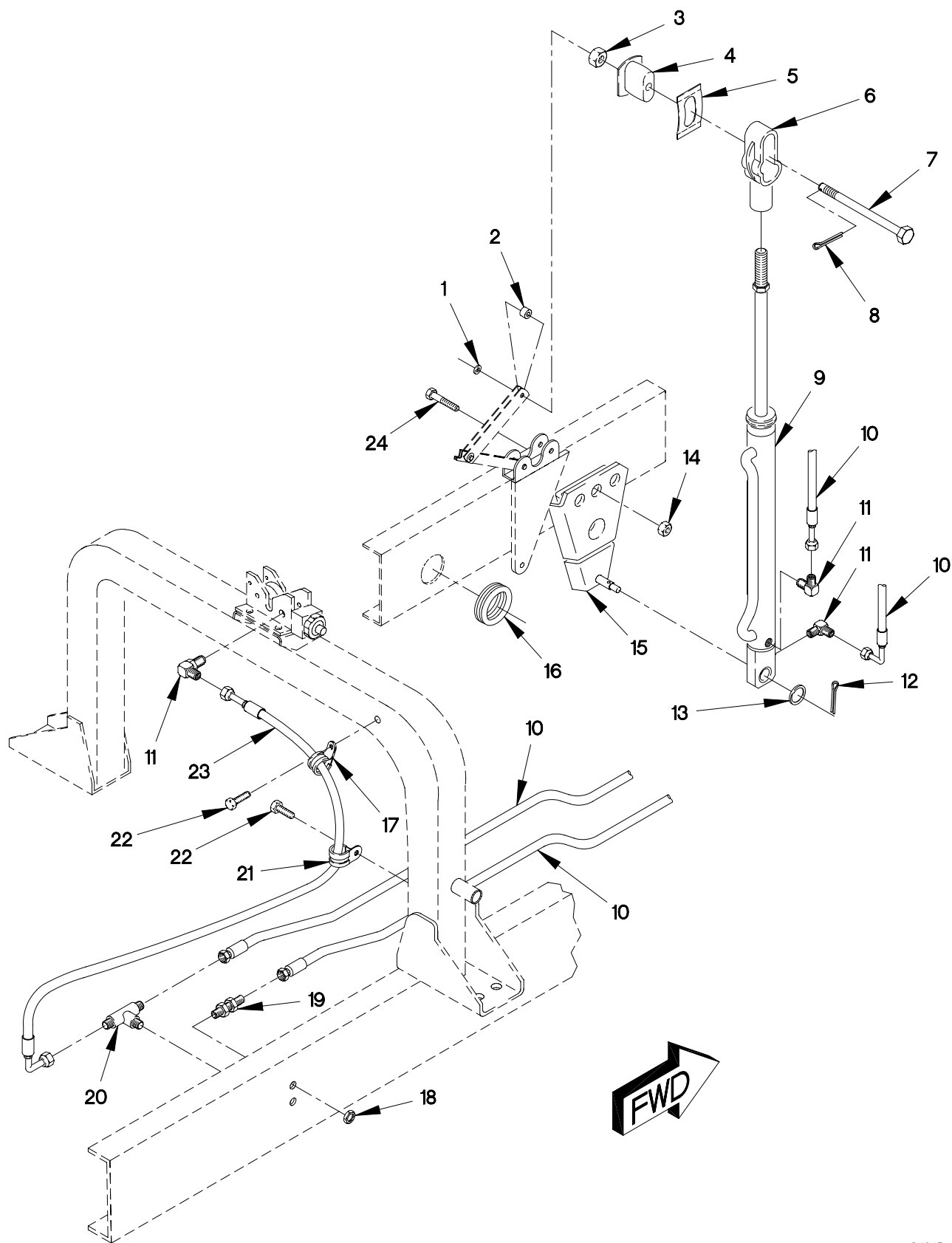
FIGURE 444. CAB HYDRAULIC CYLINDER, HOSES AND FITTINGS
