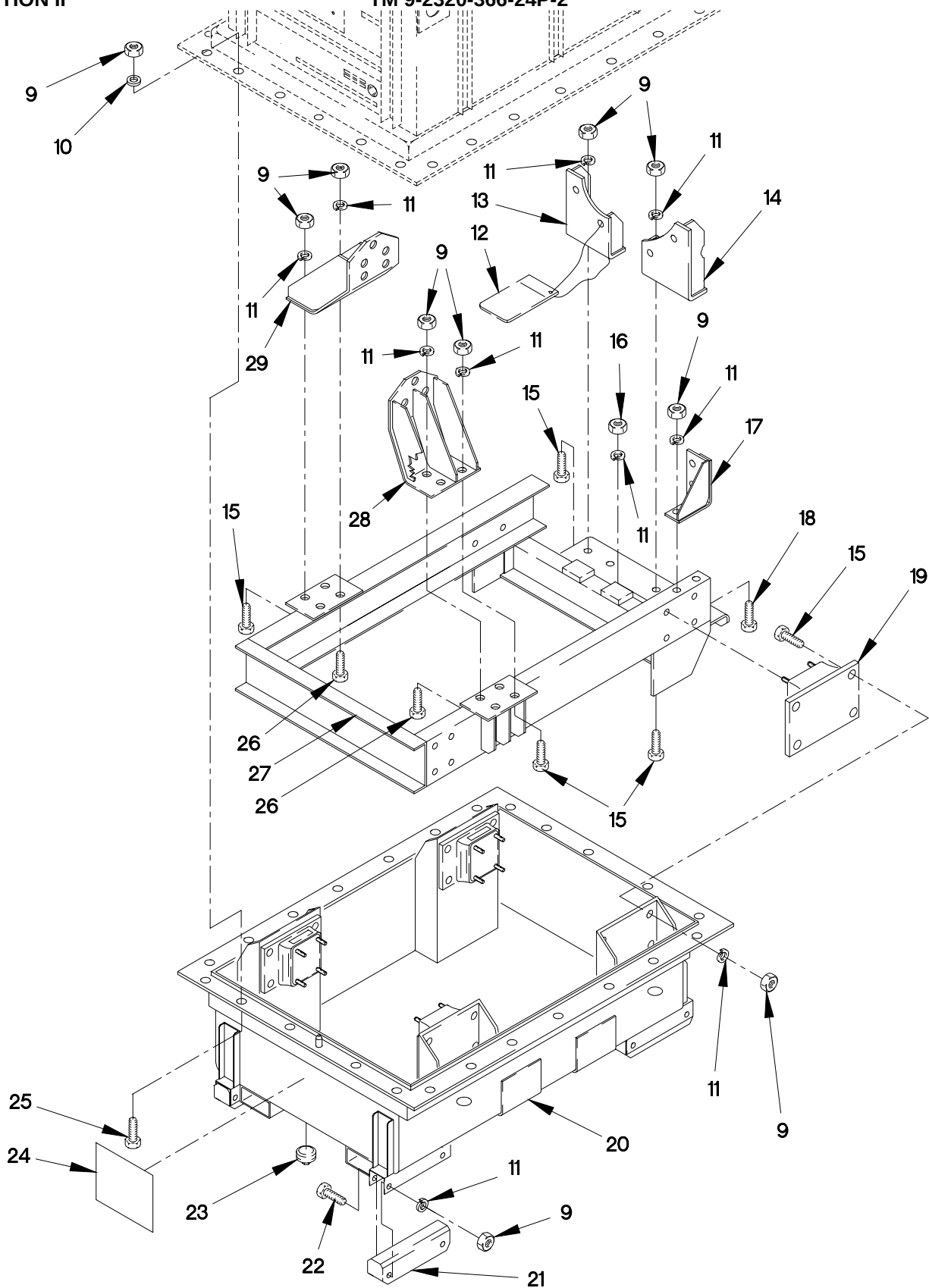
FIGURE 455. TRANSMISSION CONTAINER (SHEET 2 OF 2)
