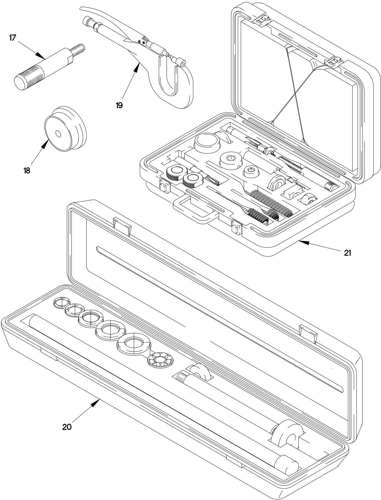
FIGURE 503. GENERAL SUPPORT MAINTENANCE SPECIAL TOOLS (SHEET 2 OF 2)
