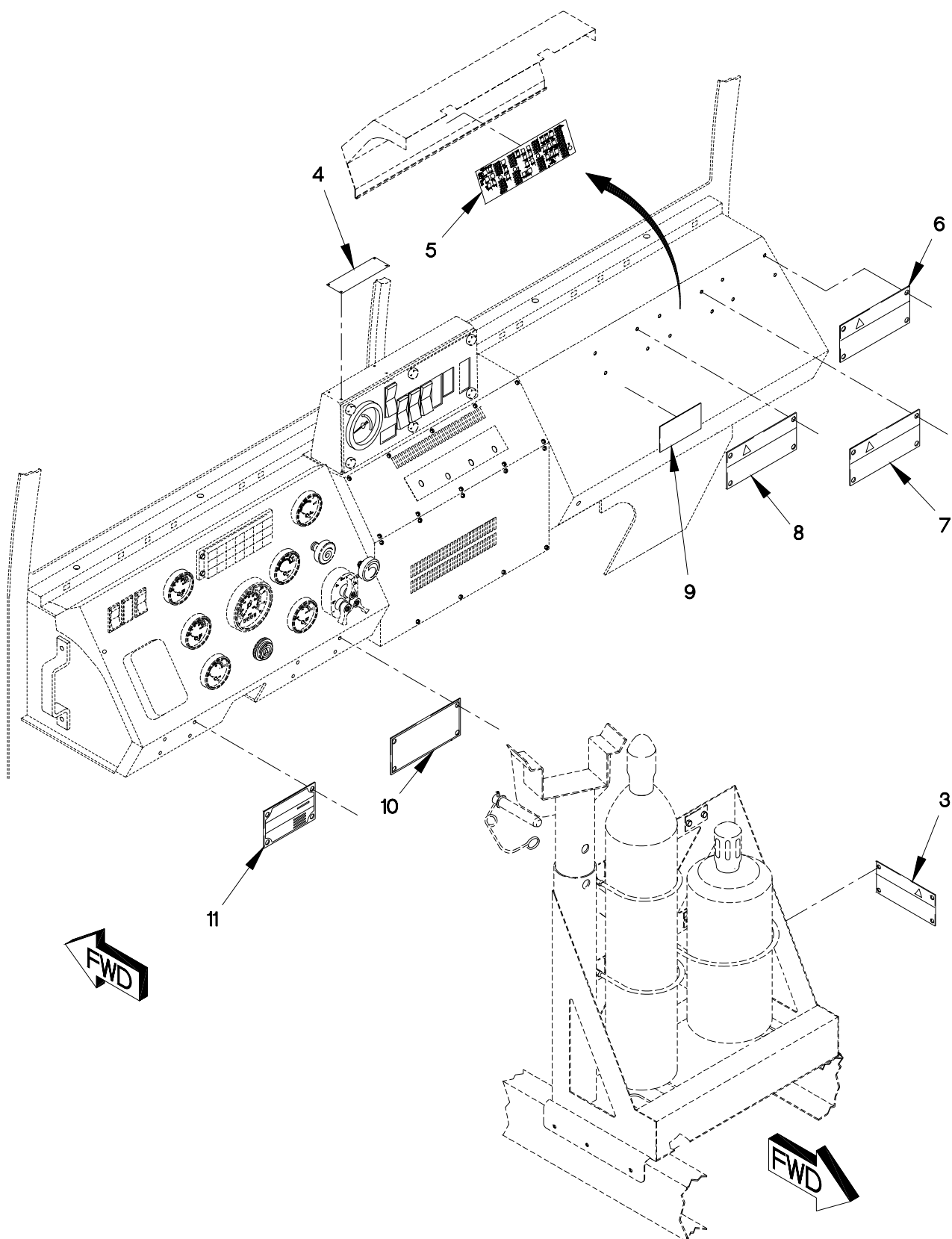
FIGURE 434. DATA AND IDENTIFICATION PLATES (SHEET 2 OF 6)
