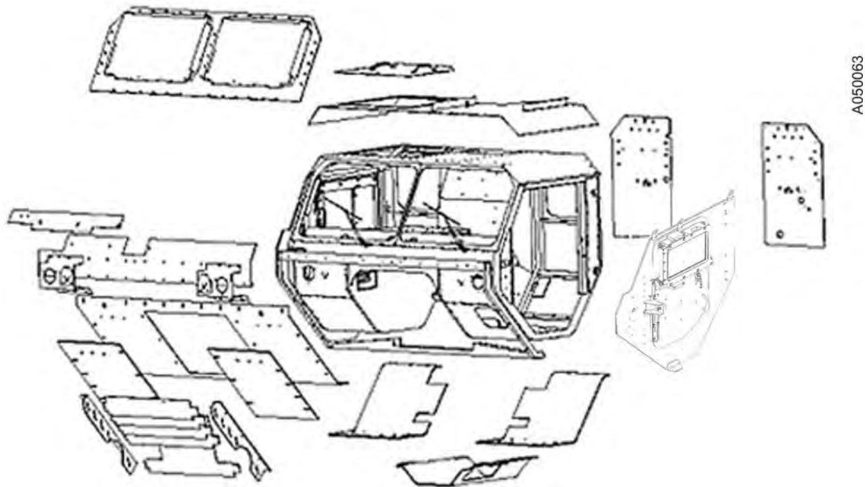
Figure 1. HEMTT Crew Protection Armor Kit component location.
