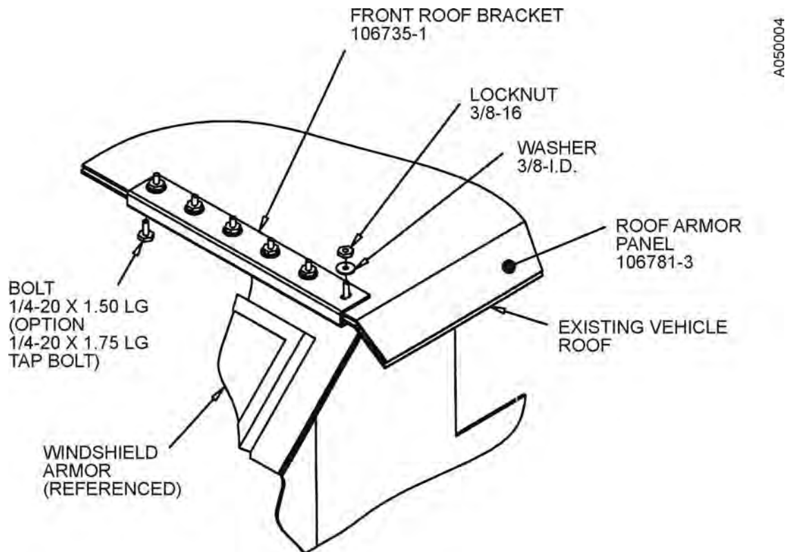
Figure 43. Secure the forward end of the Roof Armor Panel using the attachment hardware.
