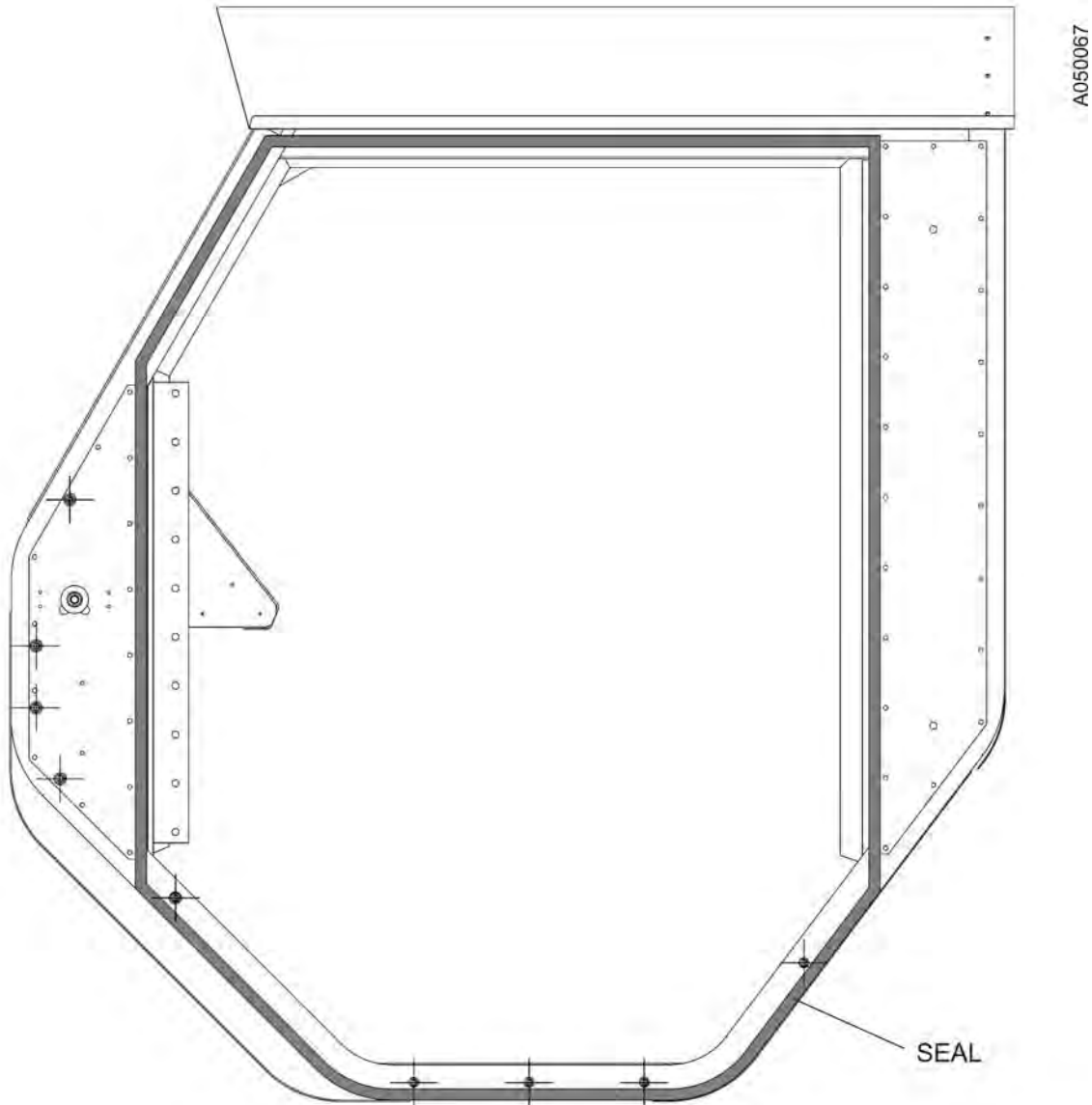
Figure 36. Side Armor Panel Side Seal Gasket attachment.
