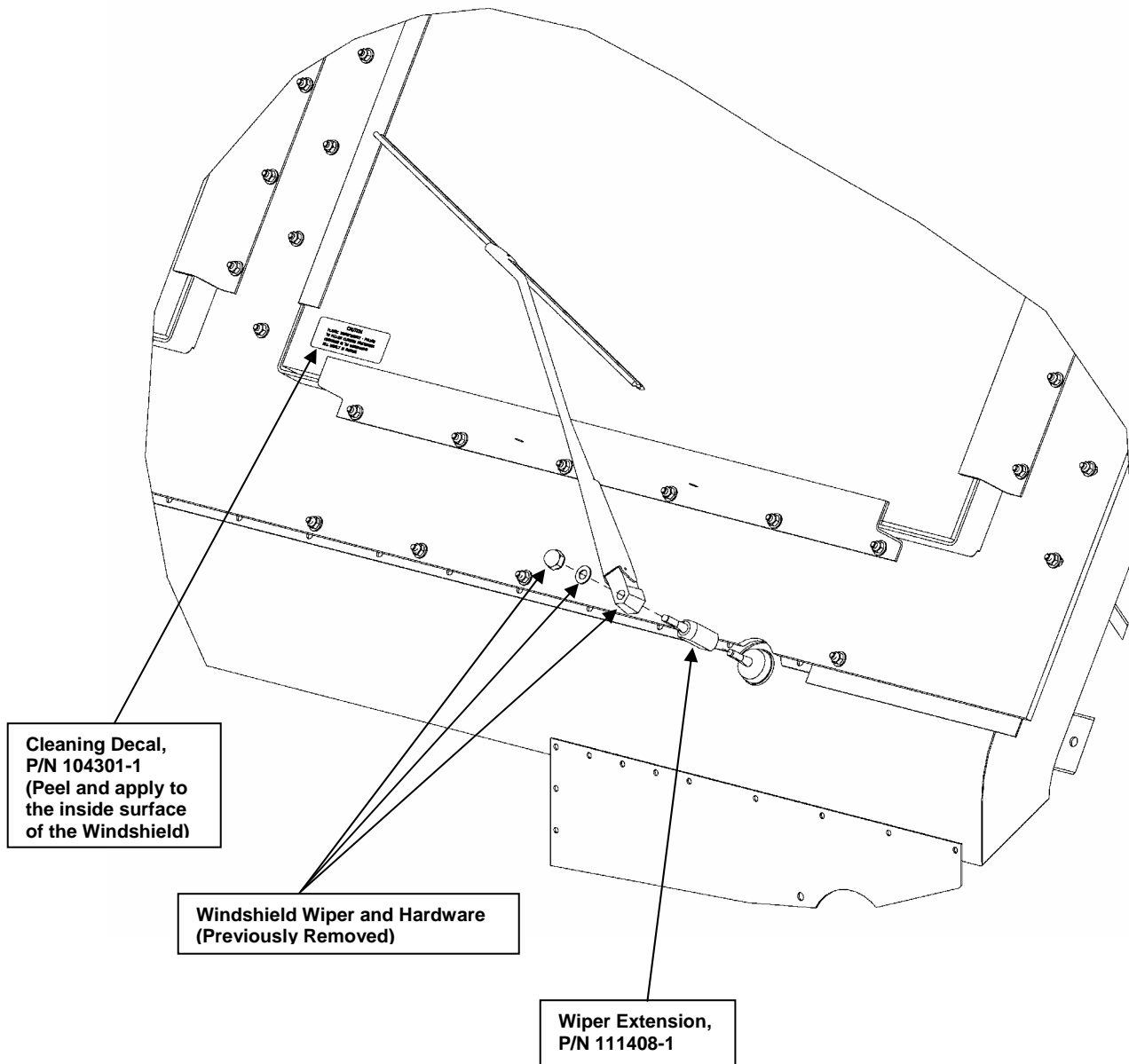
Figure 22. Windshield Wiper and Cleaning Decal installation.
