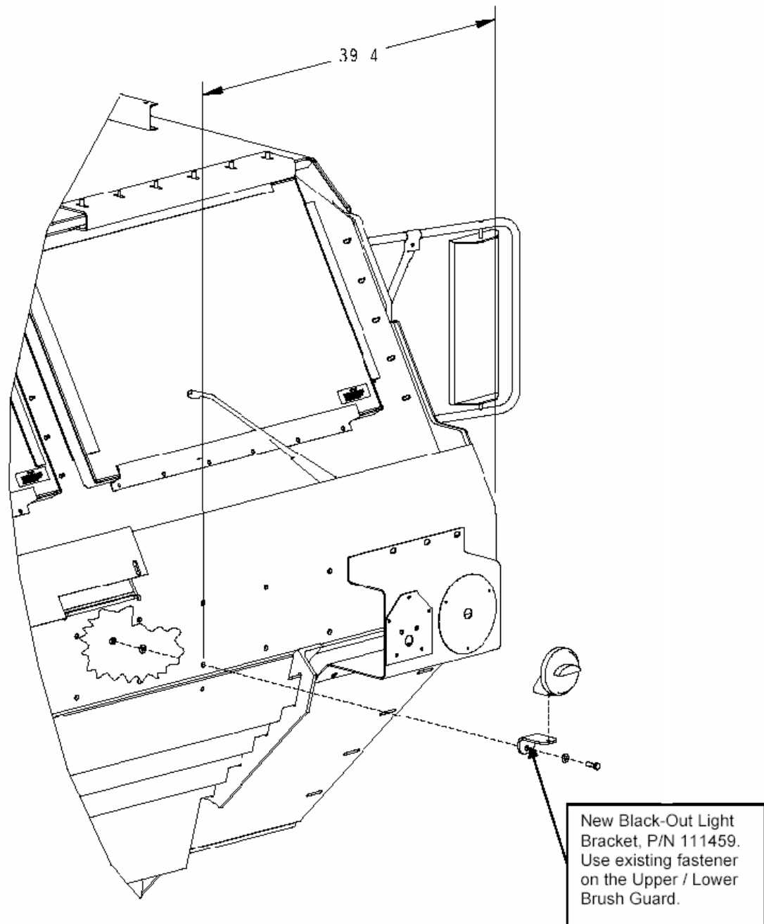
Figure 46. Blackout Light installation.
