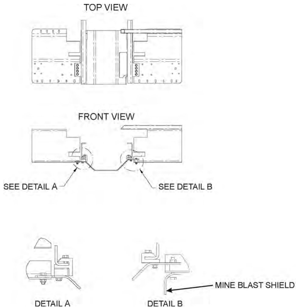
Figure 29. Blast Deflector installation (2 of 2).
