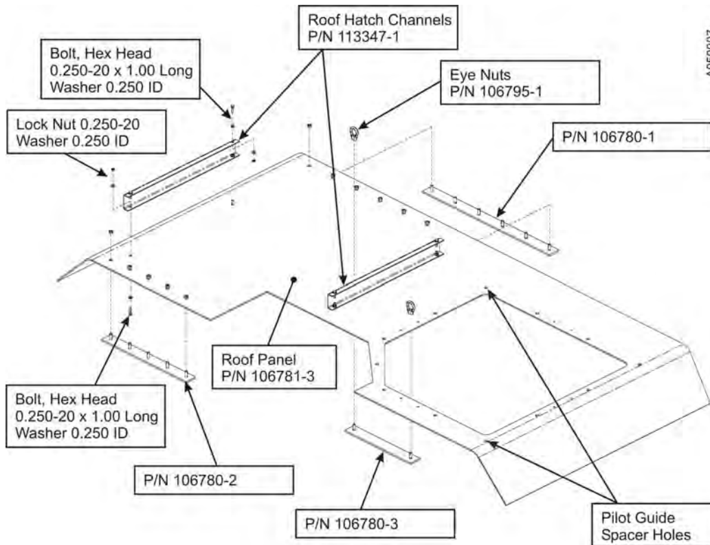
Figure 40a. Roof Armor Assembly hardware installation.
