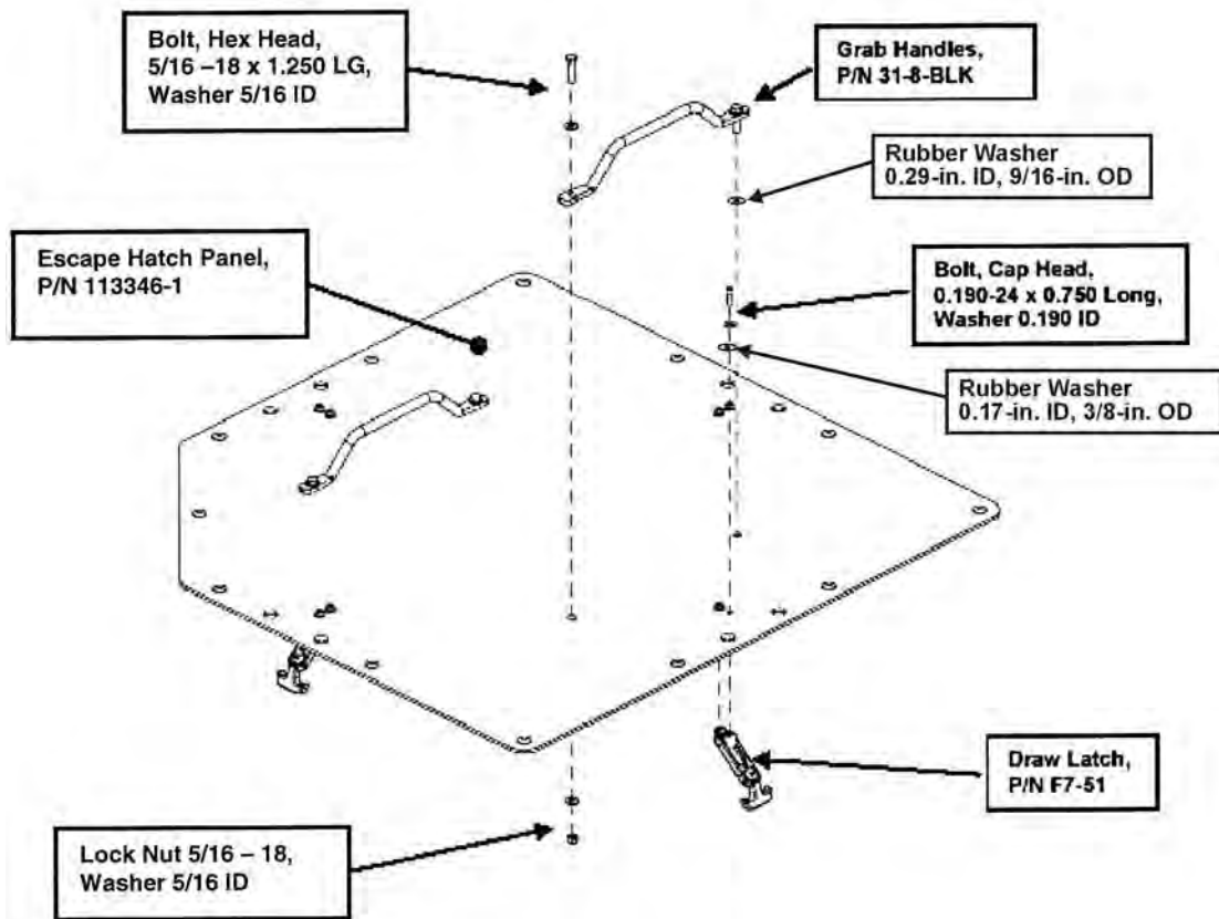
Figure 44. Escape Hatch Handle and Draw Latch illustration.
