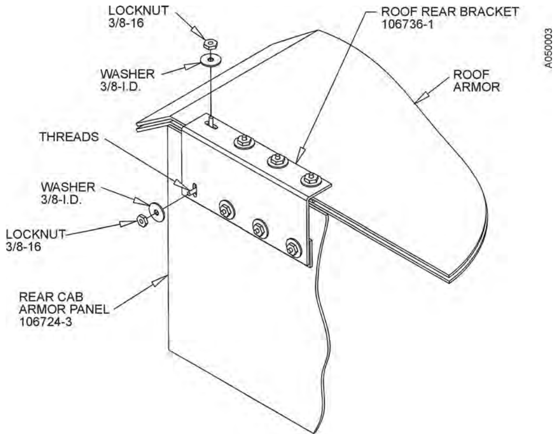
Figure 42. Position the Roof Armor Panel Rear Bracket.
