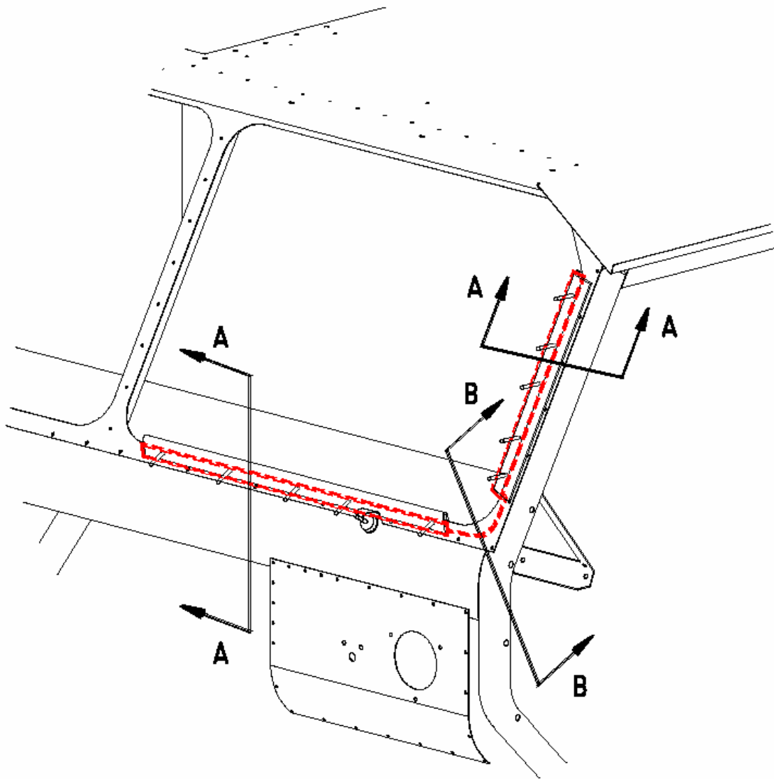
Figure 19. Urethane Sealant and Ribbon Sealer vehicle locations.
