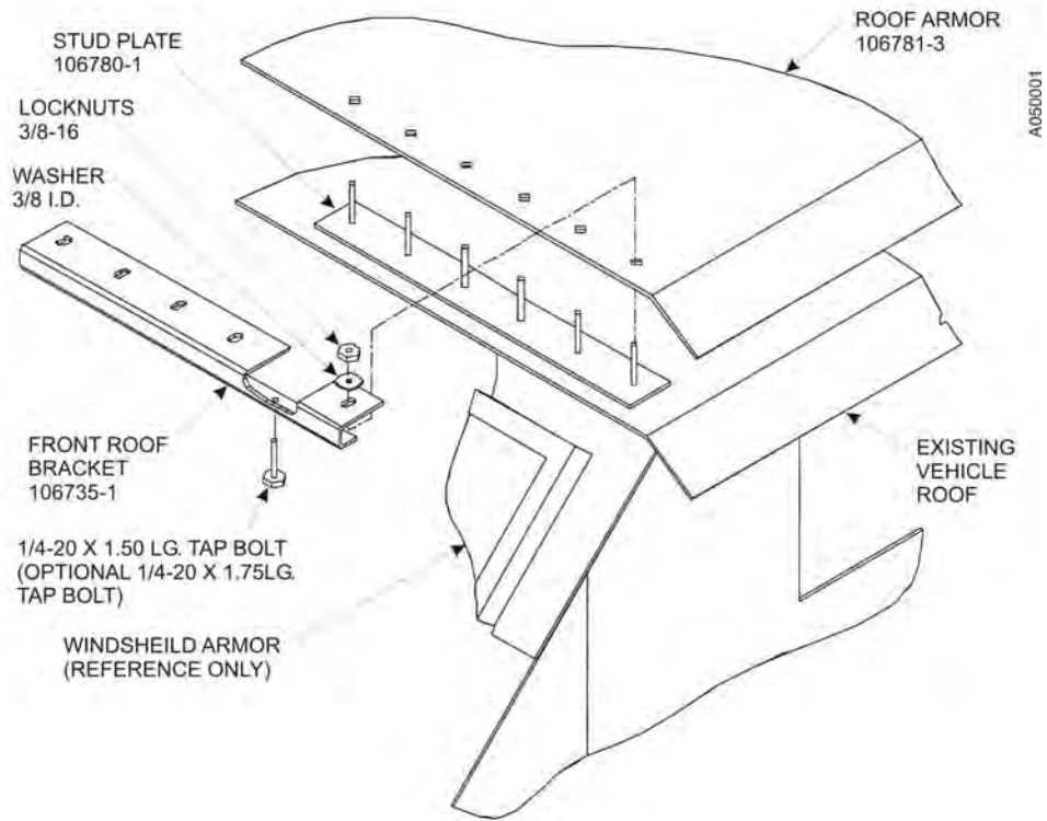
Figure 38. Roof Armor - front driver's-side installation.
