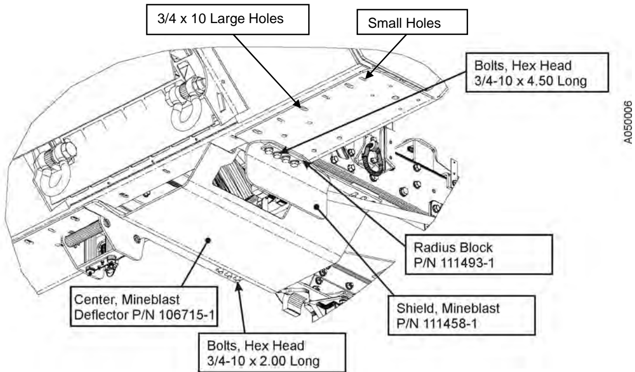
Figure 32. Secure the Center Blast Deflector to the Mounting Bracket.
