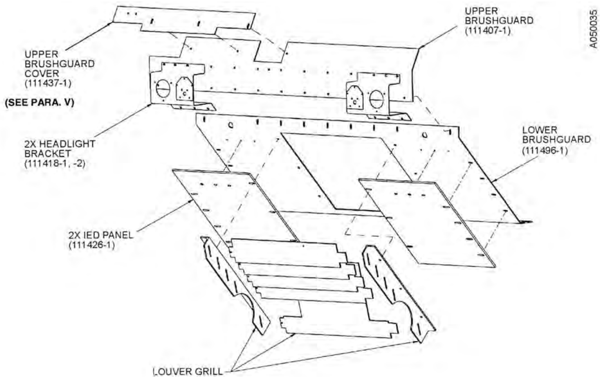
Figure 24. Front HEMTT Armor Kit locations.
