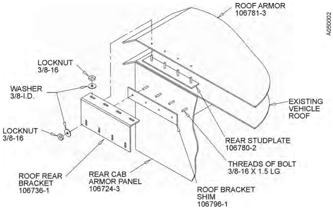
Figure 39. Roof Armor - rear driver's-side installation.
