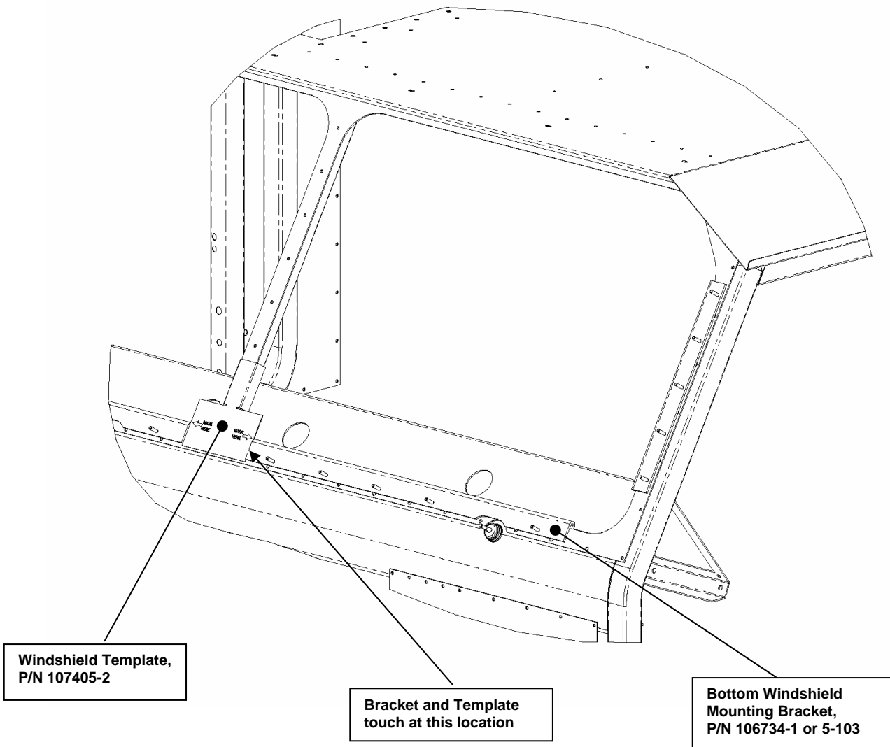
Figure 16. Windshield Bracket, Bottom Mounting.
