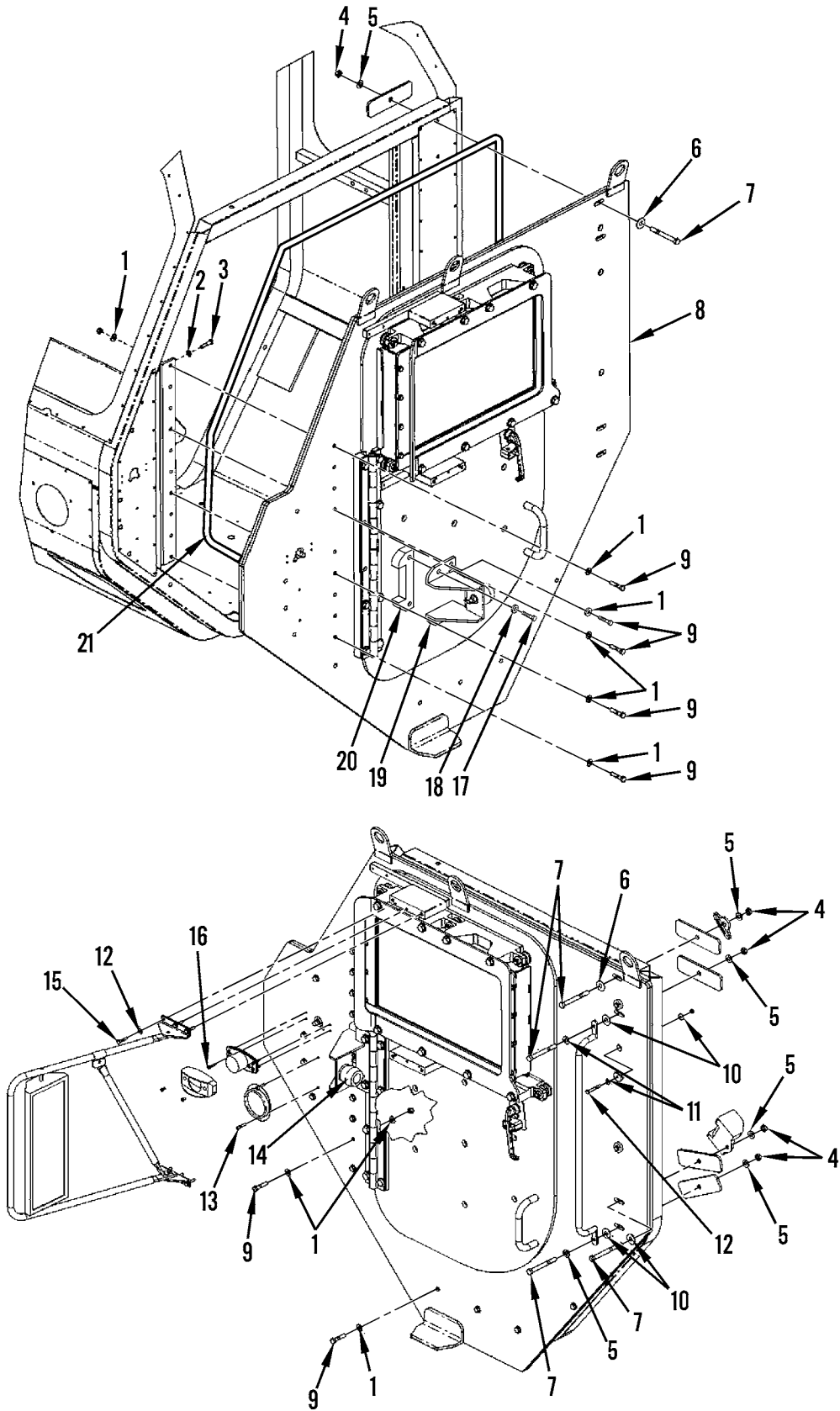
Figure 5A. Armor Door Assembly, Left and Right Side - Model B
