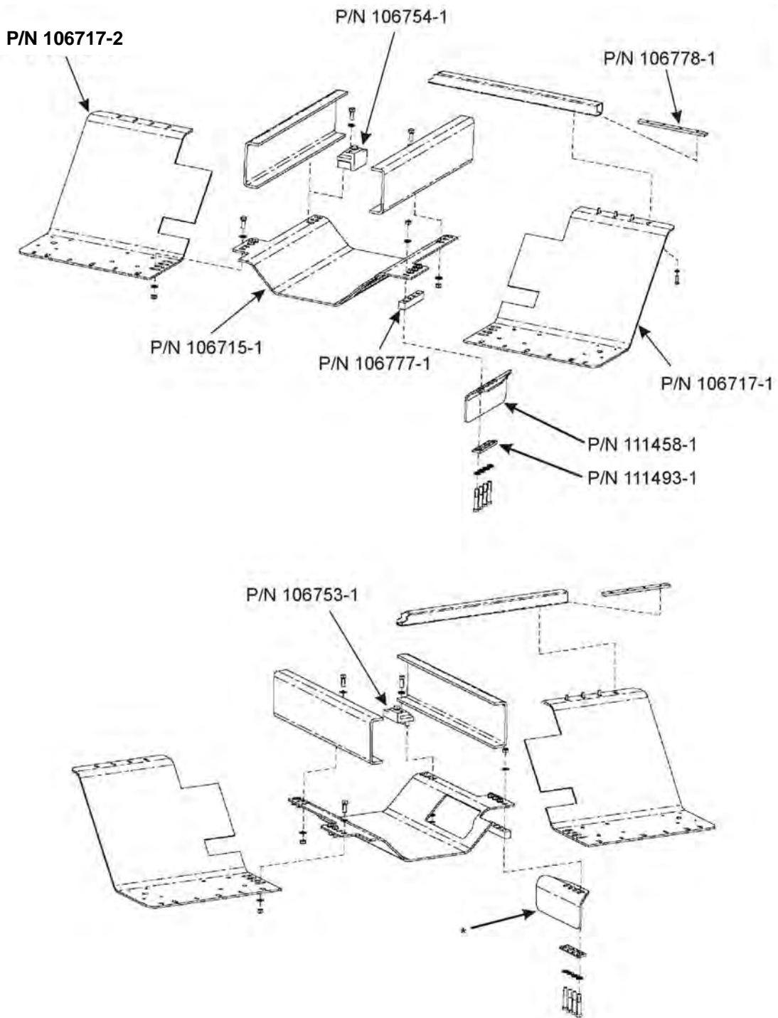
Figure 29. Blast Deflector installation (1 of 2).
