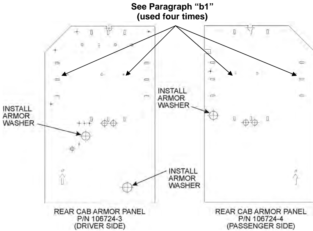
Figure 26a. Armored washer locations.
