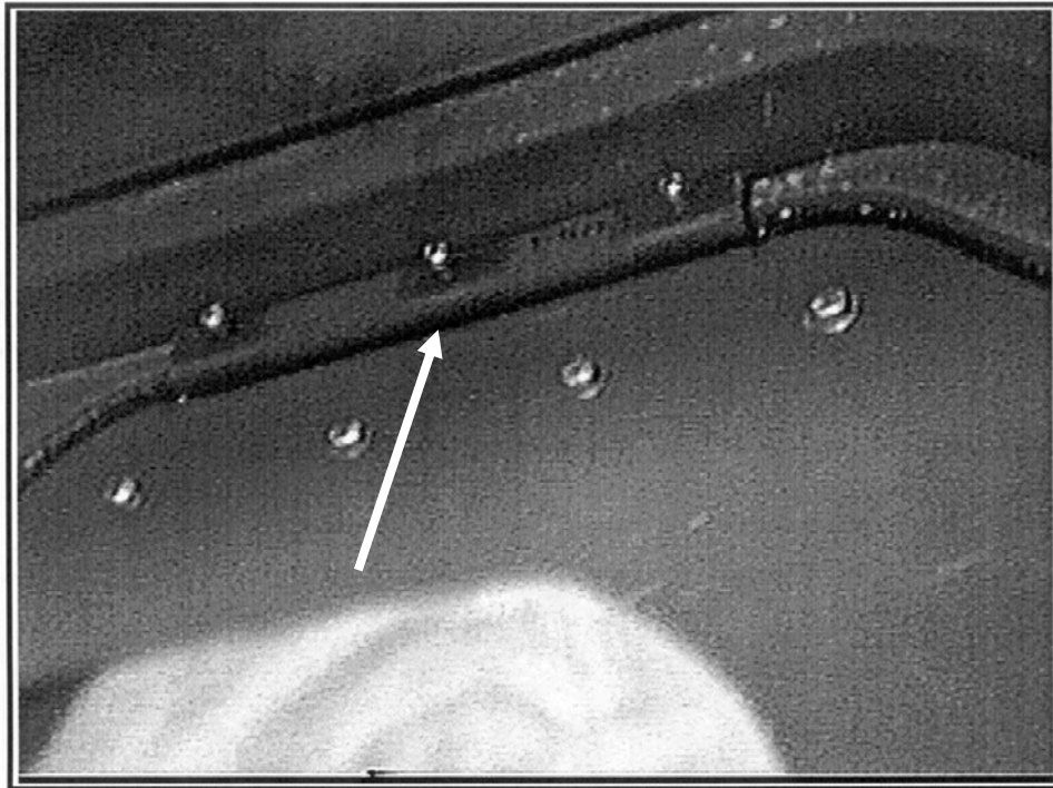
Figure 28. Slide the Mounting Armor Brackets over the rear cab window opening edges.
