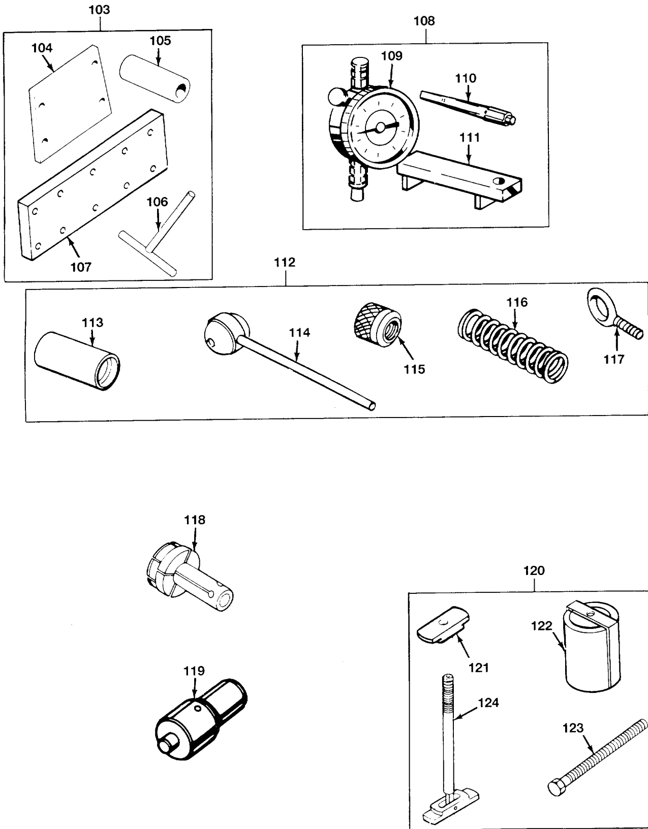
FIG.476 GENERAL SUPPORT SPECIAL TOOLS (SHEET 6 OF 8)
