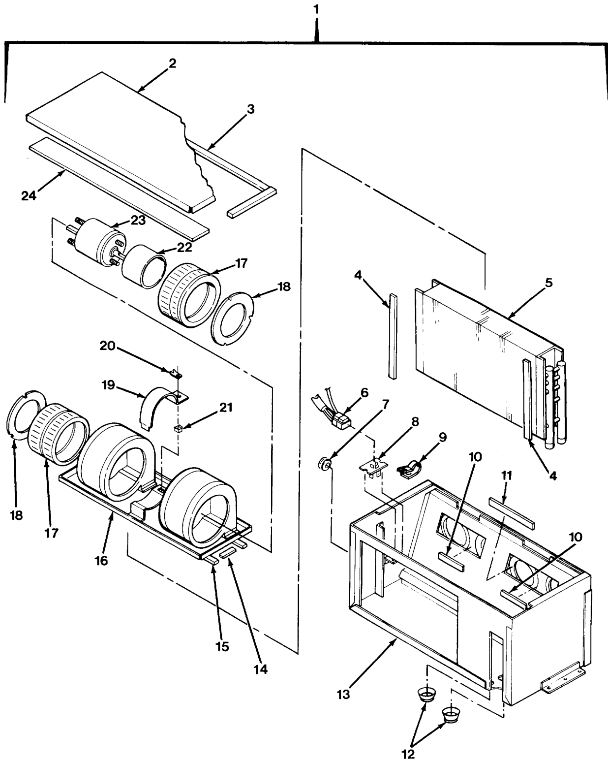
FIG. 400 HEATER ASSEMBLY
