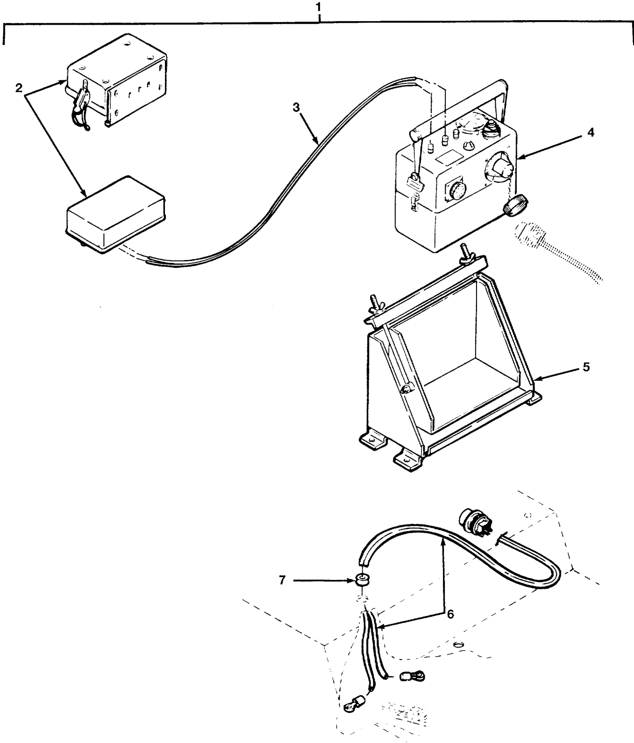
FIG. 473 M8 CHEMICAL ALARM INSTALLATION (SHEET 1 OF 2)
