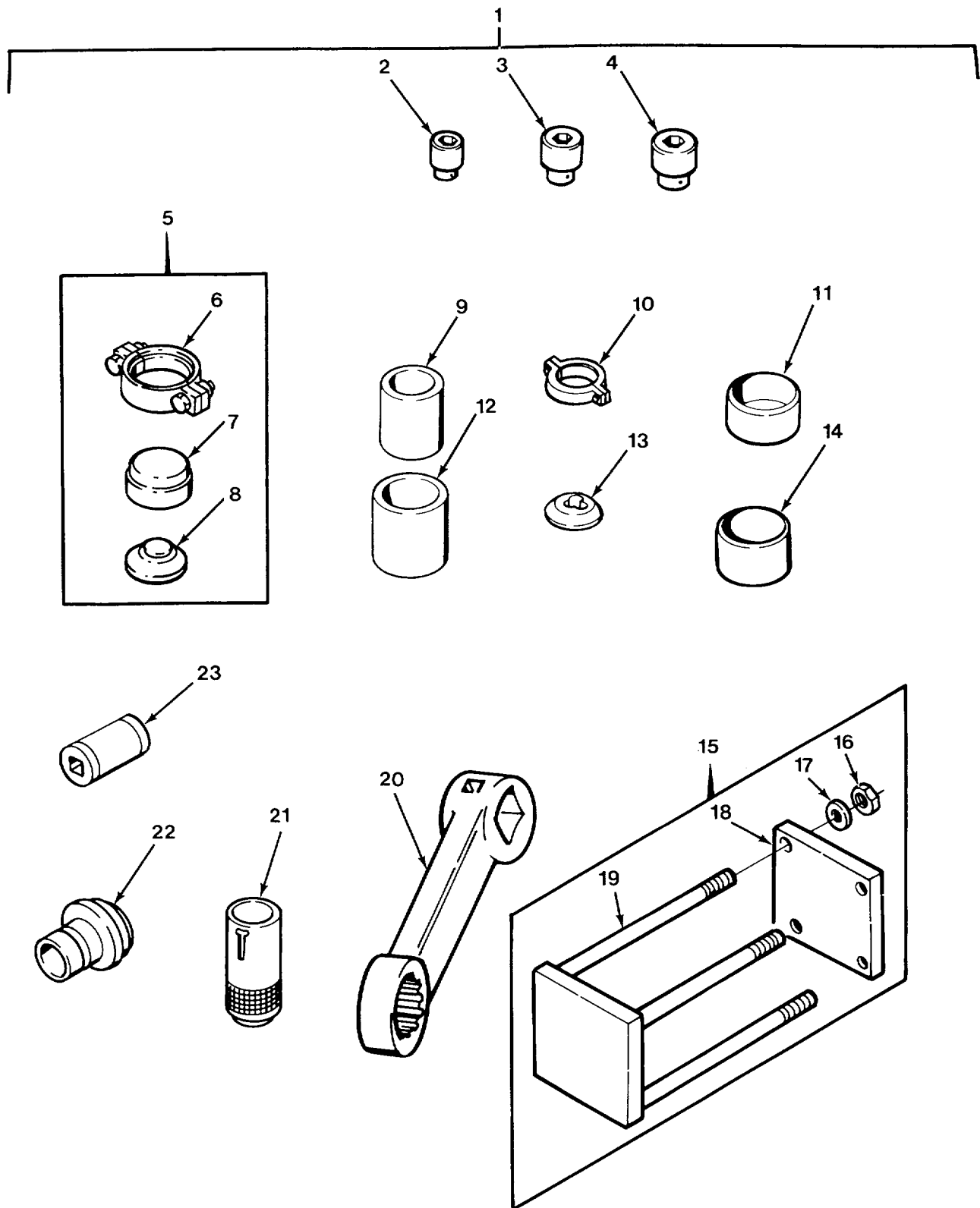
FIG.475 DIRECT SUPPORT SPECIAL TOOLS (SHEET 1 OF 3)
