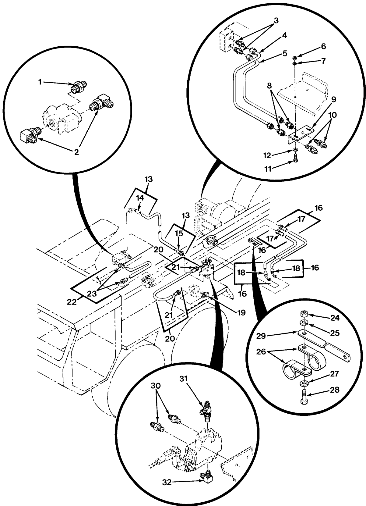
FIG. 419 HYDRAULIC LINES AND FITTINGS - M985E1 WITH WINCH (SHEET 1 OF 3)
