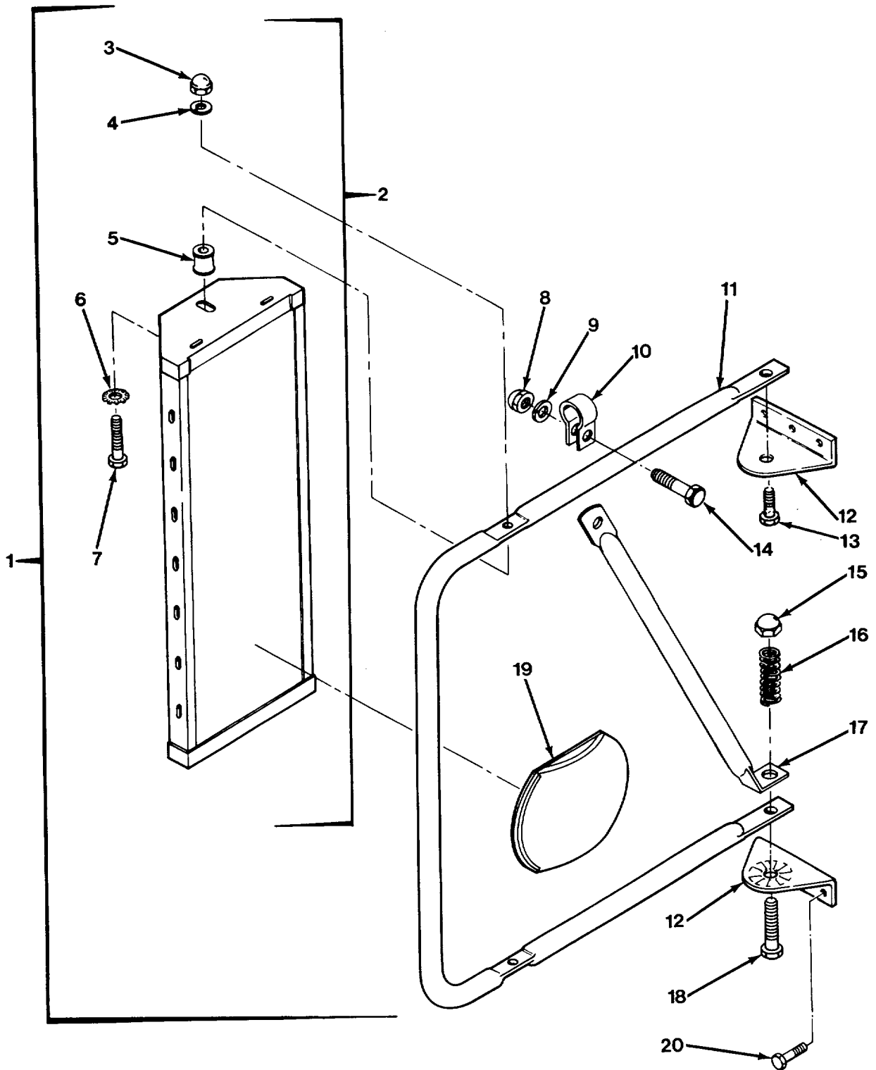
FIG. 392 MIRROR ASSEMBLY
