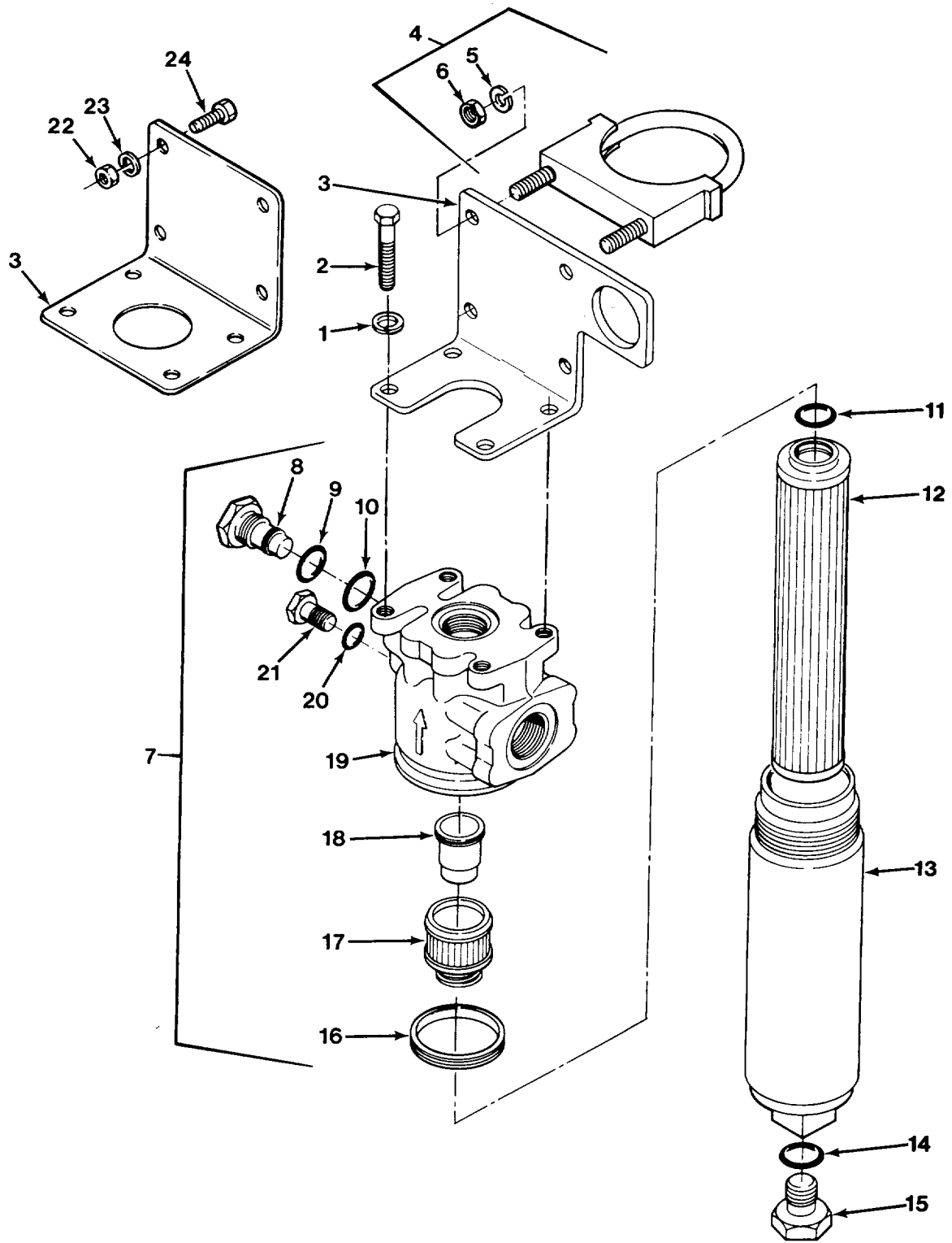
FIG. 412 CRANE HYDRAULIC FILTER - M977, M984A1 AND M985
