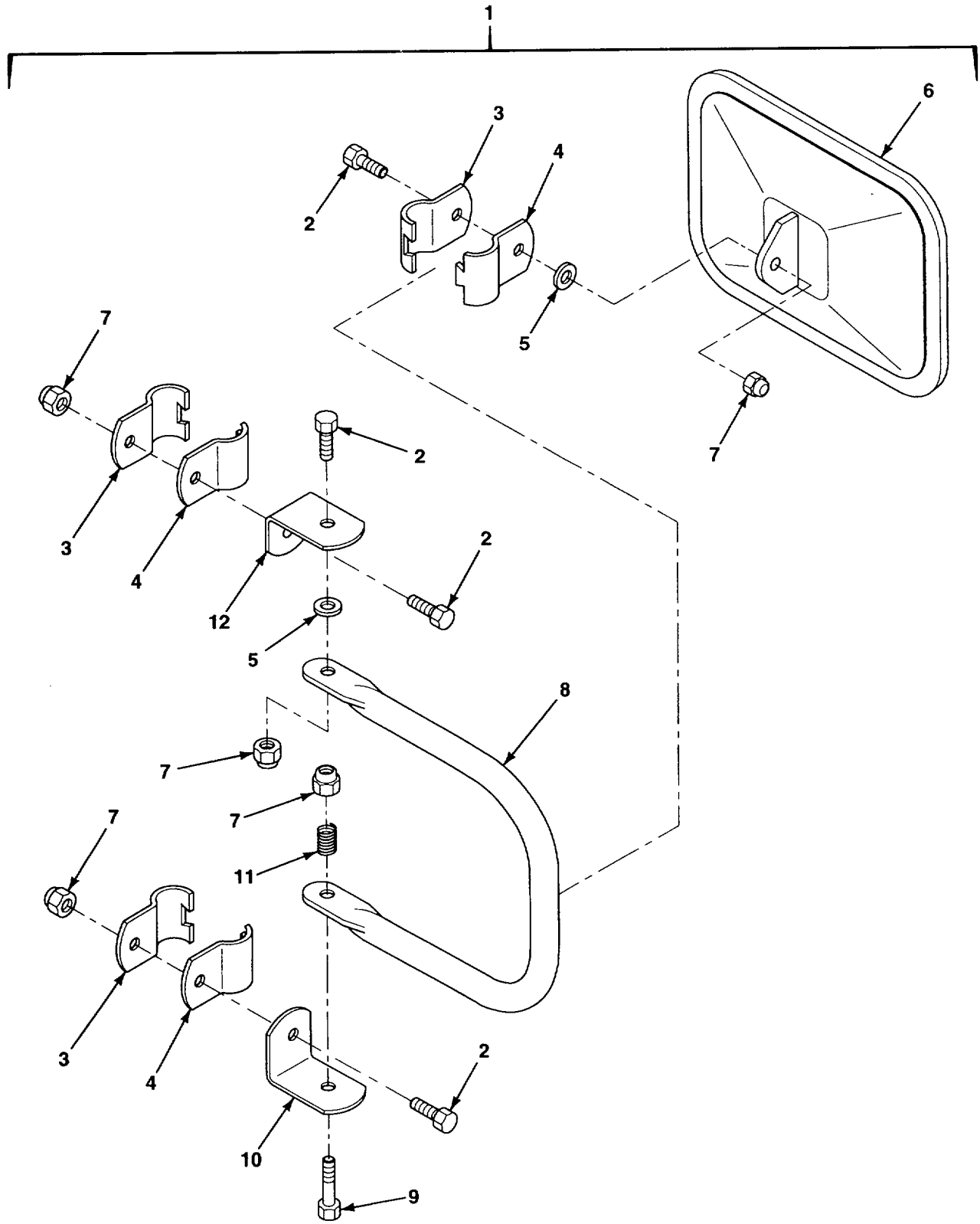
FIG. 393 EXTENSION MIRROR ASSEMBLY - M984A1
