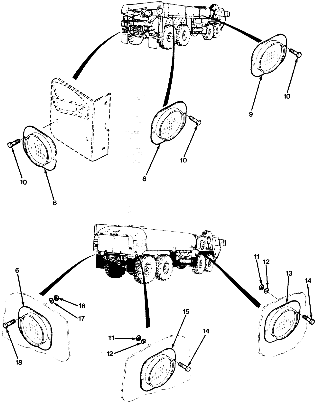
FIG. 394 REFLECTORS (SHEET 2 OF 3)
