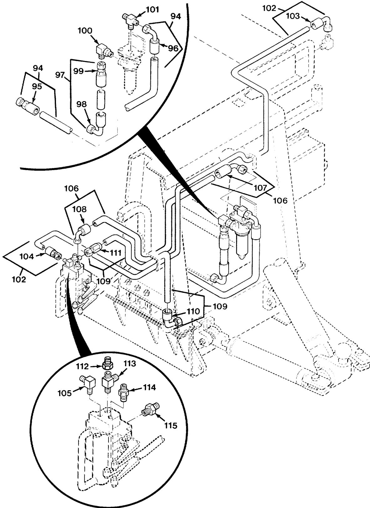
FIG. 420 HYDRAULIC LINES AND FITTINGS - M984A1 (SHEET 4 OF 5)
