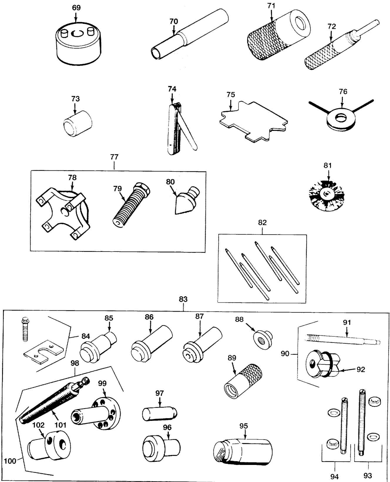
FIG.476 GENERAL SUPPORT SPECIAL TOOLS (SHEET 5 OF 8)
