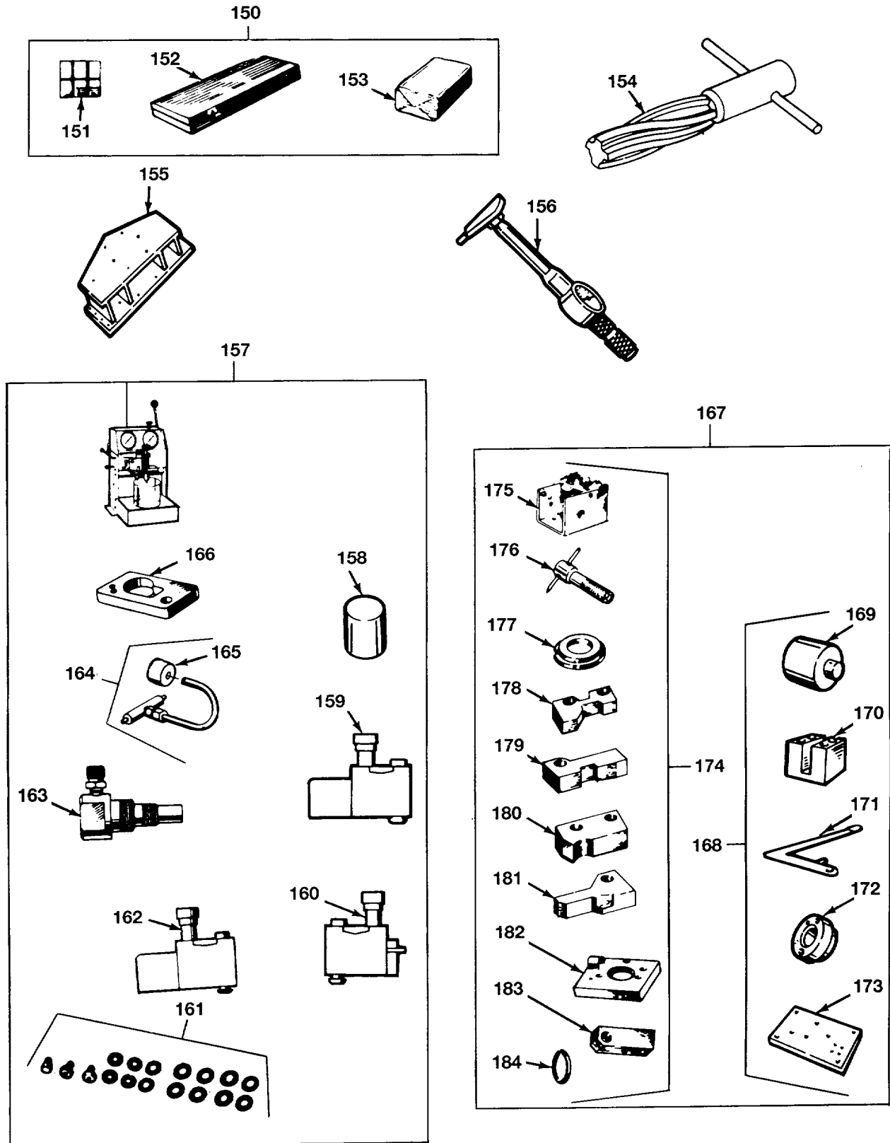
FIG.476 GENERAL SUPPORT SPECIAL TOOLS (SHEET 8 OF 8)
