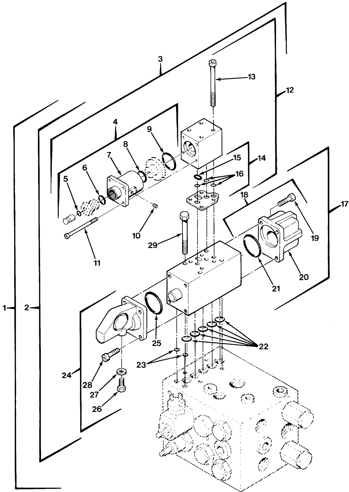
FIG.410 HEAVY DUTY WINCH MANIFOLD - M984A1 (SHEET 1 OF 3)
