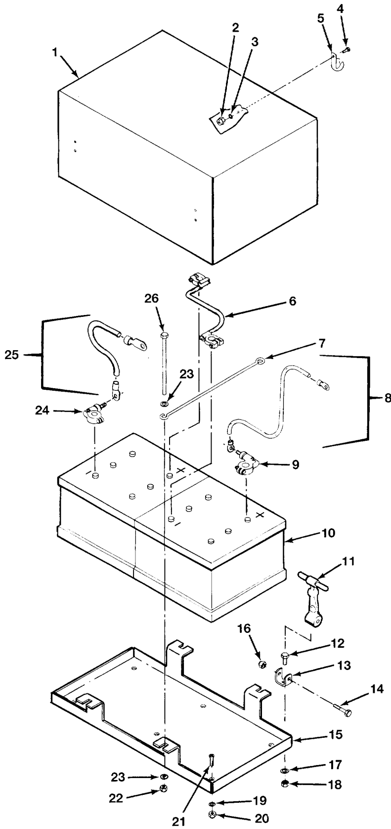
FIG. 427 ARCTIC BATTERY INSTALLATION
