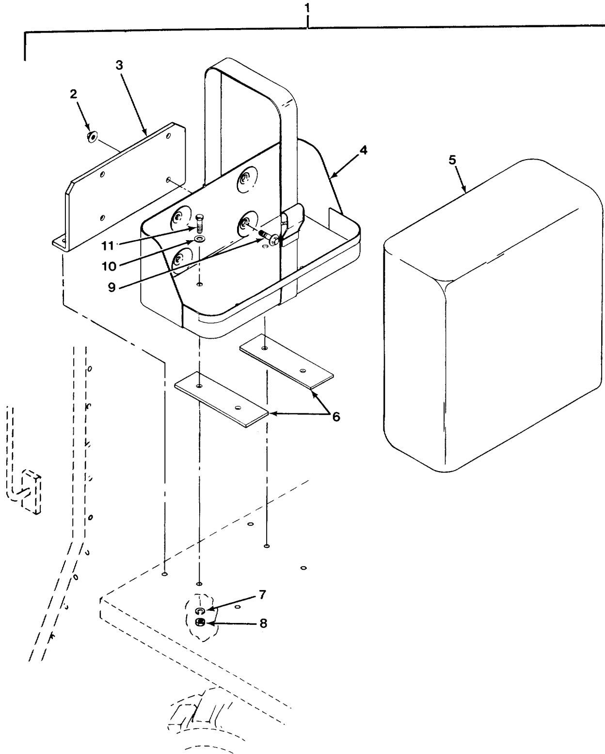
FIG. 472 M13 DECONTAMINATION UNIT INSTALLATION
