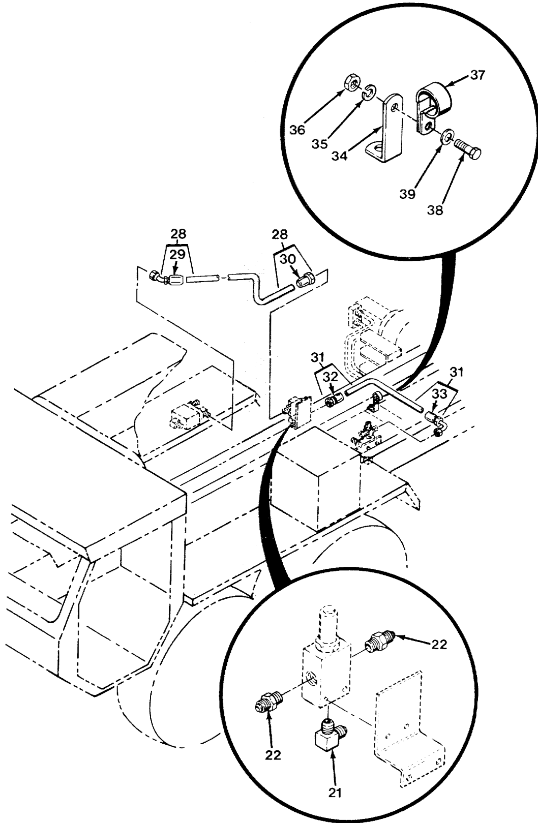
FIG. 417 HYDRAULIC LINES AND FITTINGS - M983 WITHOUT CRANE (SHEET 2 OF 3)
