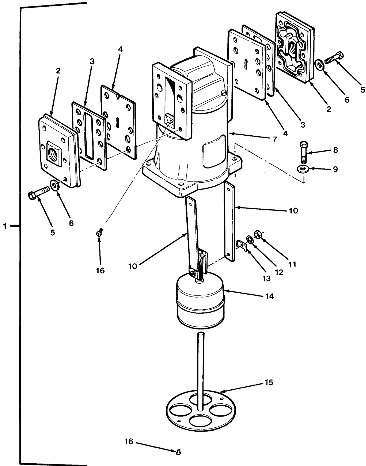
FIG. 447 AIR ELIMINATOR
