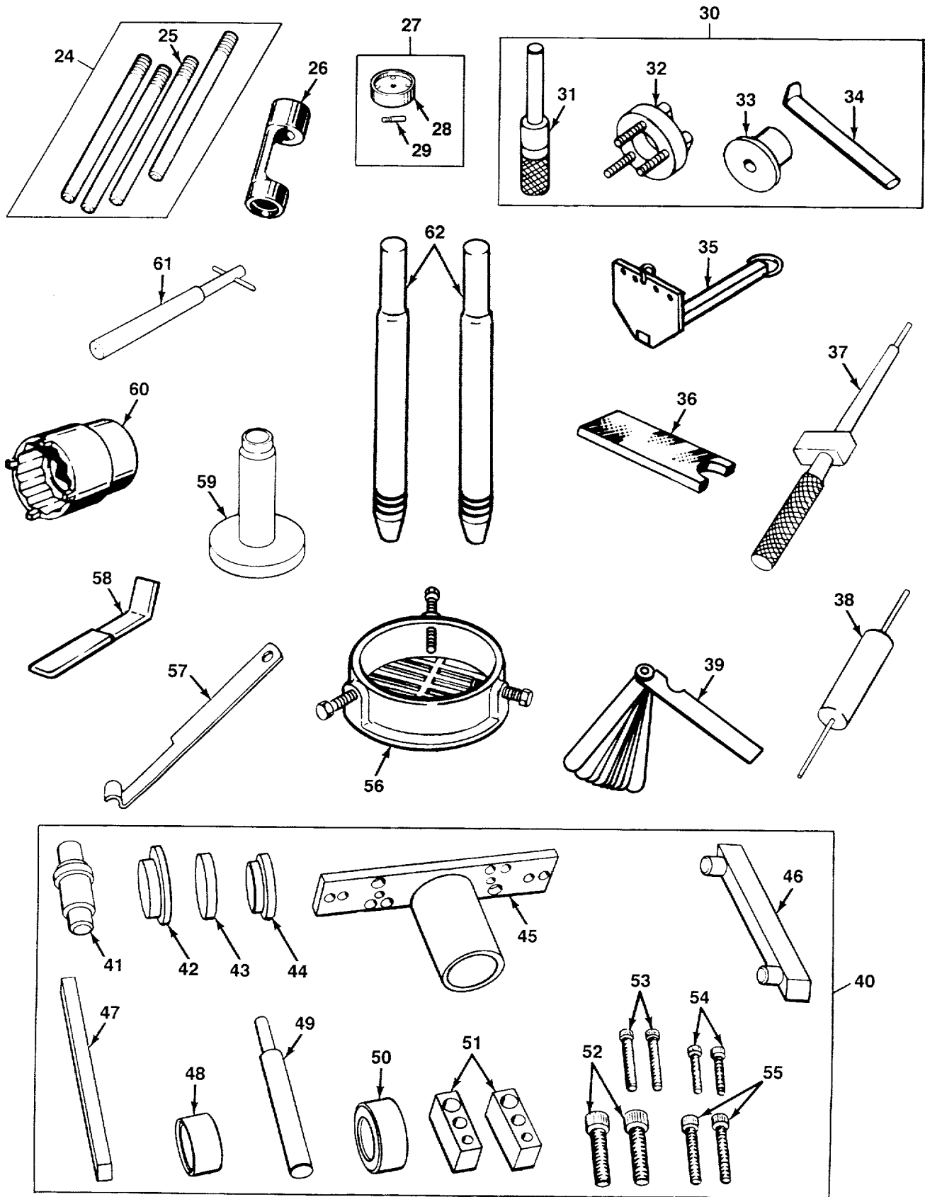
FIG.475 DIRECT SUPPORT SPECIAL TOOLS (SHEET 2 OF 3)
