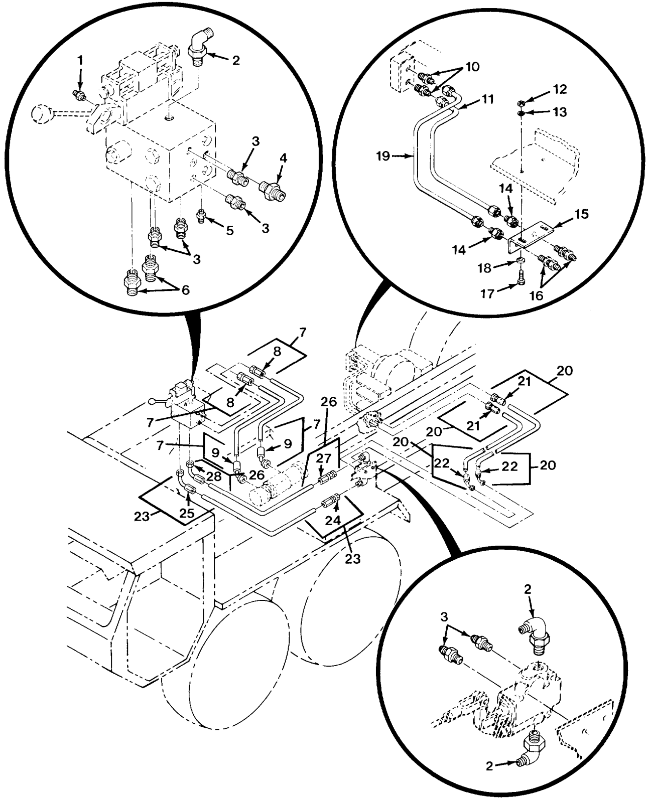
FIG. 420 HYDRAULIC LINES AND FITTINGS - M984A1 (SHEET 1 OF 5)
