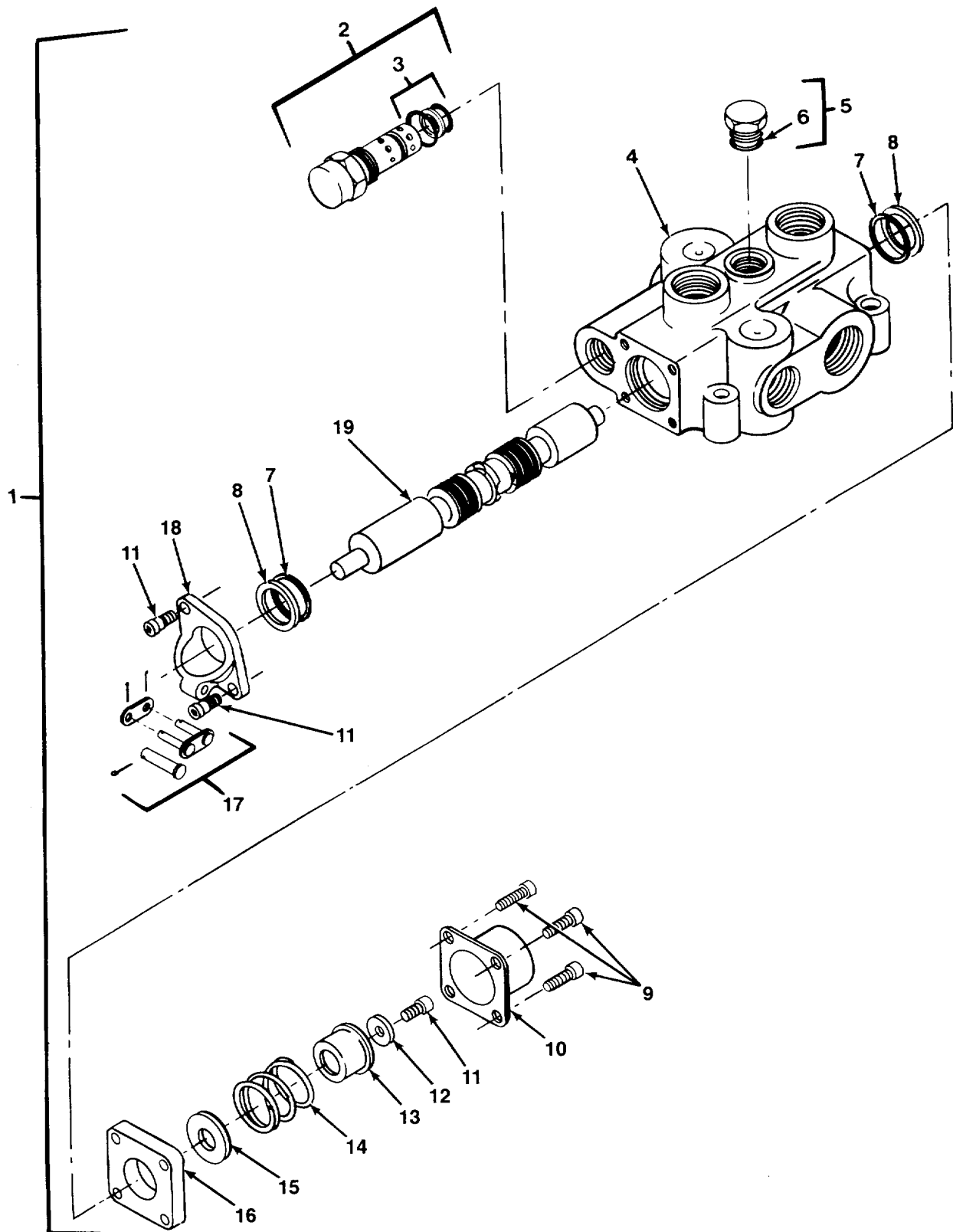
FIG.405 SELF RECOVERY WINCH CONTROL VALVE ASSEMBLY
