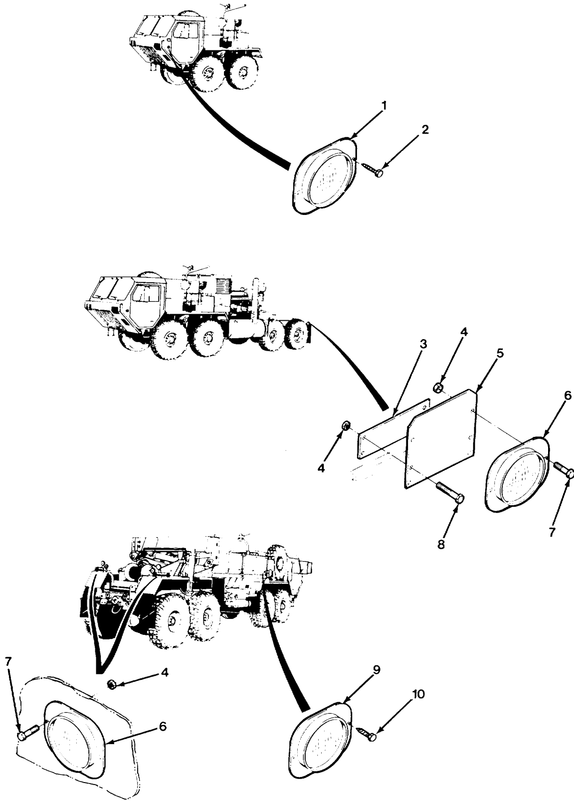
FIG. 394 REFLECTORS (SHEET 1 OF 3)
