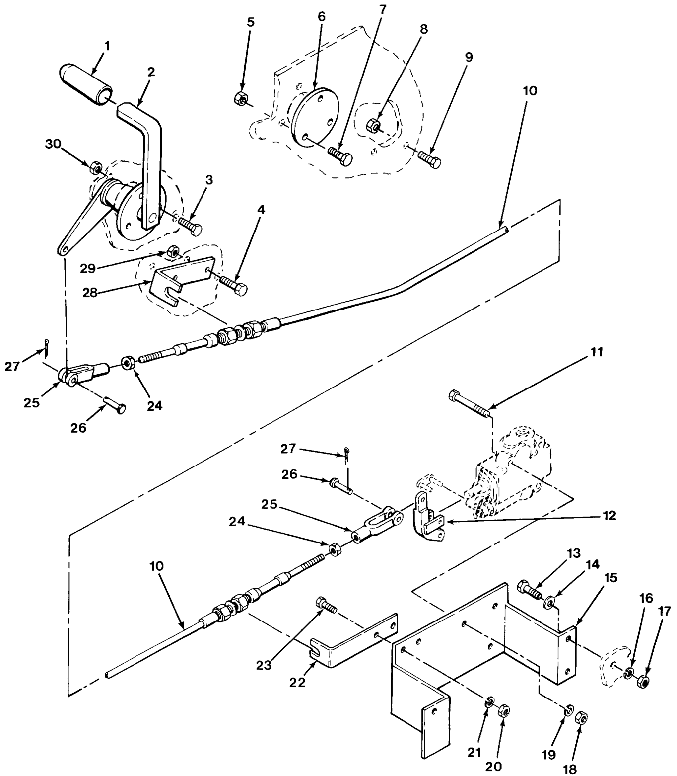
FIG. 404 SELF RECOVERY WINCH CONTROL VALVE MOUNTING
