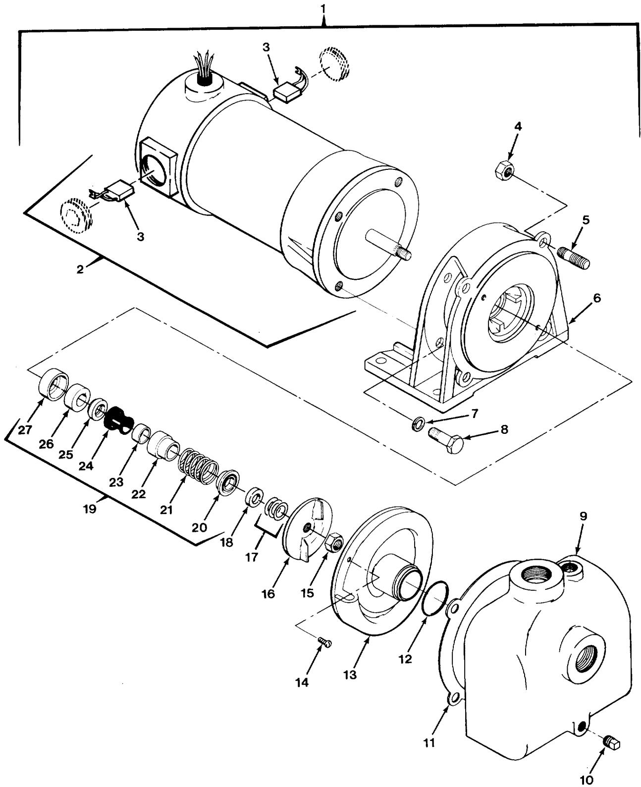
FIG. 444 AUXILIARY PUMP
