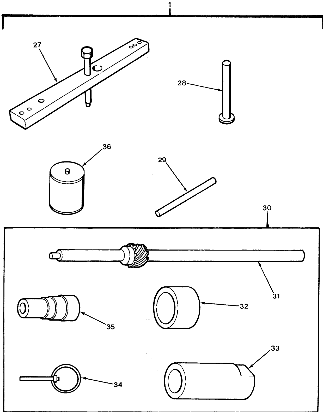
FIG.476 GENERAL SUPPORT SPECIAL TOOLS (SHEET 3 OF 8)
