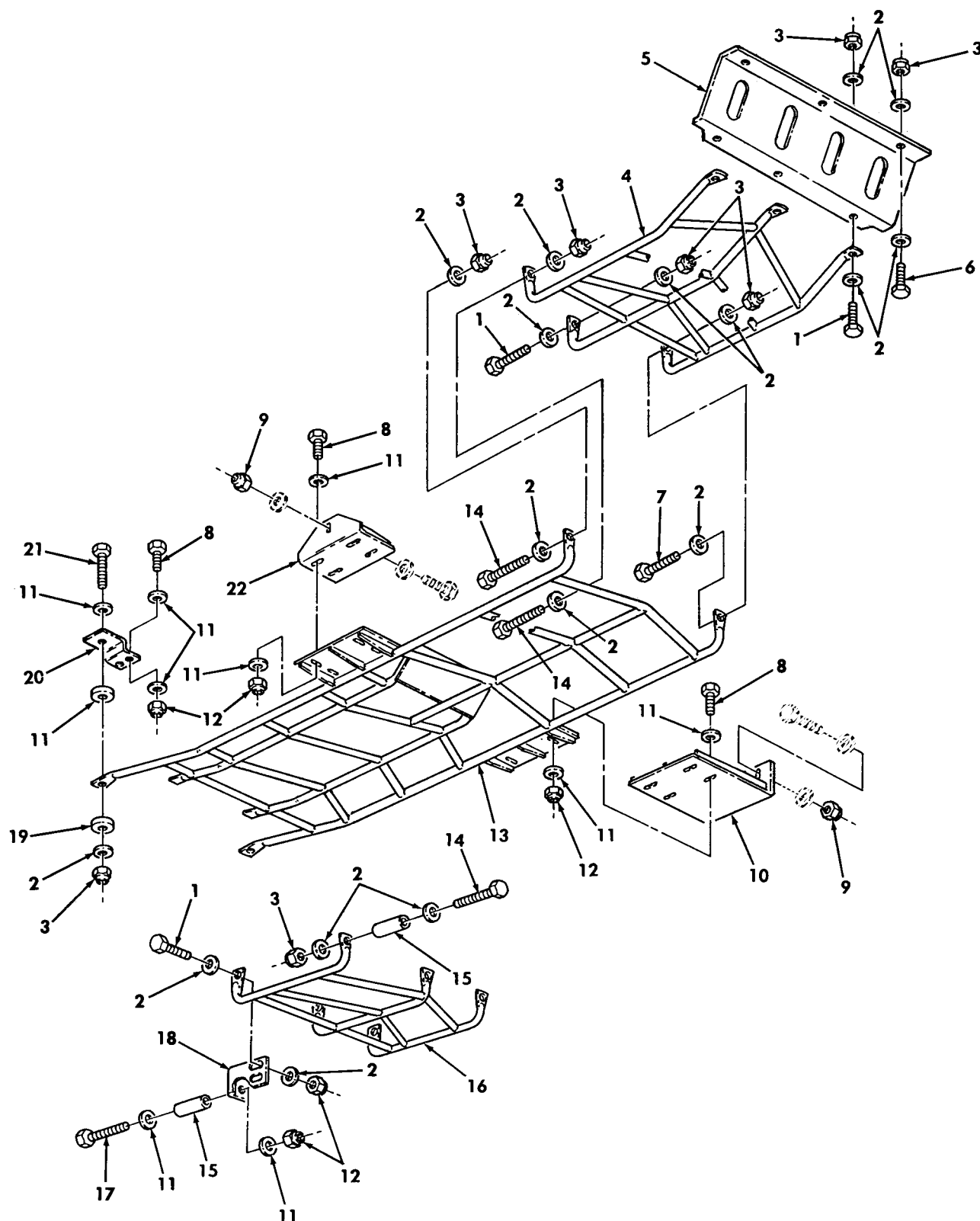
Figure 463. Underbody Protection Kit With and Without Winch.
