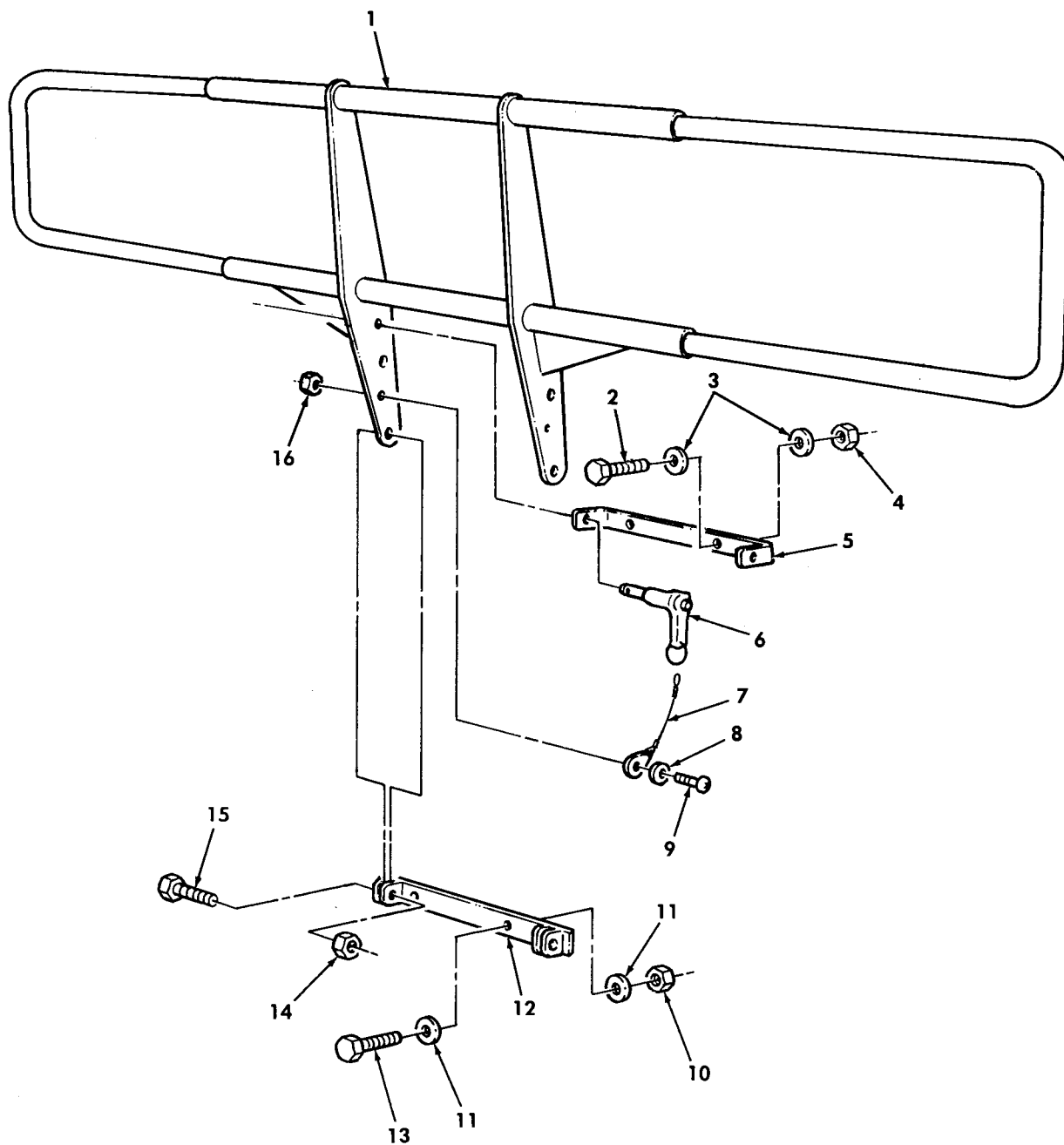
Figure 462. Brushguard Kit.
