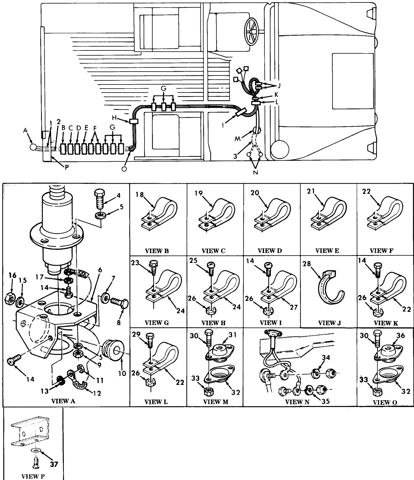
Figure 410. Communications Kit, Radio Cables, AN/GRC-160, AN/VRC-46, and TSEC/KY-57.
