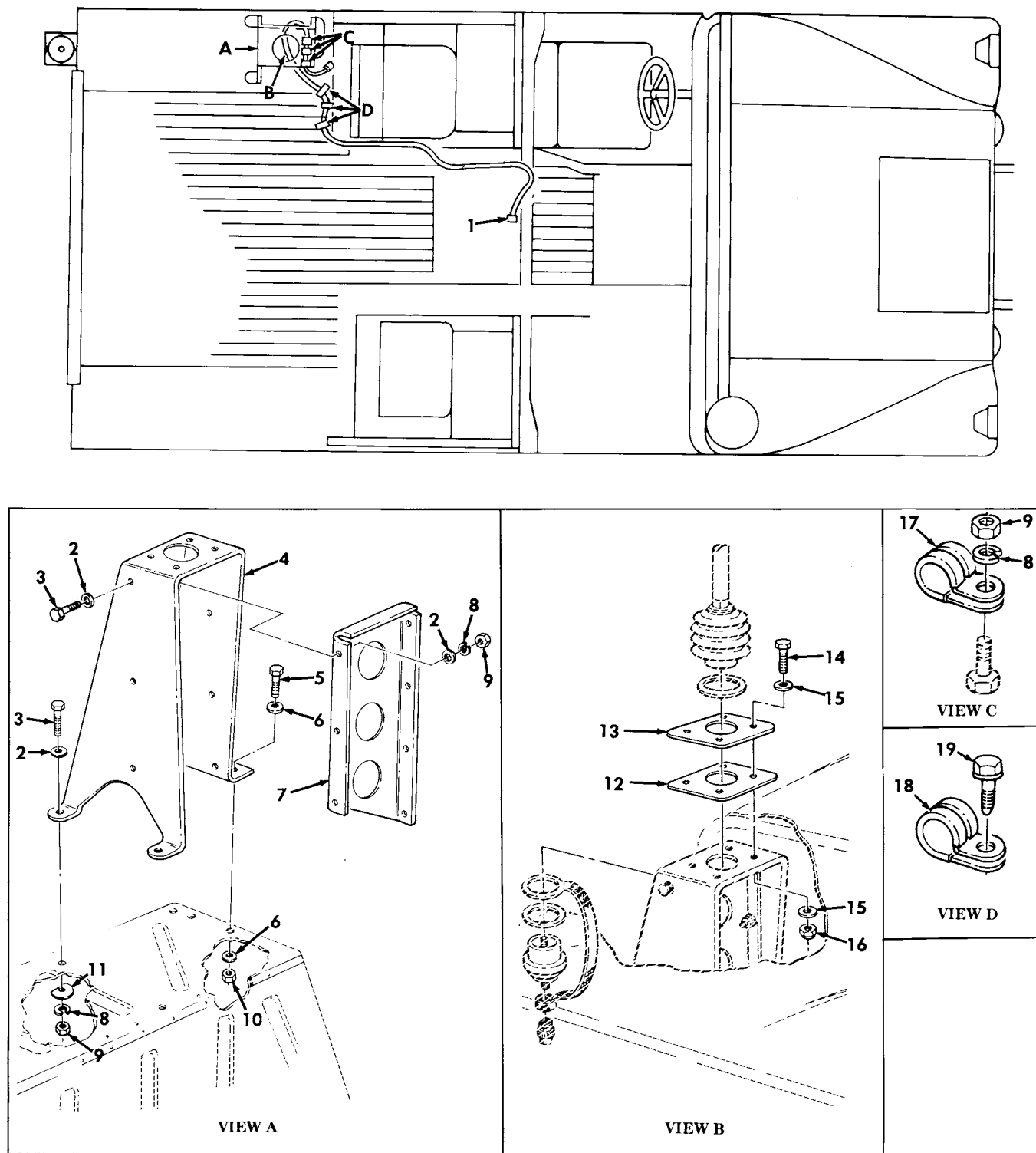
Figure 425. Communications Kit, Radio Cables, AN/VRC-47 and AN/VRC-48.
