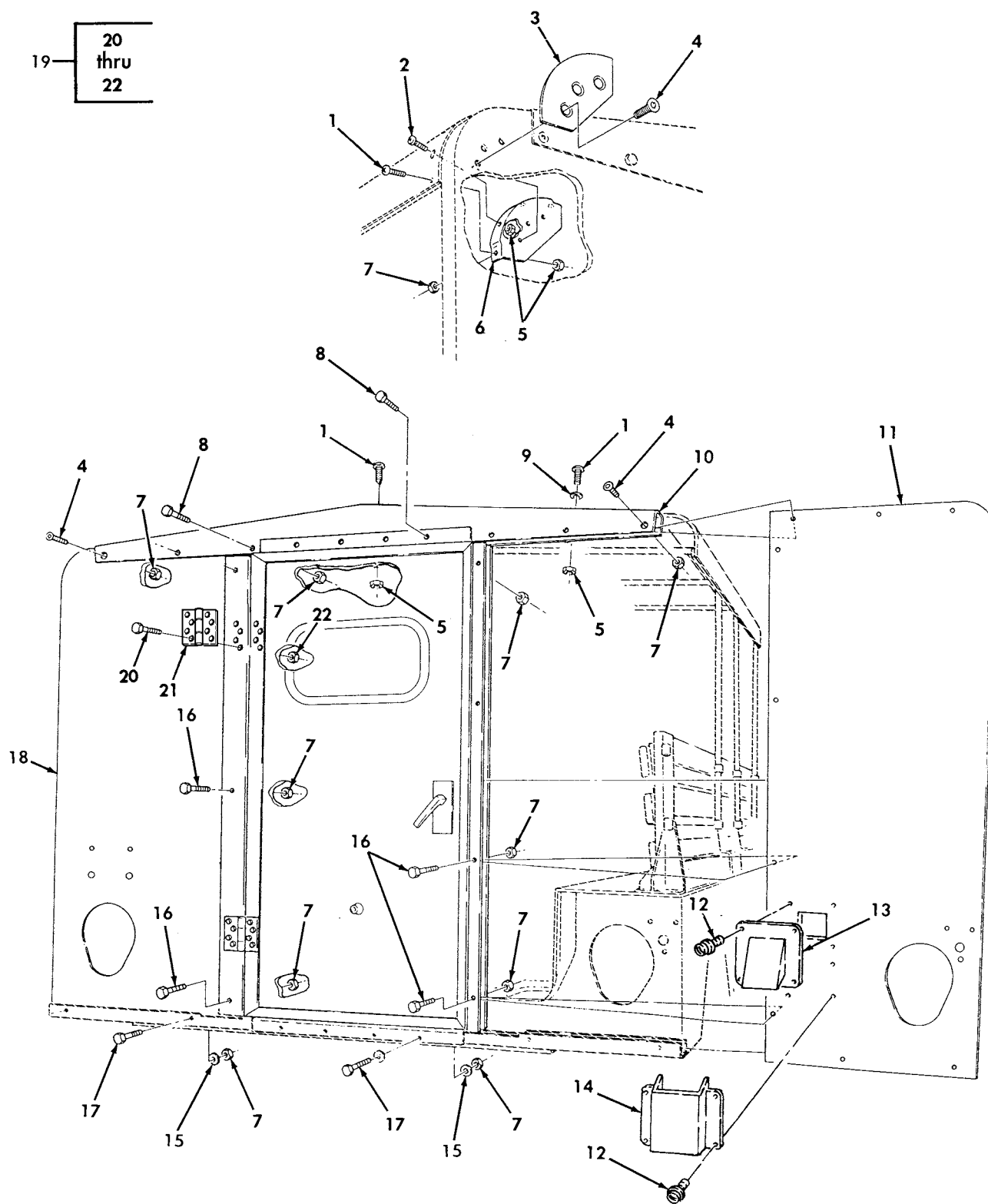
Figure 397. End Closures, Door Assembly, and Mounting Hardware.
