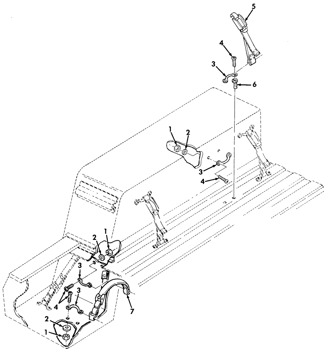
Figure 450. Kit, Prime Mover, Lt. Howitzer, 105 MM L119, Aiming Post and Cable Reel Stowage.
