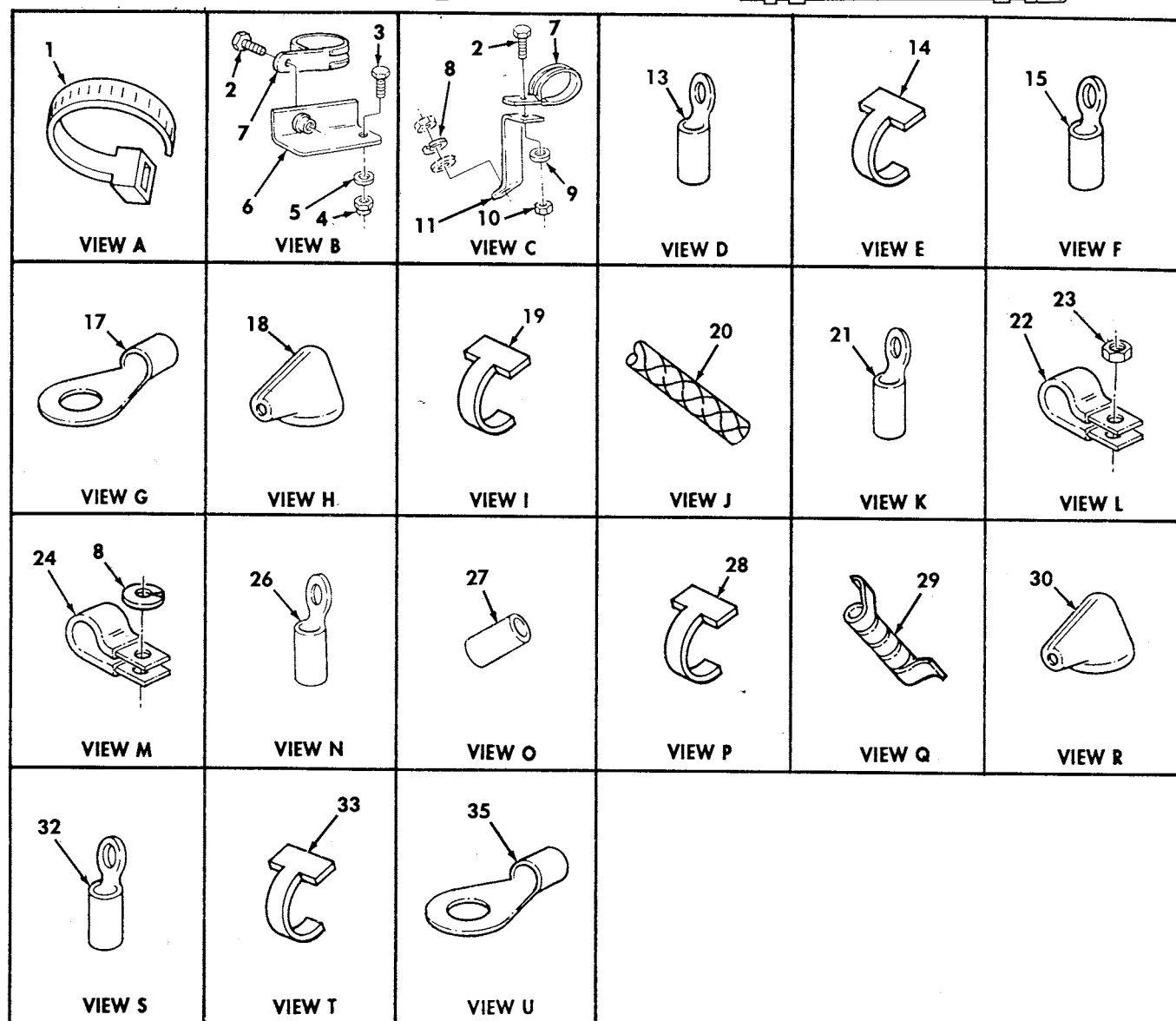
Figure 480. 400 AMP Alternator Wiring Harness Cable Assemblies.
