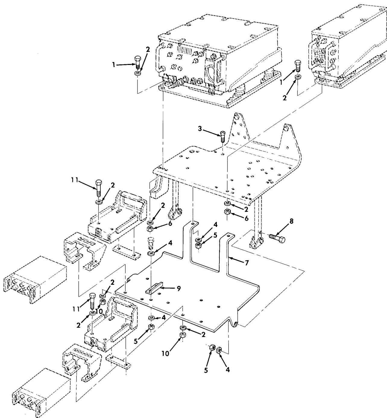
Figure 413. Communications Kit, Radio Rack Assembly, AN/VRC-47 and (2) TSEC/KY-57 Assemblies.
