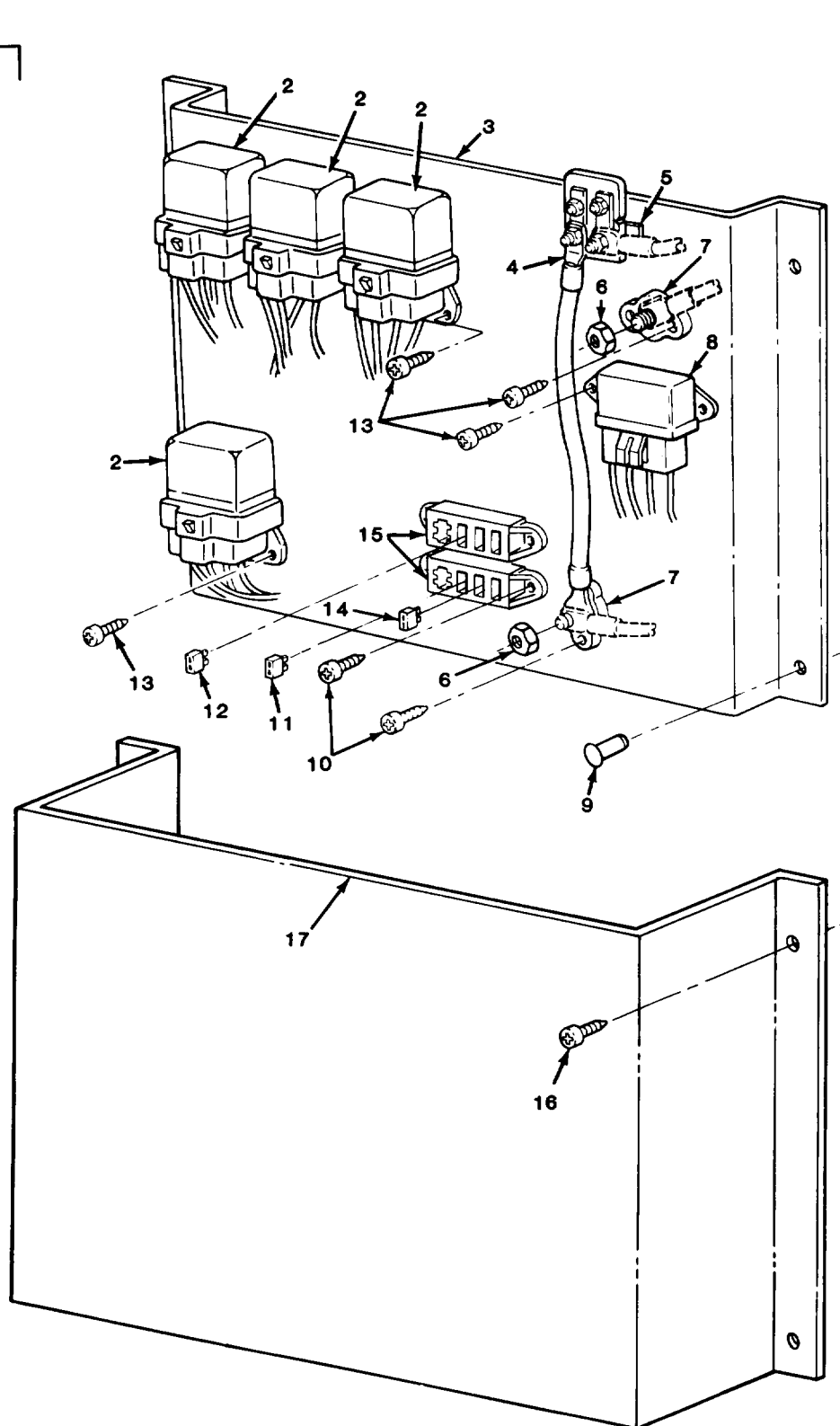
FIGURE 222. RELAY PANEL ASSEMBLY COMPONENTS AND RELATED PARTS (M1010).
