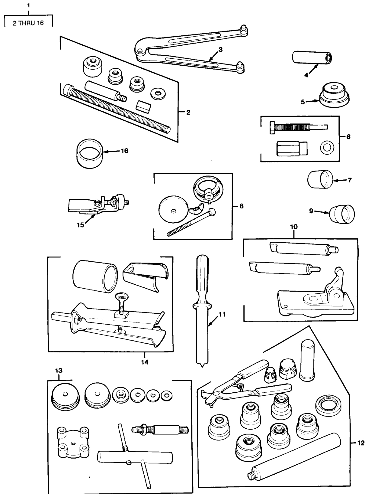
FIGURE 303. SPECIAL TOOLS.
