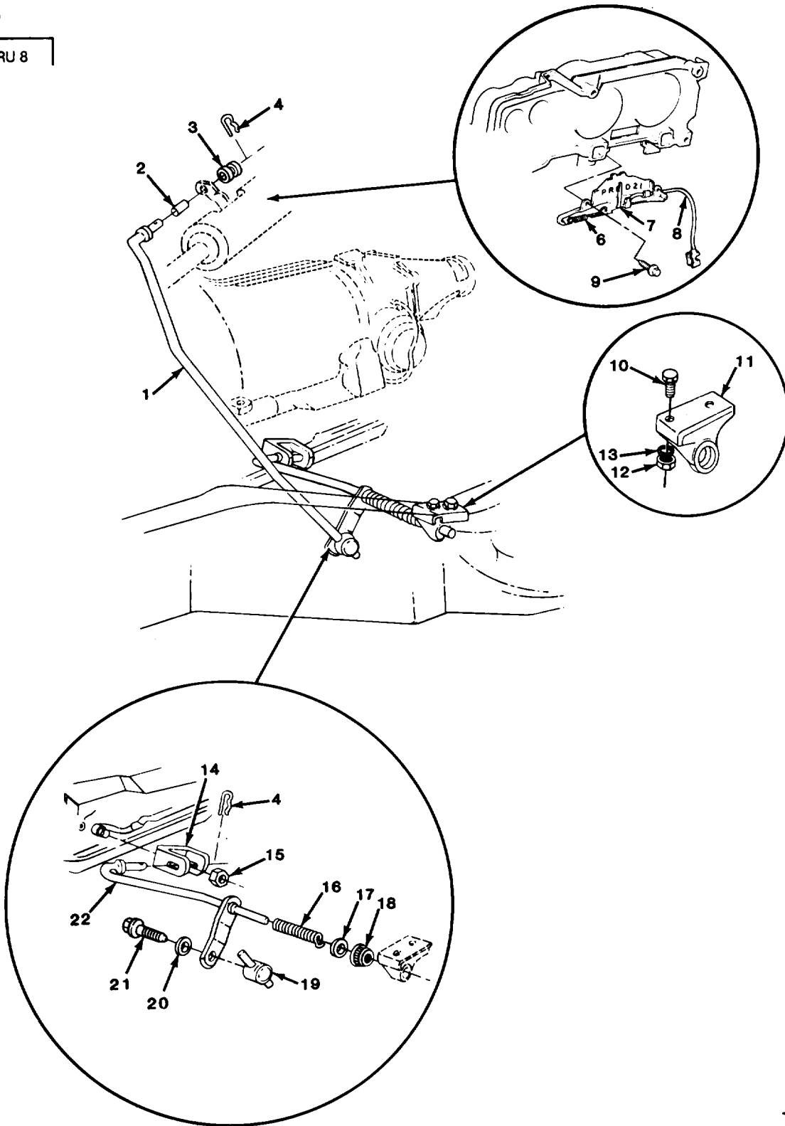
FIGURE 69. SHIFTING LINKAGE.
