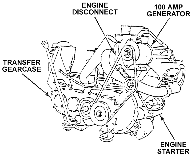
Figure 1-4. M548A1 Powerplant
