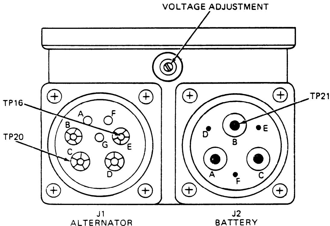
Figure 2-6. End view-model 03.
