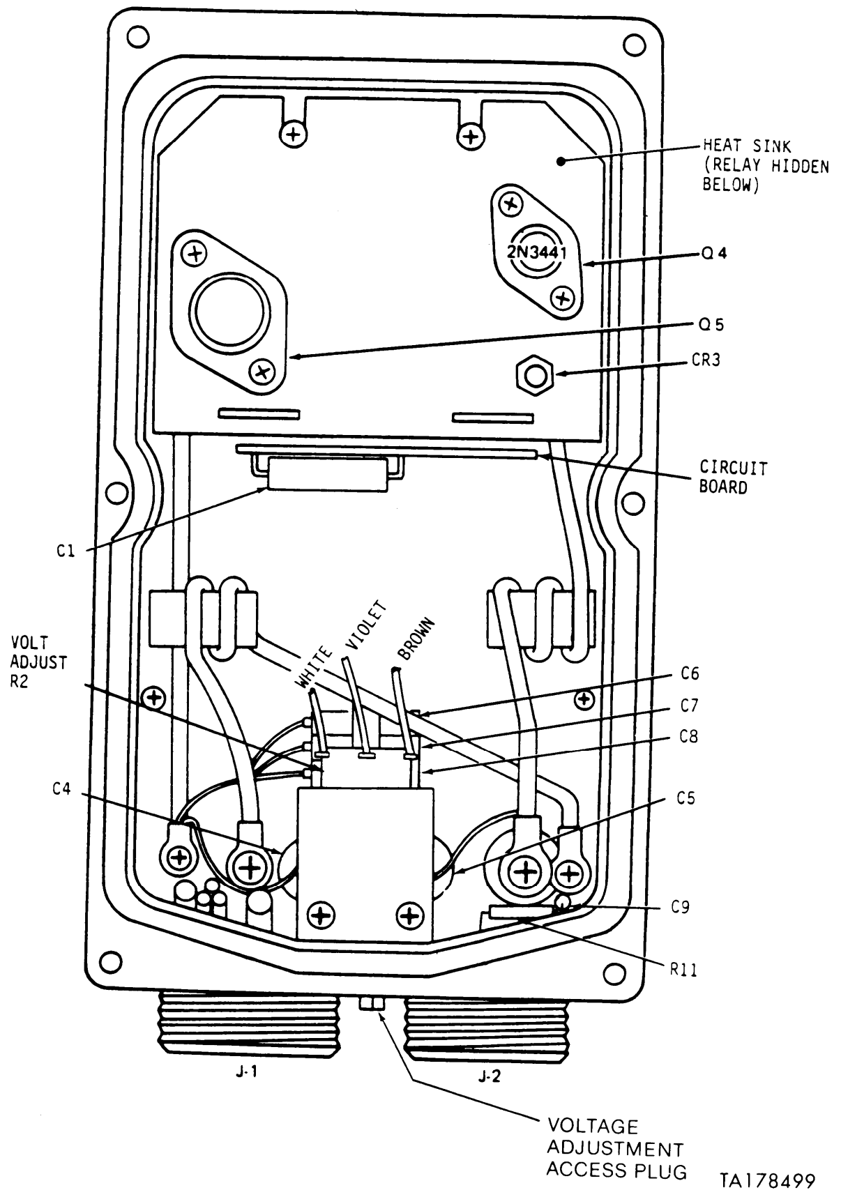
Figure 2-17. Vap-Air model 26440001-05.
