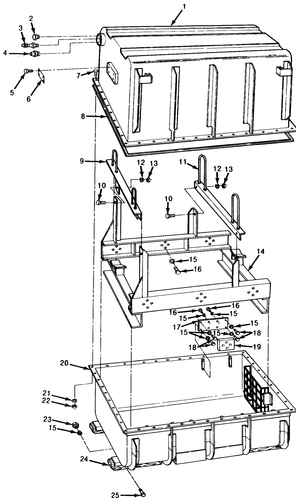
Figure 24. Transmission Assembly Container -- Exploded View
