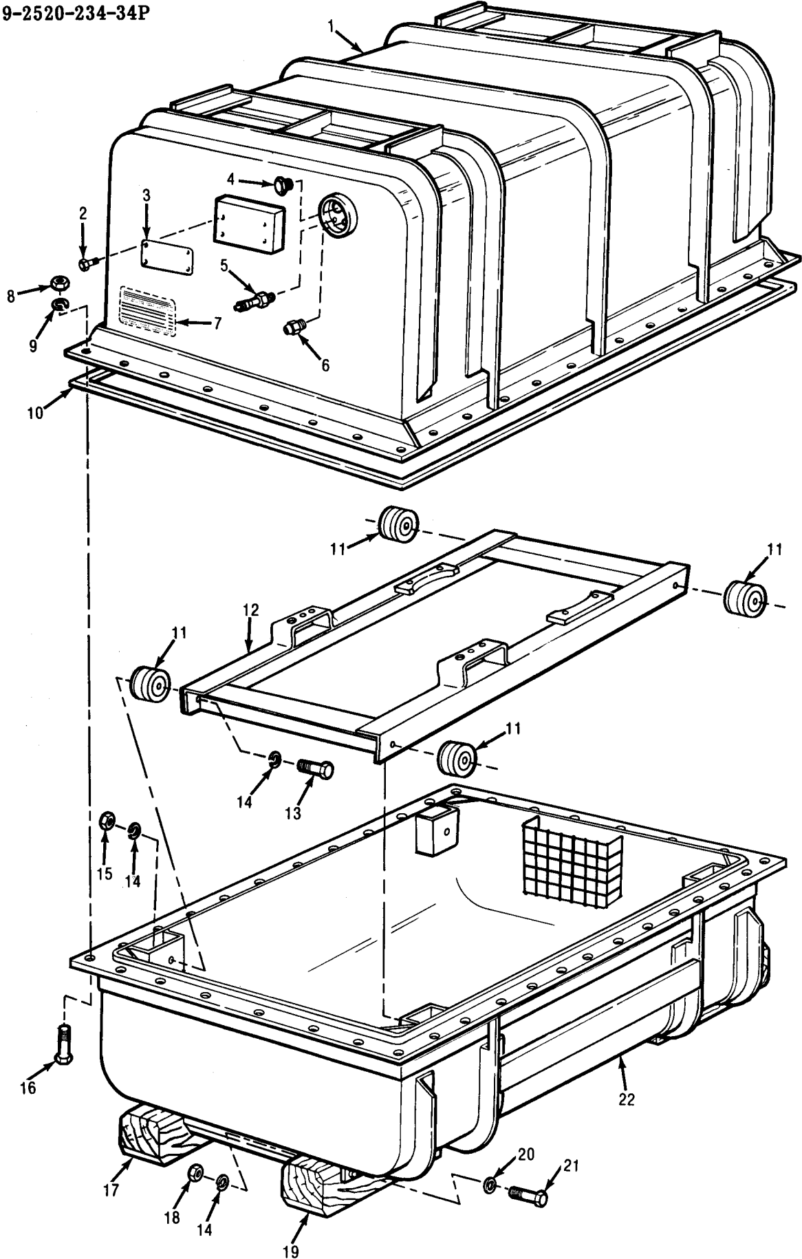
Figure 25. Input Transfer Assembly Container — Exploded View
