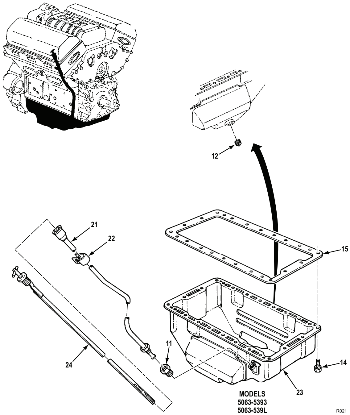
Figure 19. Oil Pan and Oil Gage Assembly. (Sheet 3 of 3)
