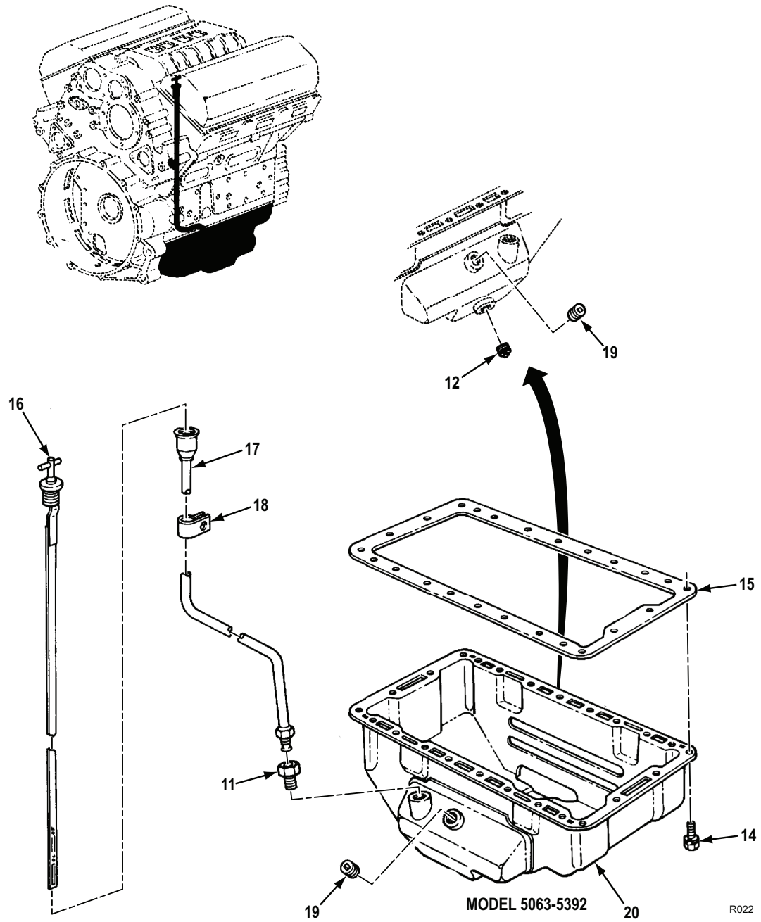
Figure 19. Oil Pan and Oil Gage Assembly. (Sheet 2 of 3)
