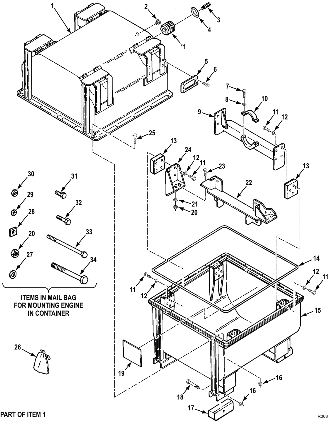
Figure 59. Shipping and Storage Container Assembly (Model 5063-5299).
