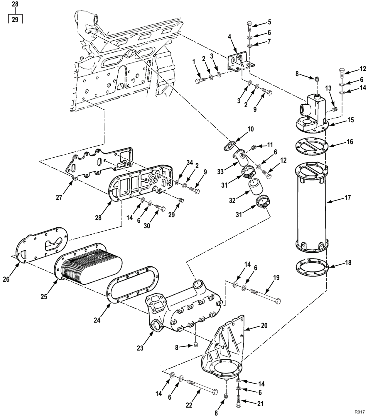
Figure 17. Oil Cooler Assembly (Model 5063-5393 and 5063-539L).
