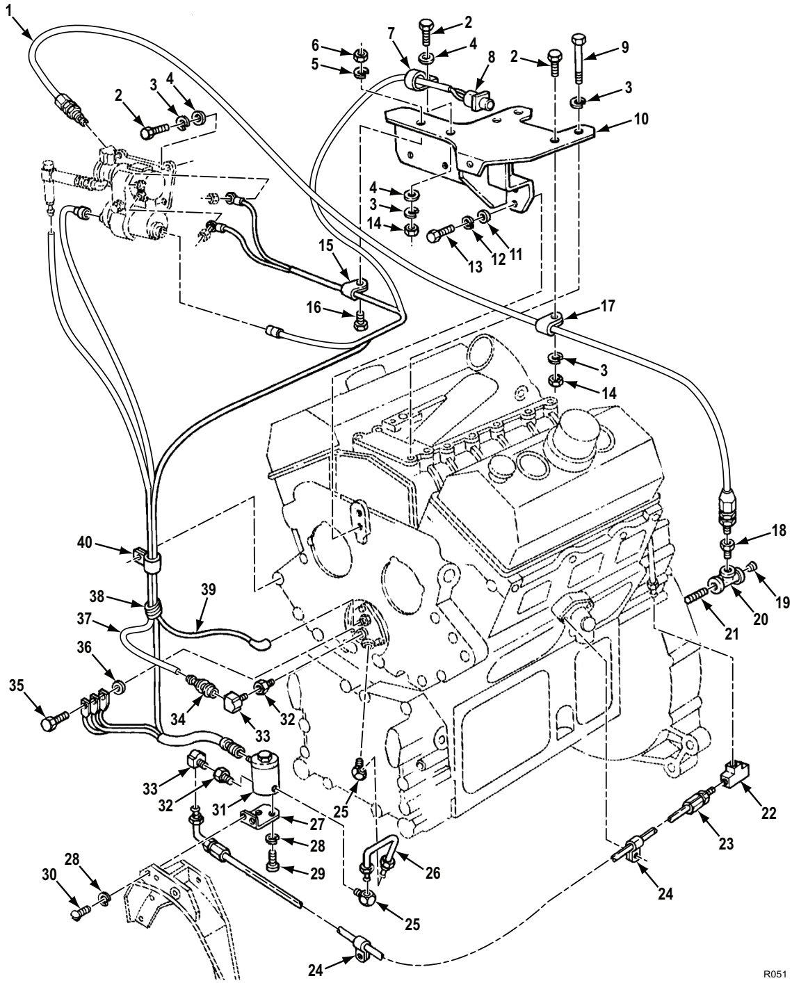
Figure 47. Air Box Heater and Related Parts (Model 5063-5392).
