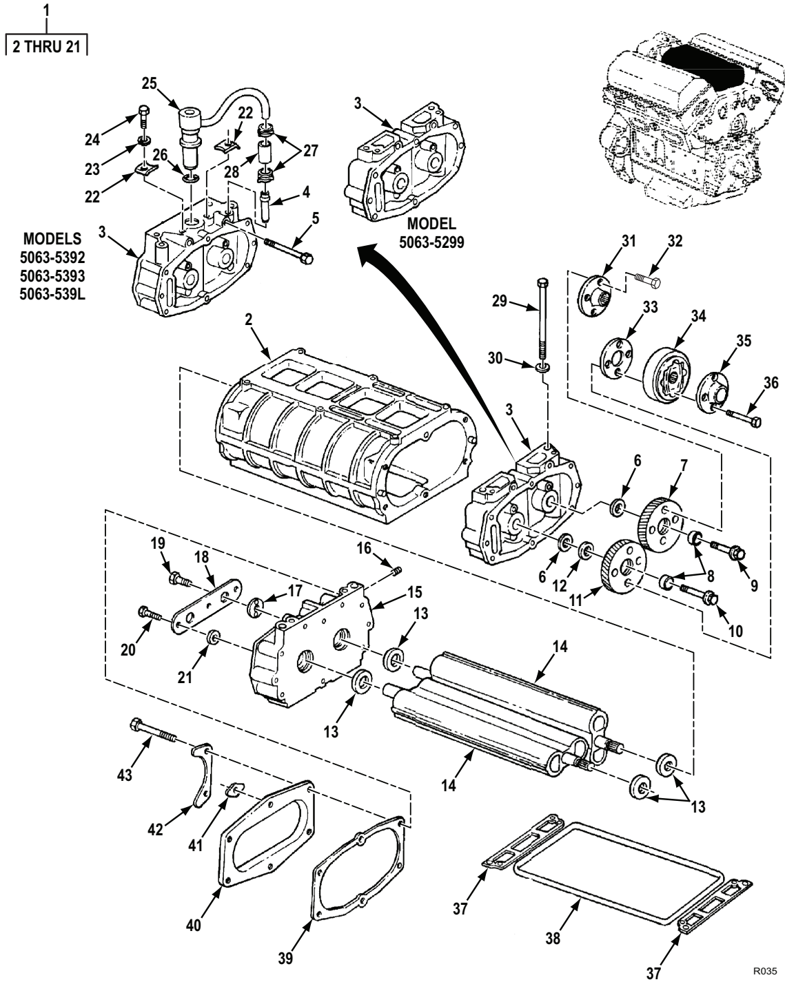
Figure 32. Blower Assembly.
