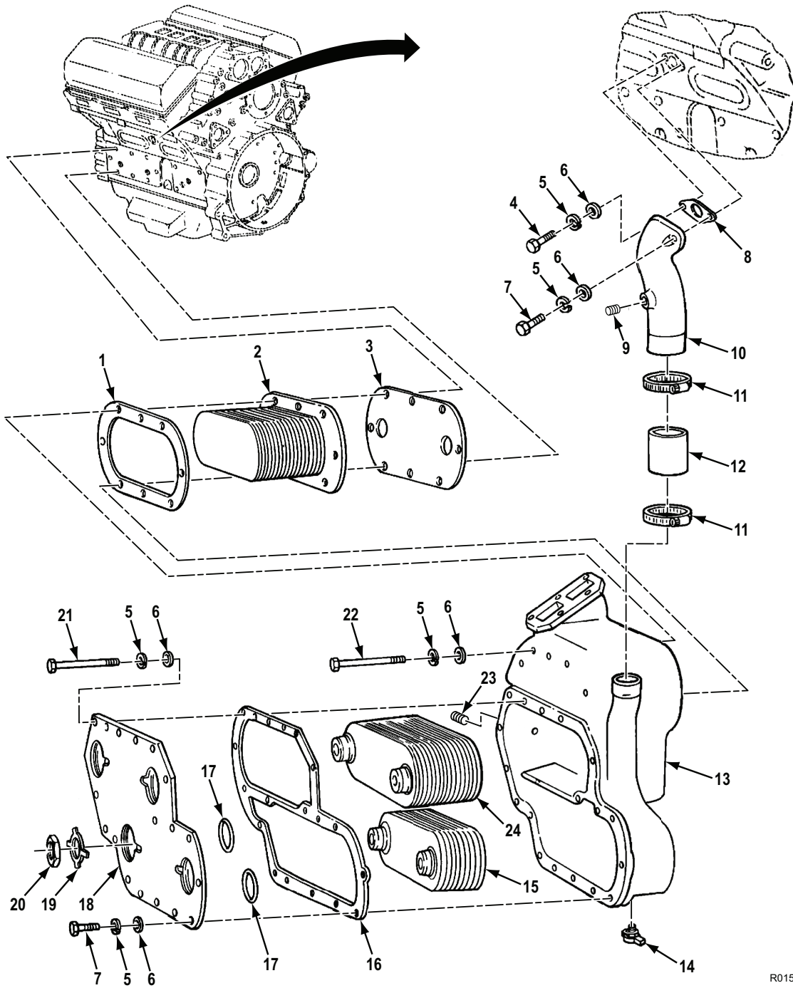
Figure 15. Oil Cooler Assembly (Model 5063-5299).
