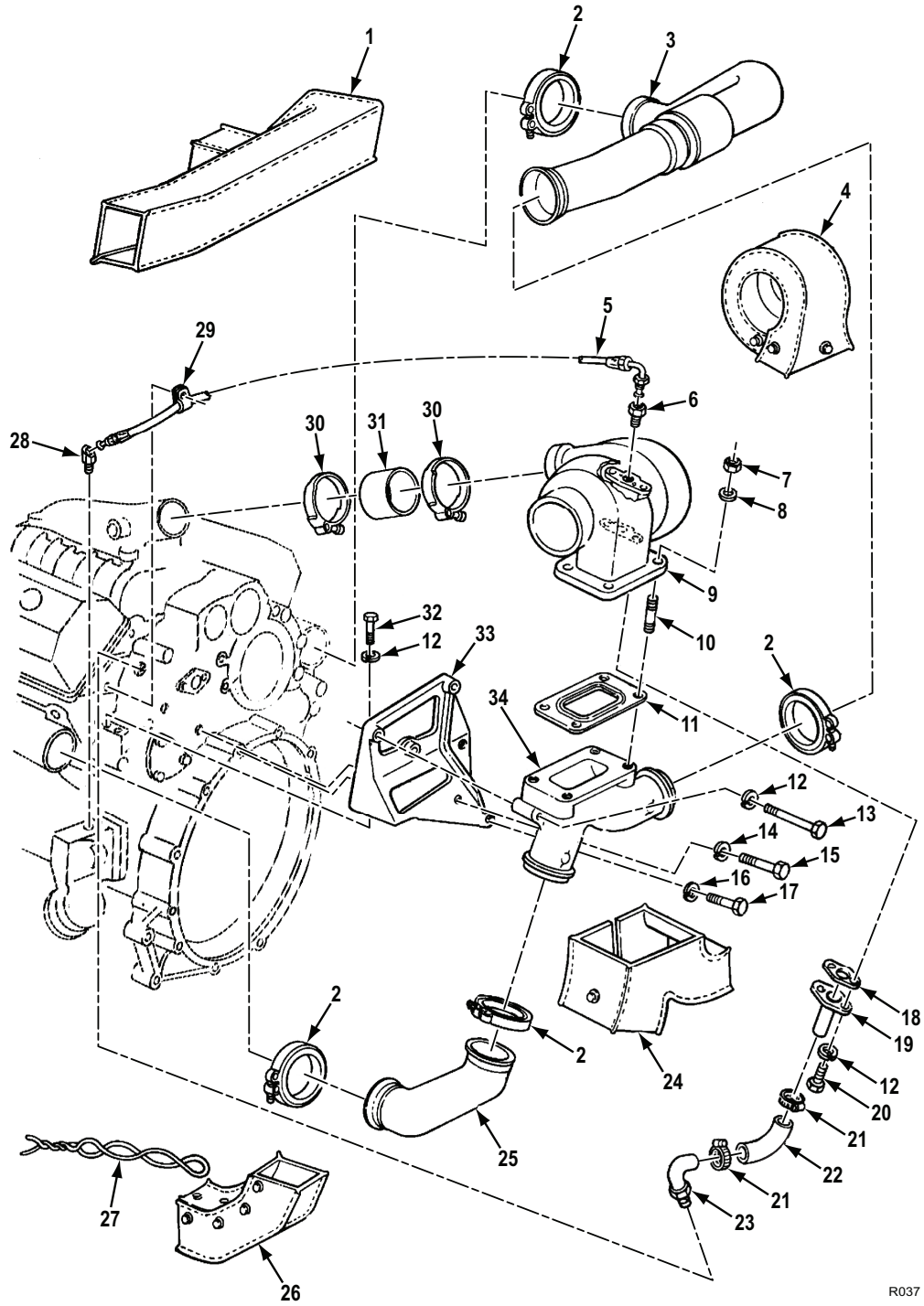
Figure 34. Turbocharger and Related Parts (Models 5063-5393 and 5063-539L).
