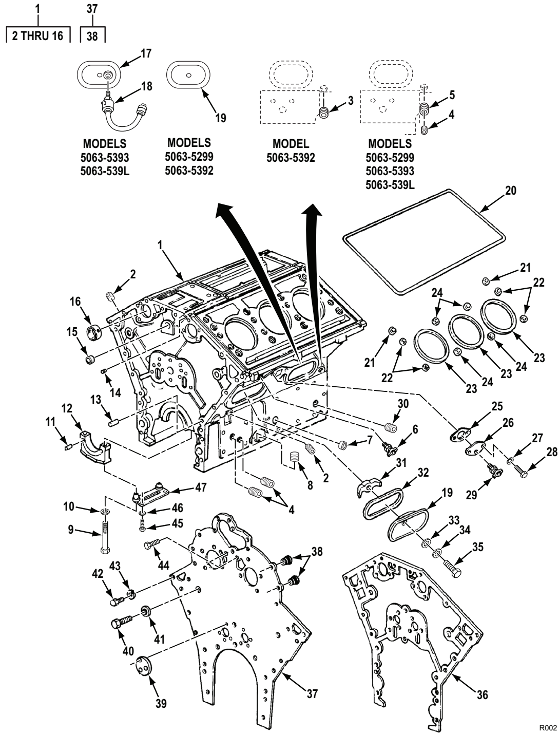
Figure 2. Cylinder Block Assembly, End Plate, and Related Parts.
