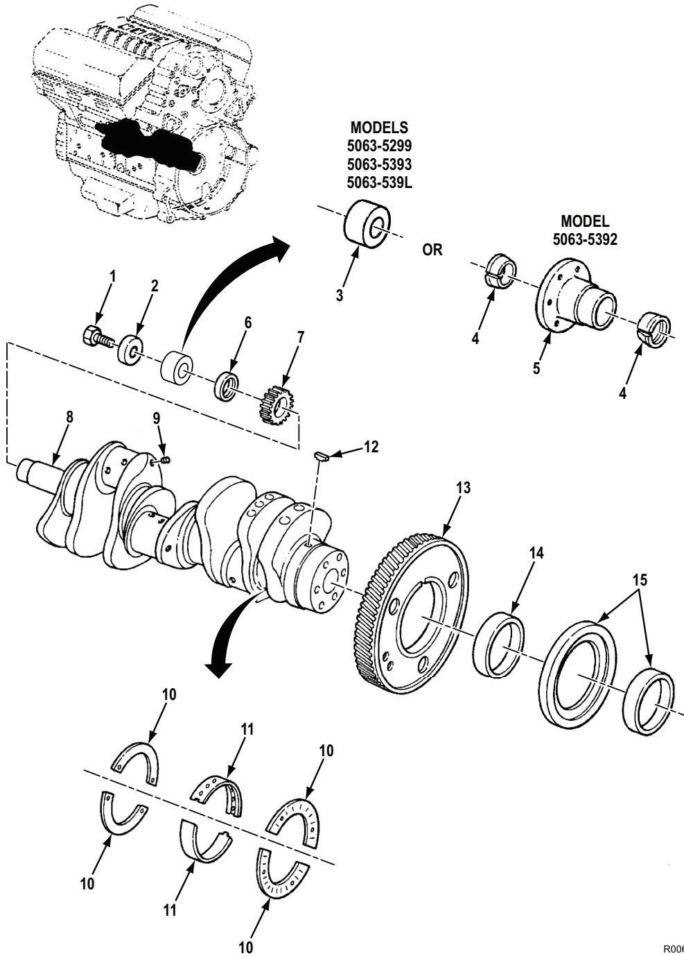
Figure 6. Crankshaft, Main Bearings, and Timing Gear.
