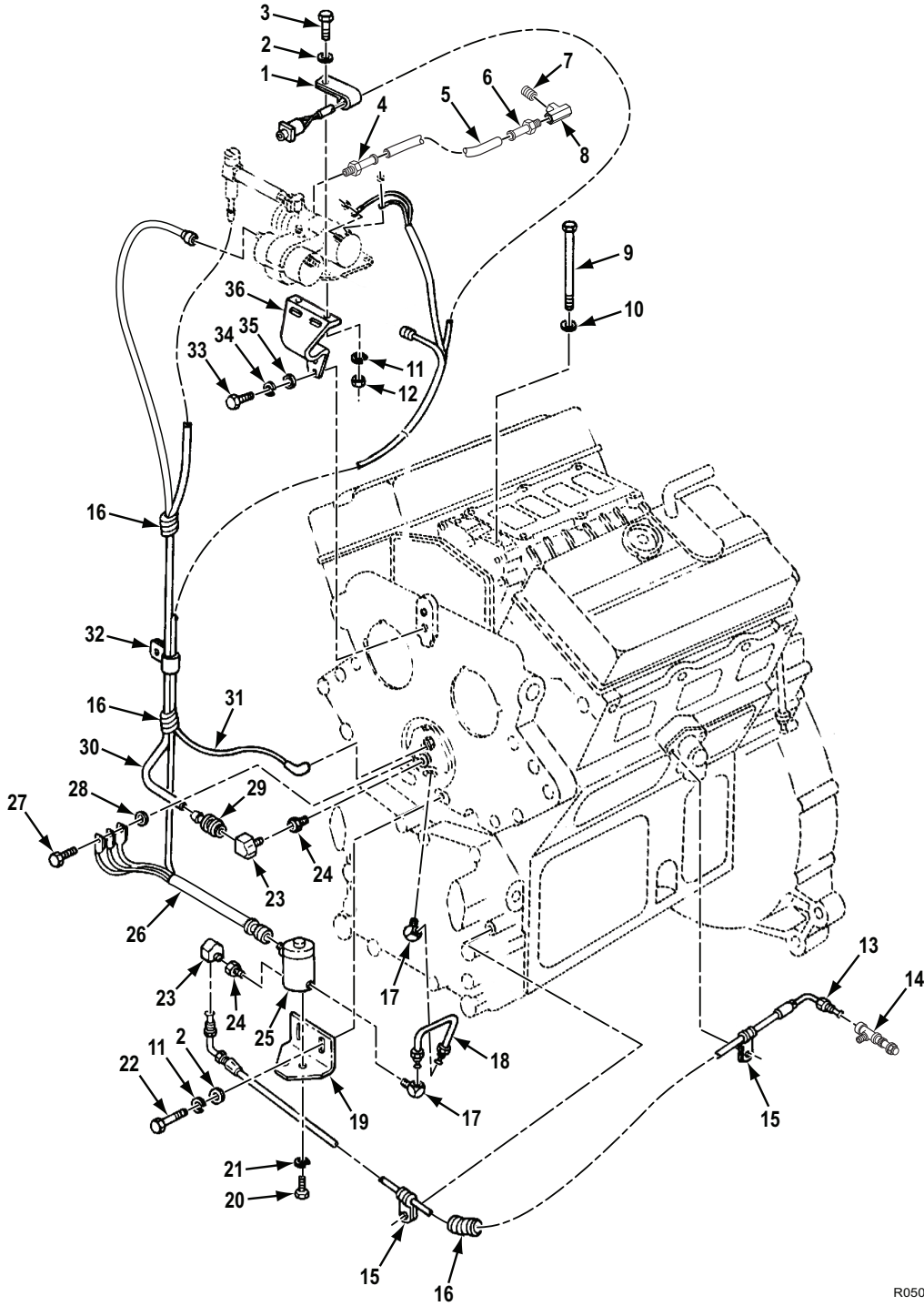
Figure 46. Air Box Heater and Related Parts (Models 5063-5299).
