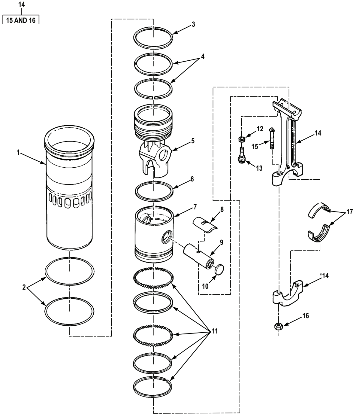
Figure 9. Pistons and Rod Assembly (Crosshead Type) With Liner.
