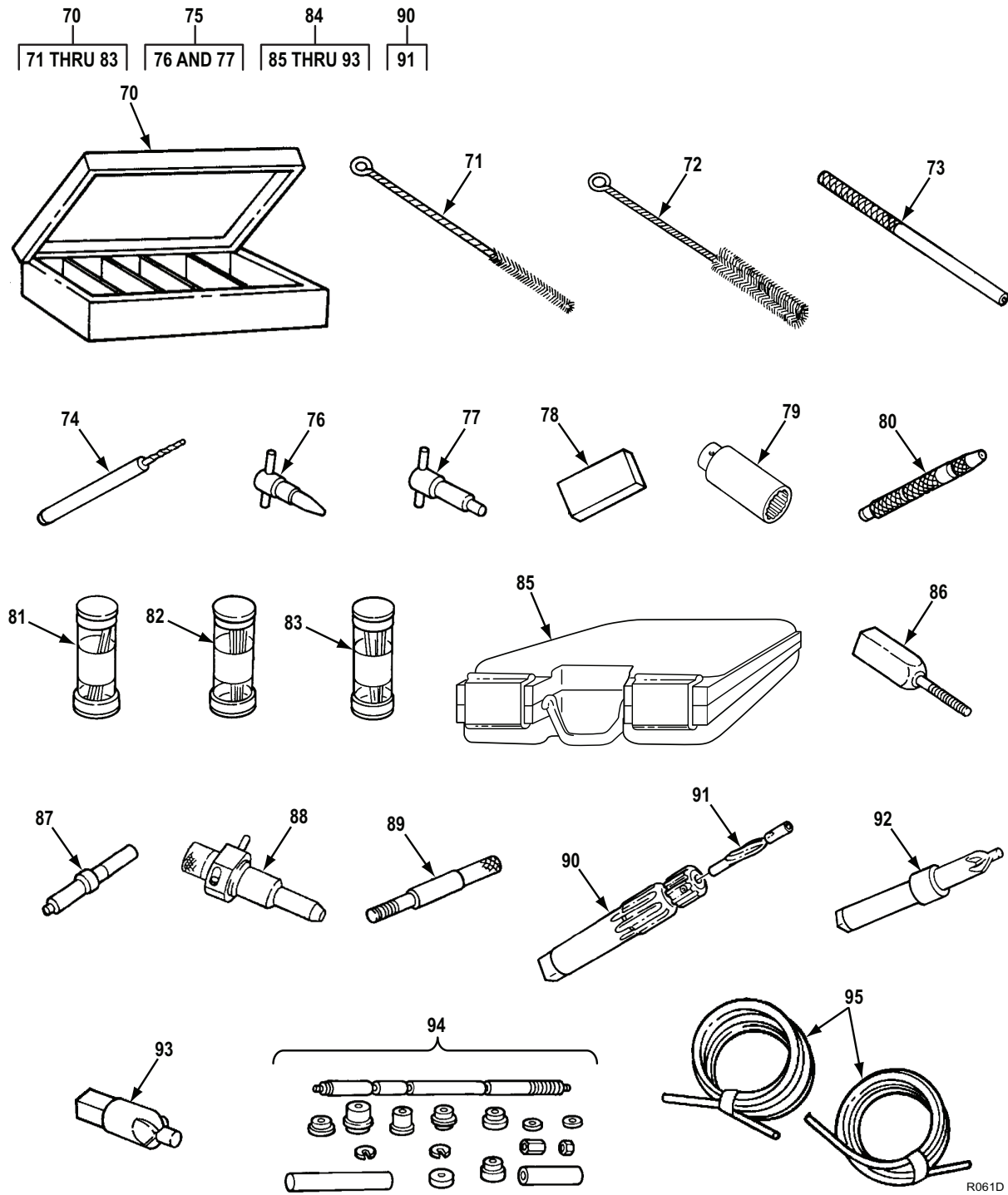
Figure 57. Special Tools For Sustainment Level Maintenance-Below Depot (SML-BD). (Sheet 5 of 5)
