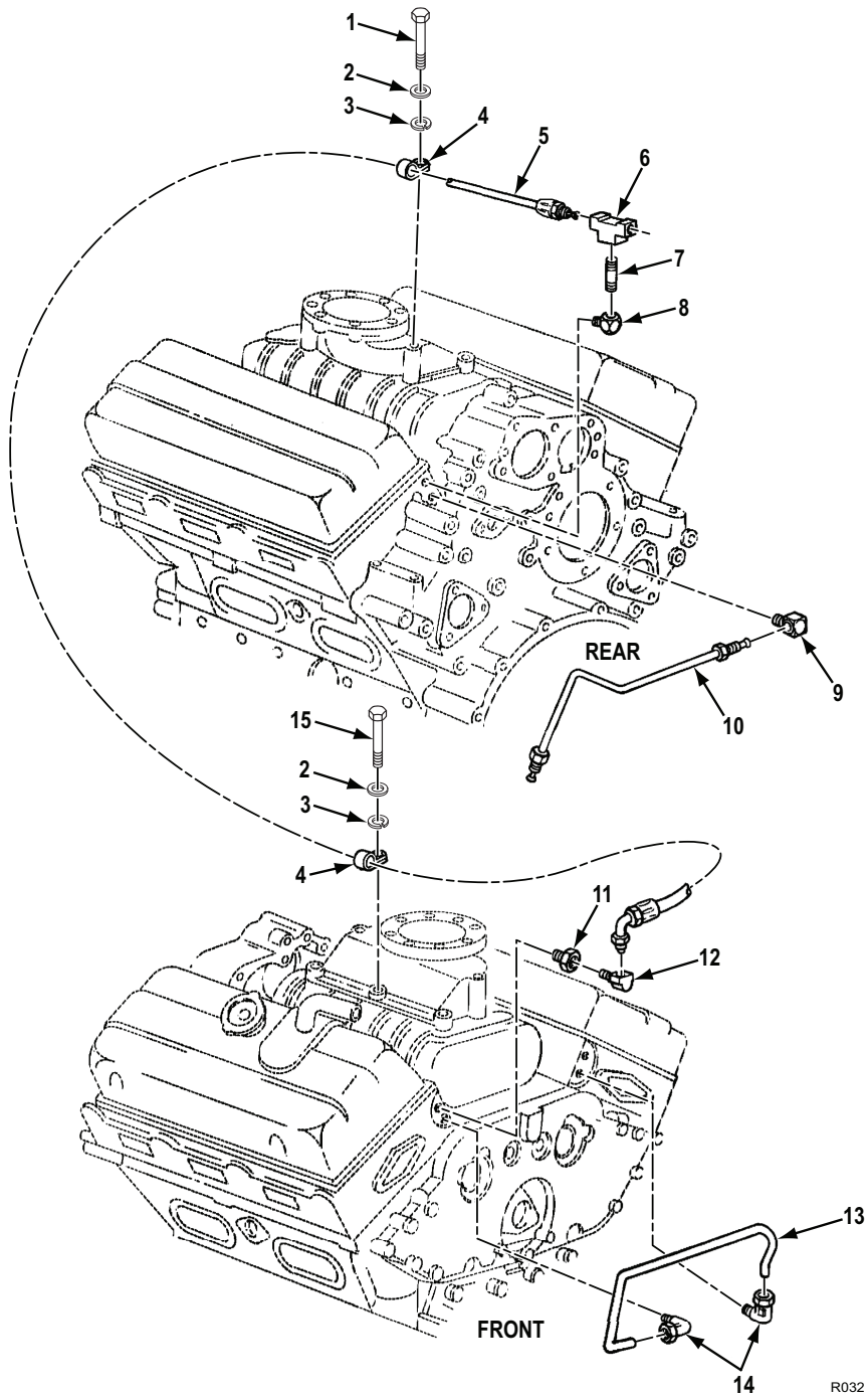
Figure 29. Fuel Lines and Fittings (Model 5063-5299).
