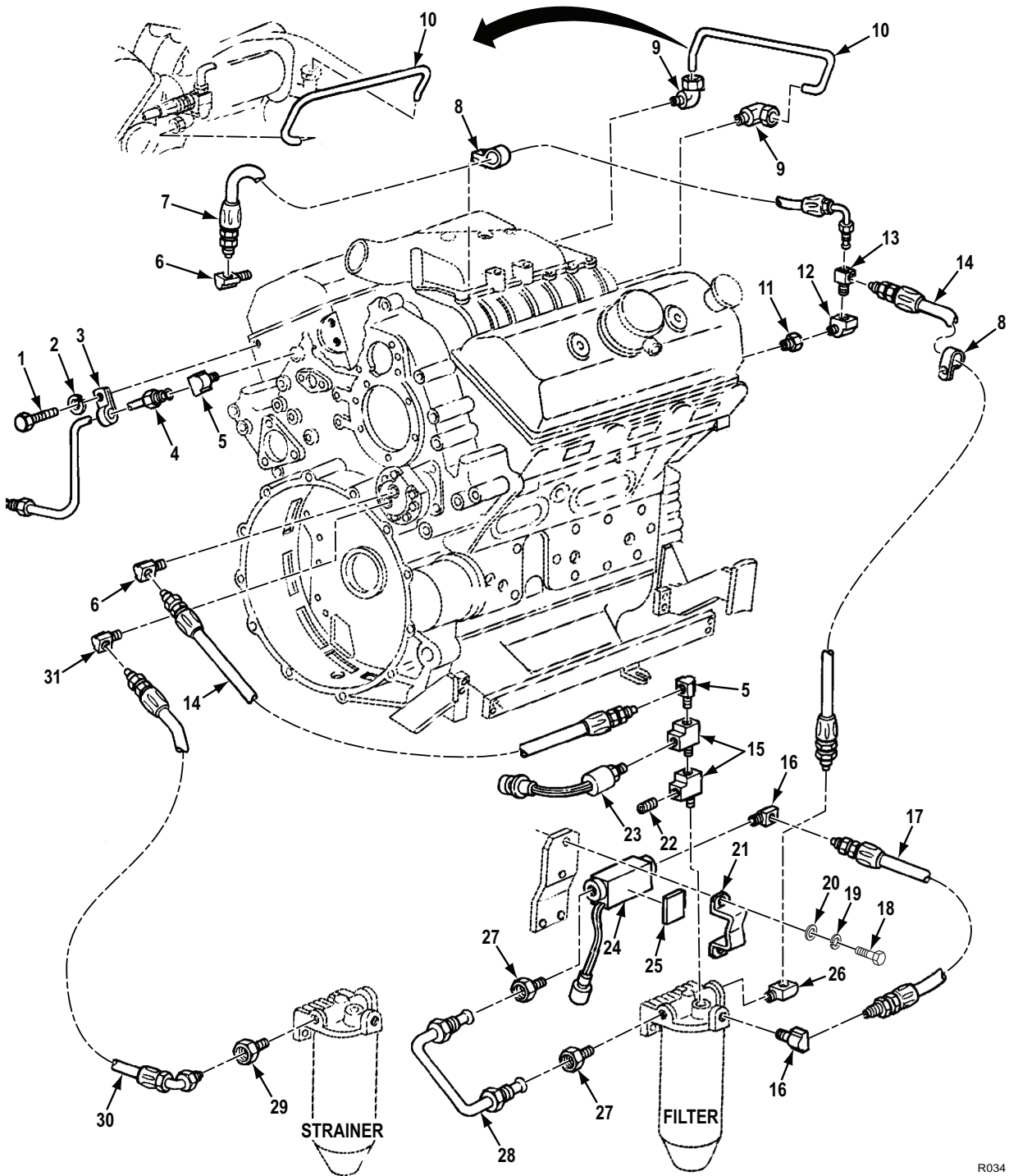
Figure 31. Fuel Lines and Fittings (Models 5063-5393 and 5063-539L).
