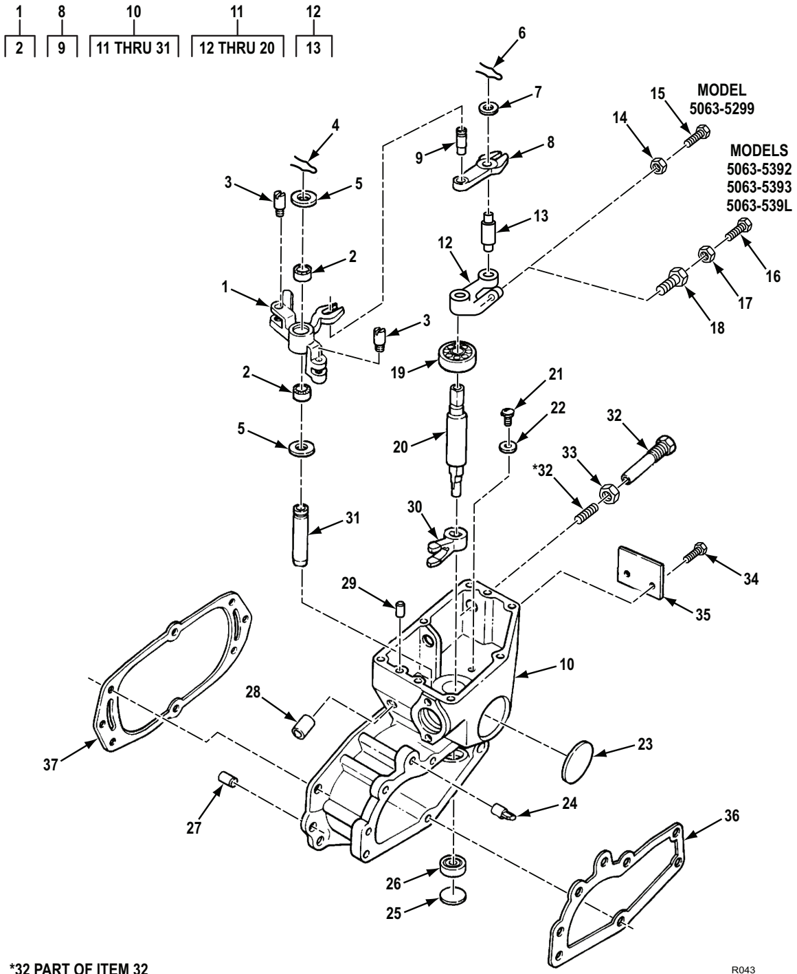
Figure 39. Governor Housing Assembly and Components.
