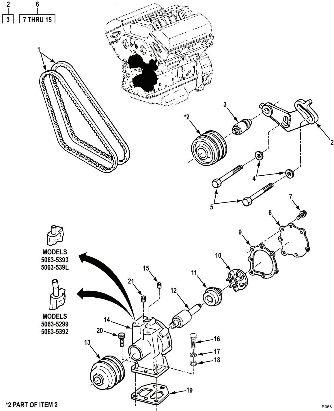
Figure 54. Coolant Pump Assembly, Idler Pulley, and Belt Set.
