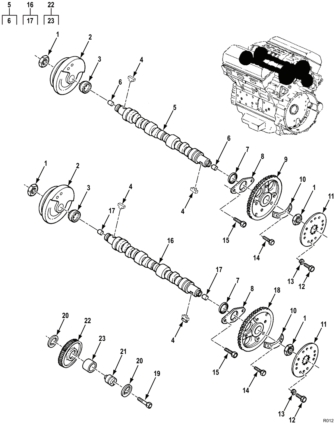
Figure 12. Camshafts, Idler Gear, and Balance Gear.
