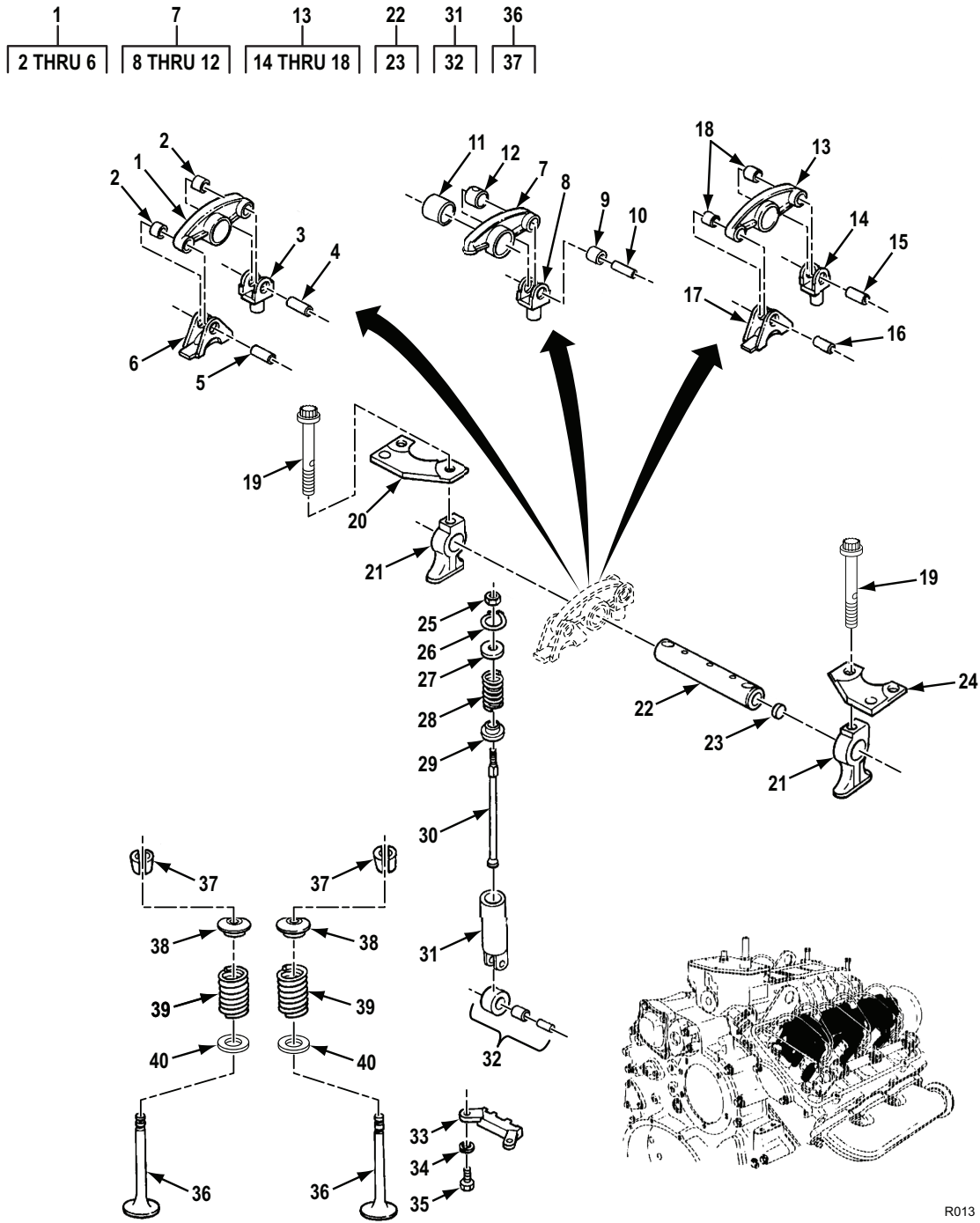
Figure 13. Rocker Arm Assemblies, Valves, and Cam Followers.
