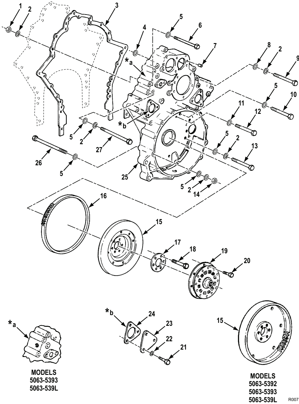
Figure 7. Drive Plate, Flywheel, and Housing.
