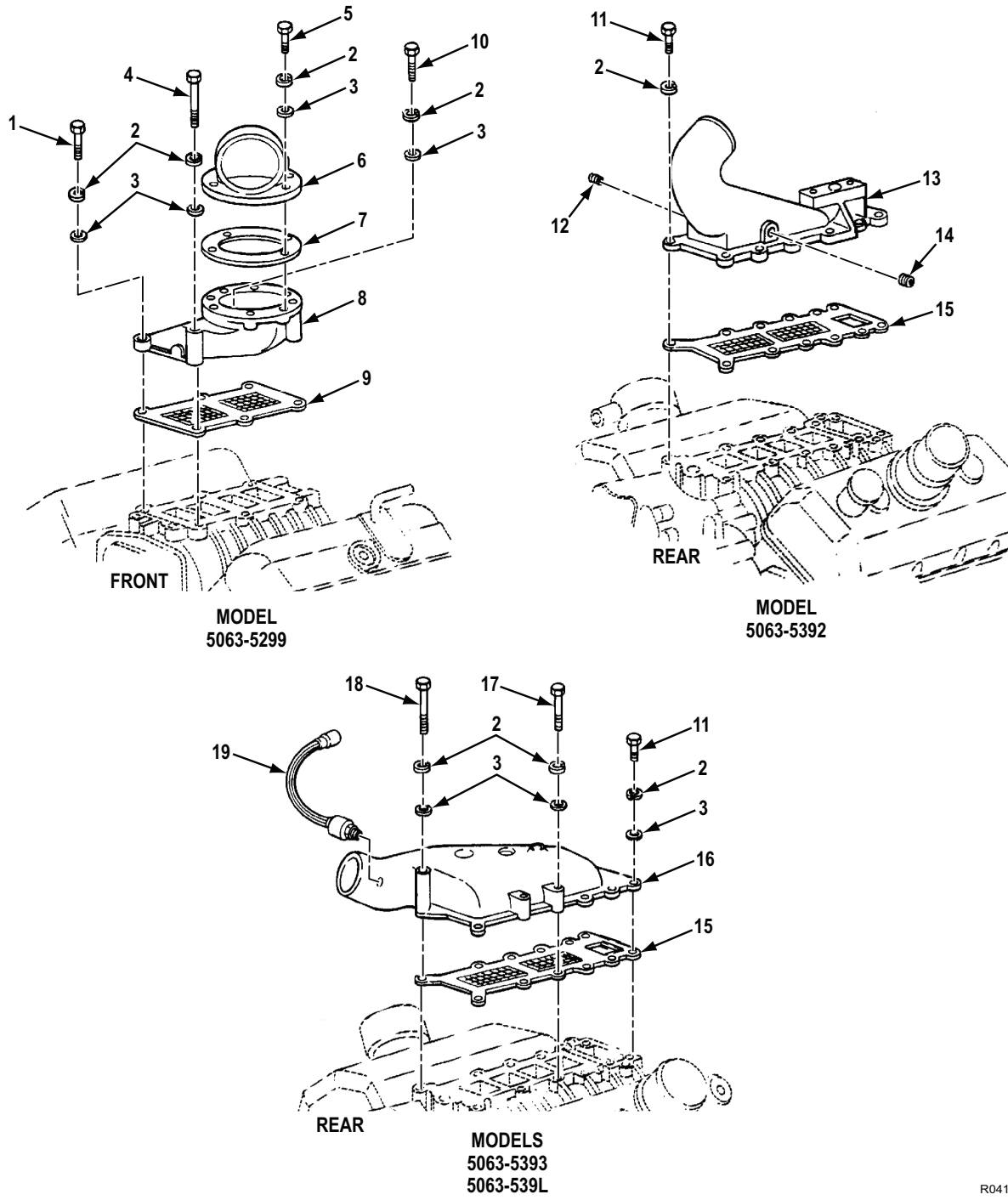
Figure 37. Air Inlet Housing and Related Parts.
