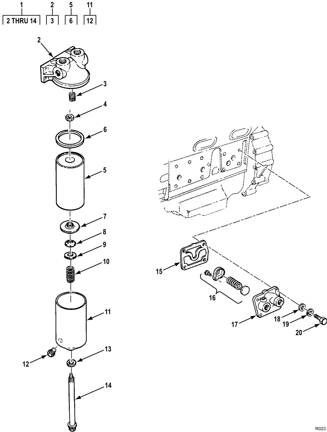
Figure 20. Oil Filter Assembly and Adapter (Model 5063-5299).
