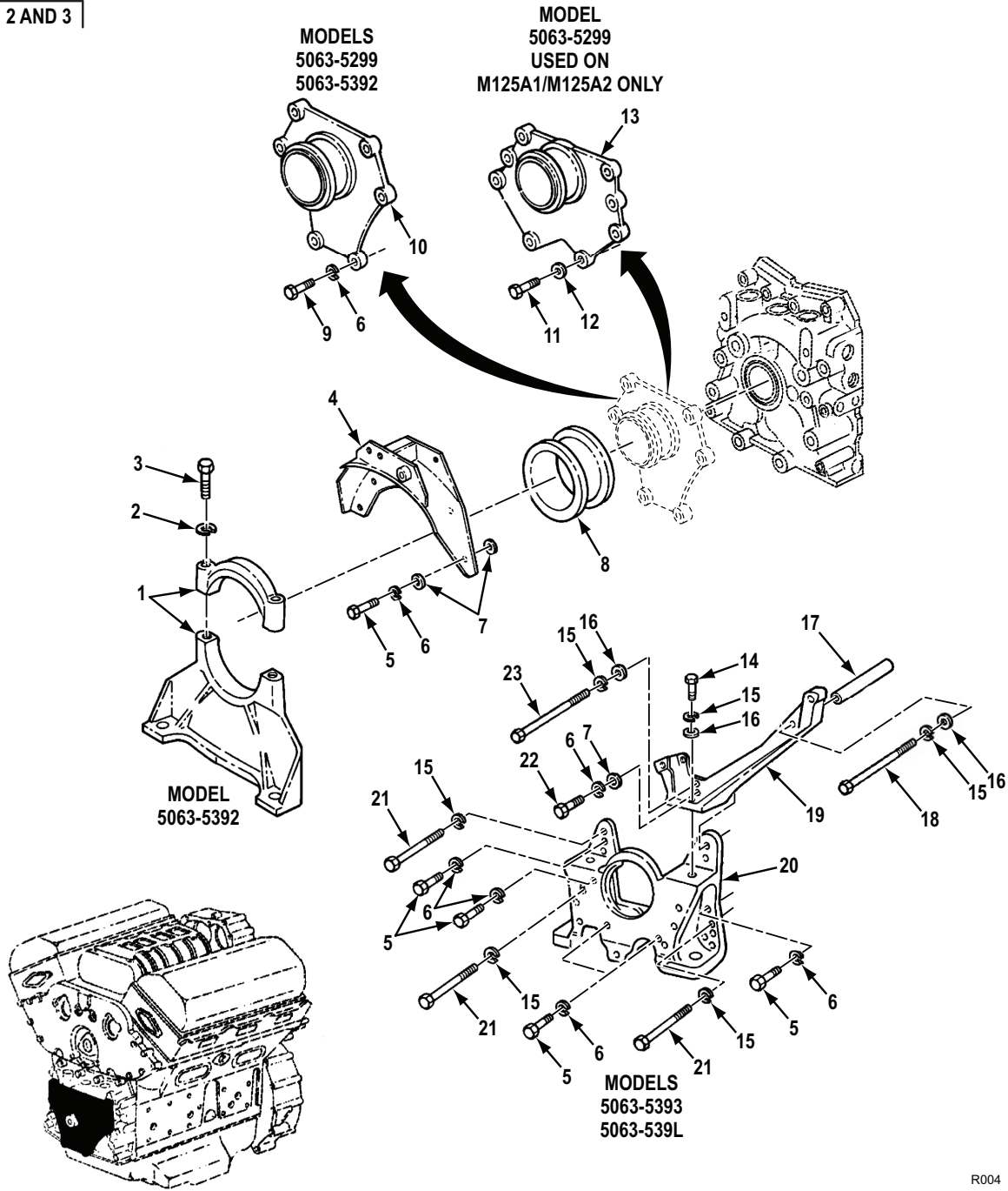
Figure 4. Engine Front Support (Trunnion).
