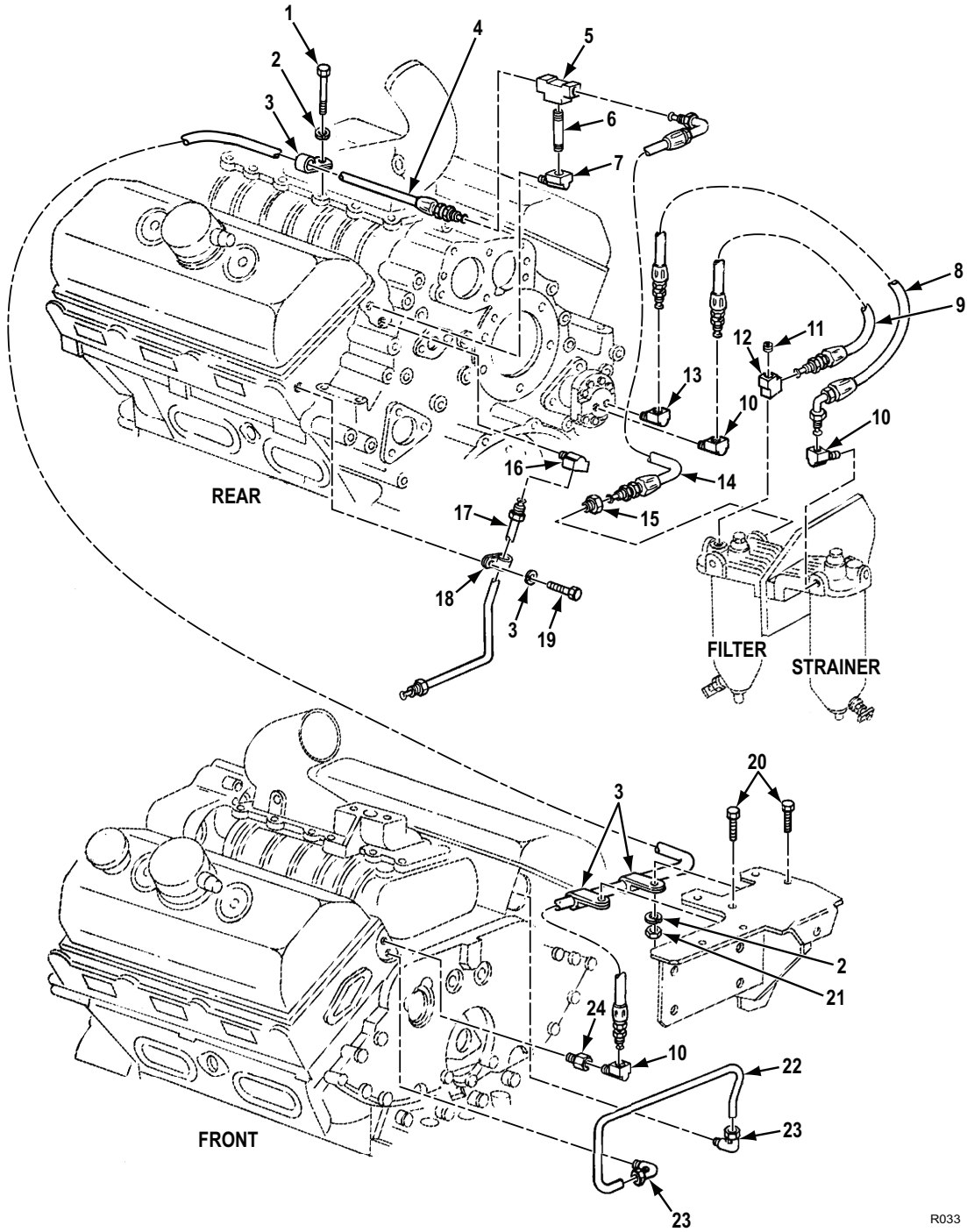
Figure 30. Fuel Lines and Fittings (Model 5063-5392).
