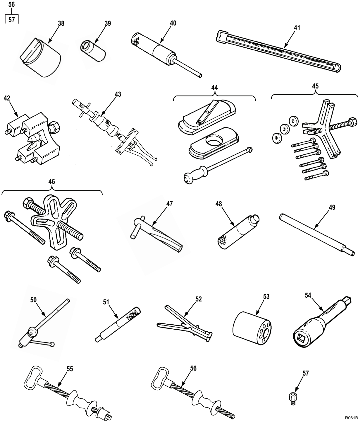
Figure 57. Special Tools For Sustainment Level Maintenance-Below Depot (SML-BD). (Sheet 3 of 5)
