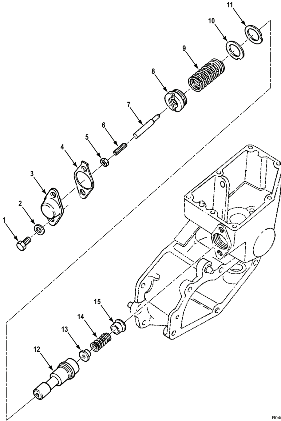
Figure 41. Governor High Speed Spring Pack and Related Parts.
