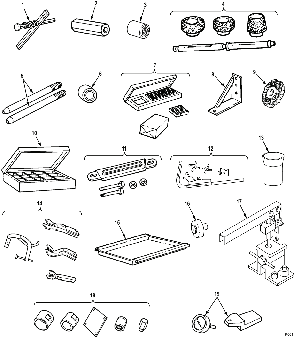
Figure 57. Special Tools For Sustainment Level Maintenance-Below Depot (SML-BD). (Sheet 1 of 5)
