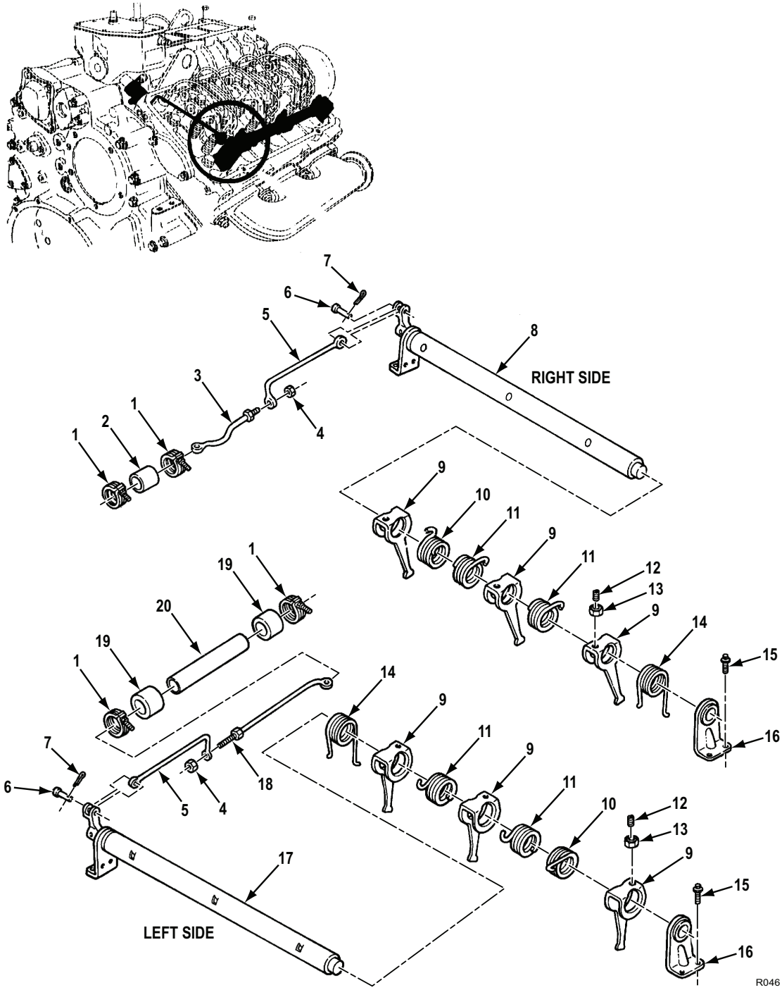
Figure 42. Fuel Injector Control Tubes and Linkage.
