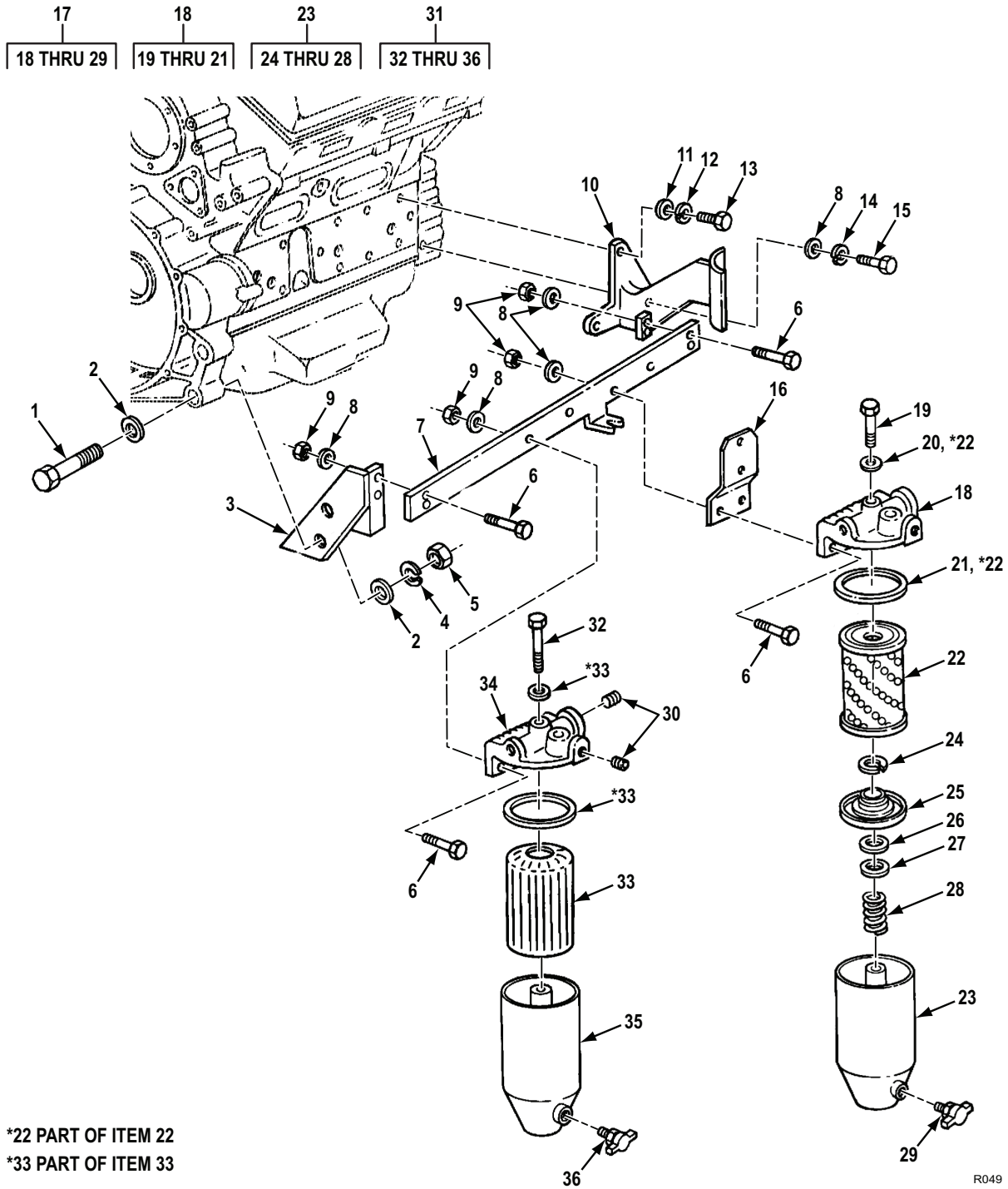
Figure 45. Fuel Filter and Strainer Assemblies (Models 5063-5393 and 5063-539L).
