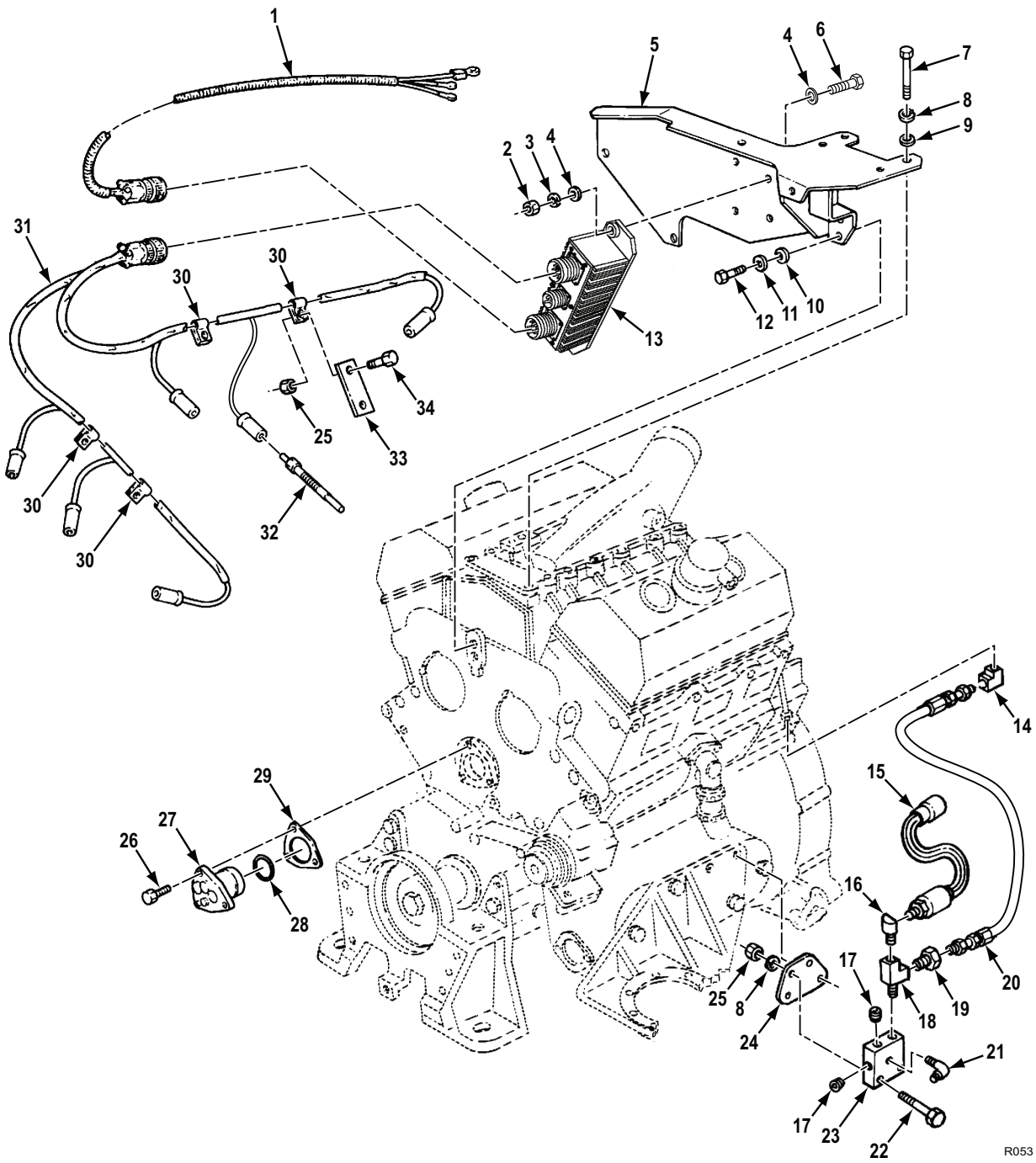
Figure 49. Glow Plug Controller and Related Parts (Model 5063-539L).
