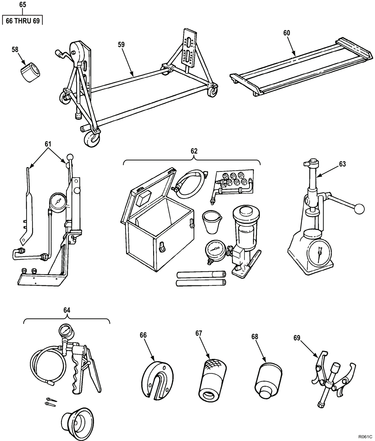
Figure 57. Special Tools For Sustainment Level Maintenance-Below Depot (SML-BD). (Sheet 4 of 5)
