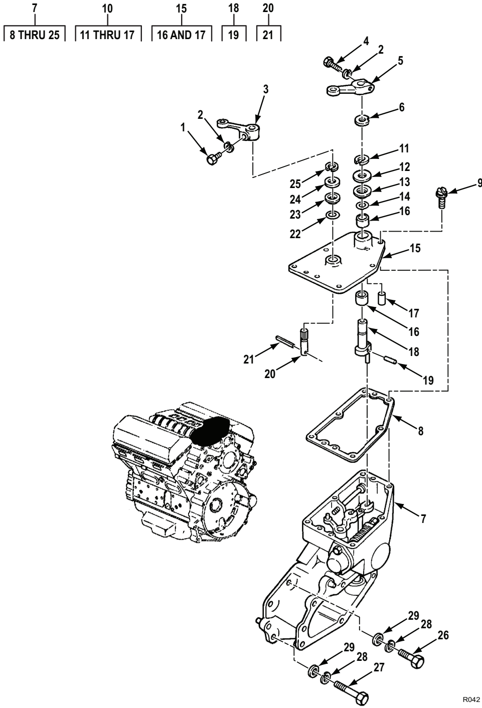
Figure 38. Governor and Cover Assembly.
