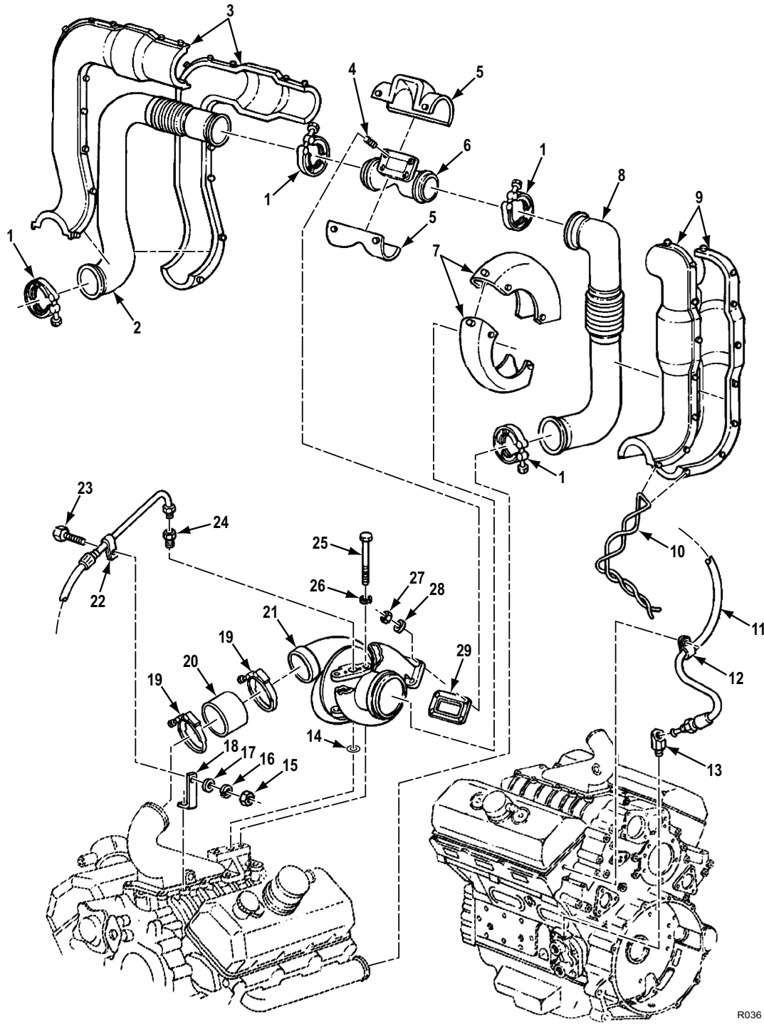
Figure 33. Turbocharger and Related Parts (Model 5063-5392).
