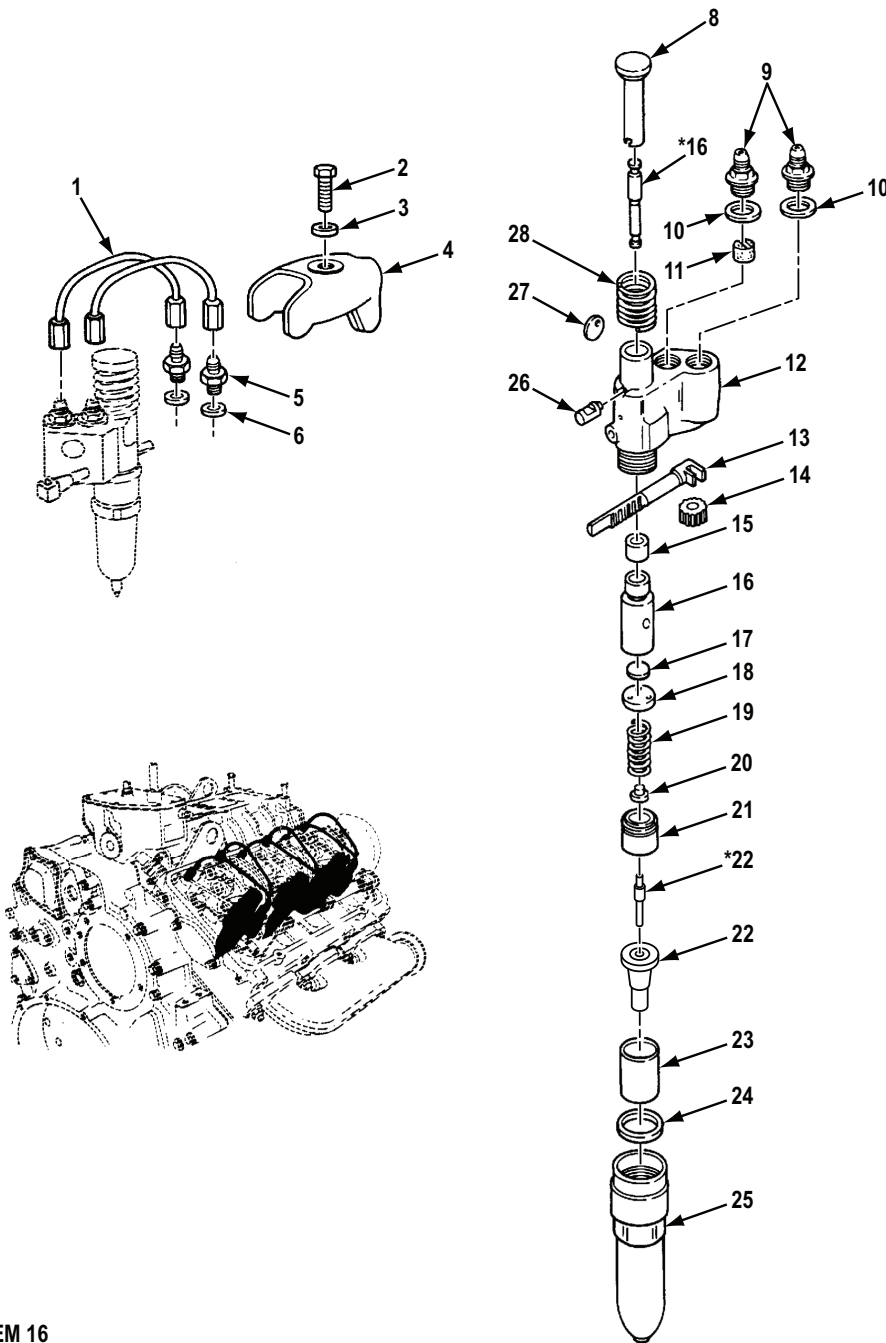
Figure 27. Fuel Injector and Related Parts.
