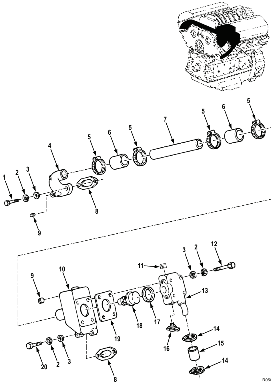
Figure 52. Thermostat, Housing, Lines, and Fittings (Models 5063-5299 and 5063-5392).
