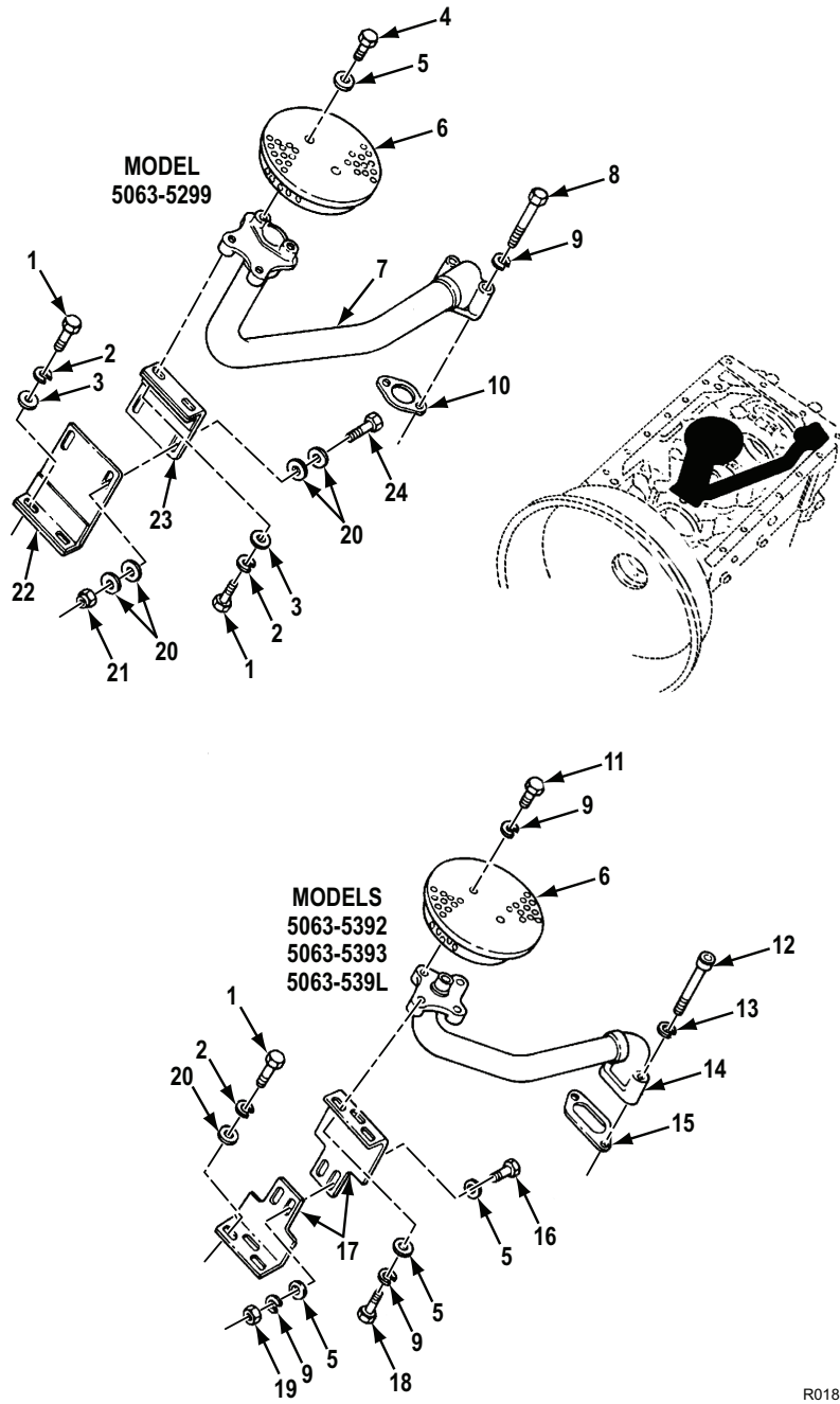
Figure 18. Oil Inlet Pipe, Screen, and Supports.
