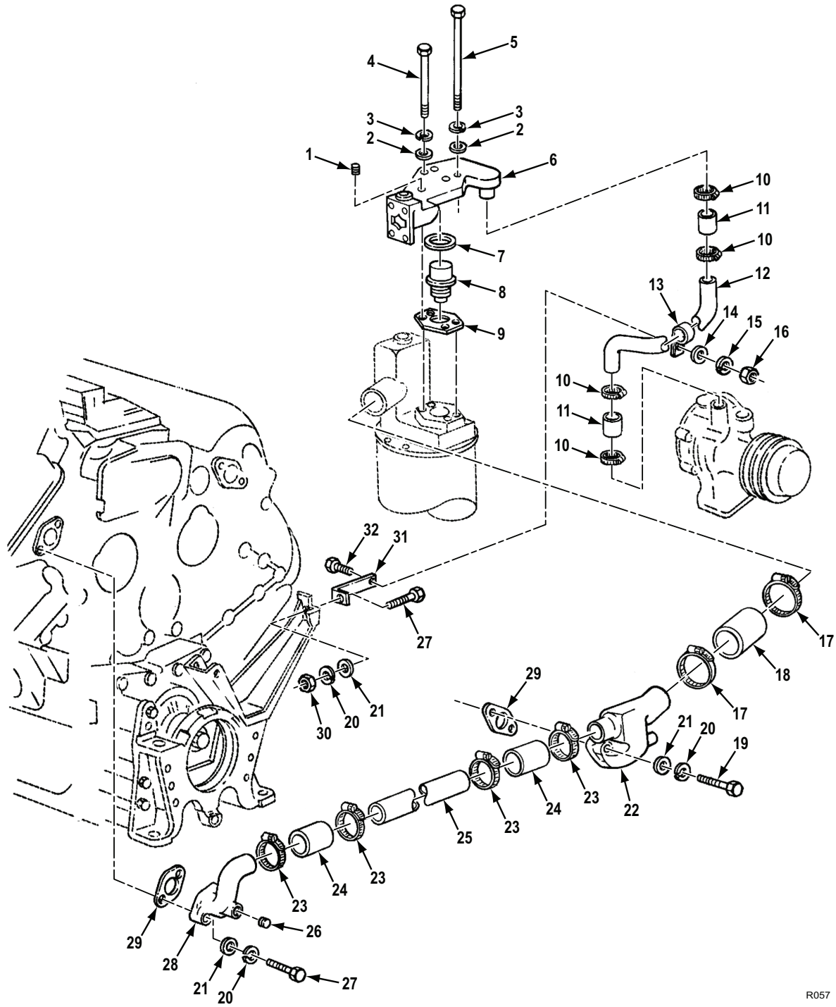
Figure 53. Thermostat, Housing, Lines, and Fittings (Models 5063-5393 and 5063-539L).
