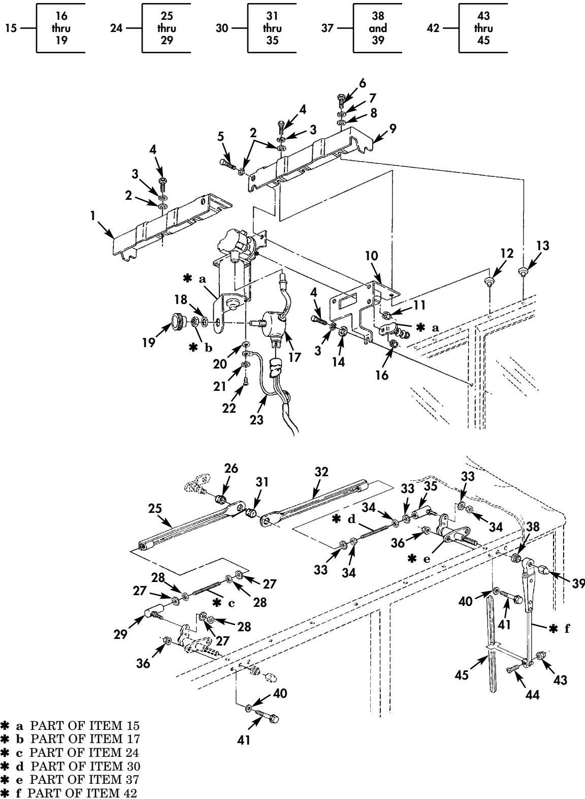
Figure 173. Windshield Wiper, Washer, and Related Parts (Sheet 1 of 3).
