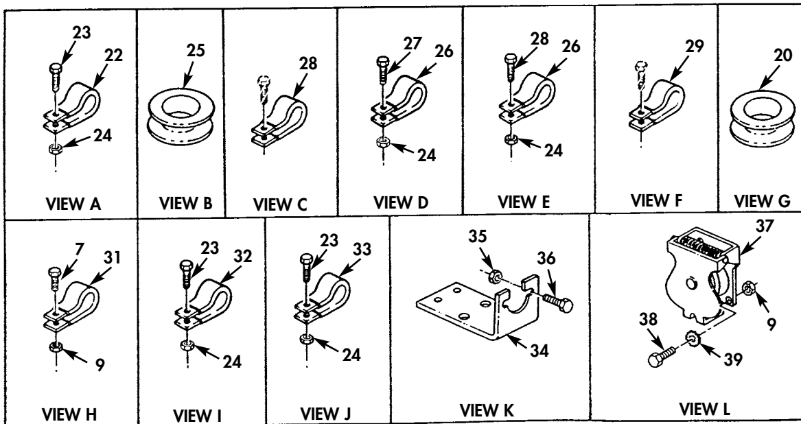
Figure 53. Rear Wiring Harness, Van, Tanker, and Cargo (Sheet 2 of 2).
