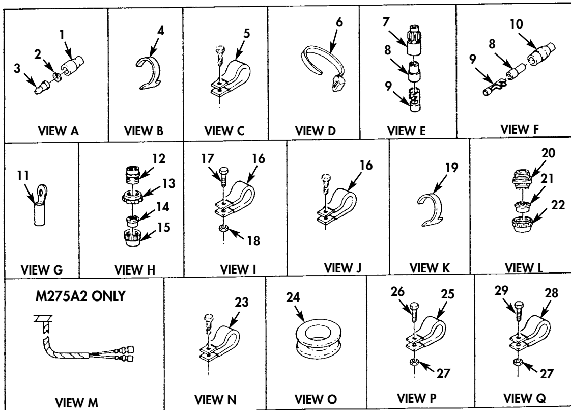
Figure 51. Front Wiring Harness Hardware.
