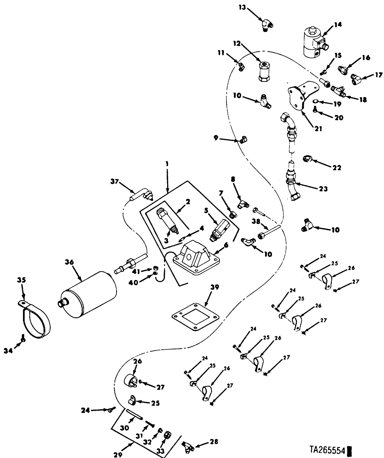
FIGURE 46. LEFT BANK MANIFOLD HEATER ASSEMBLY AND RELATED PARTS.
