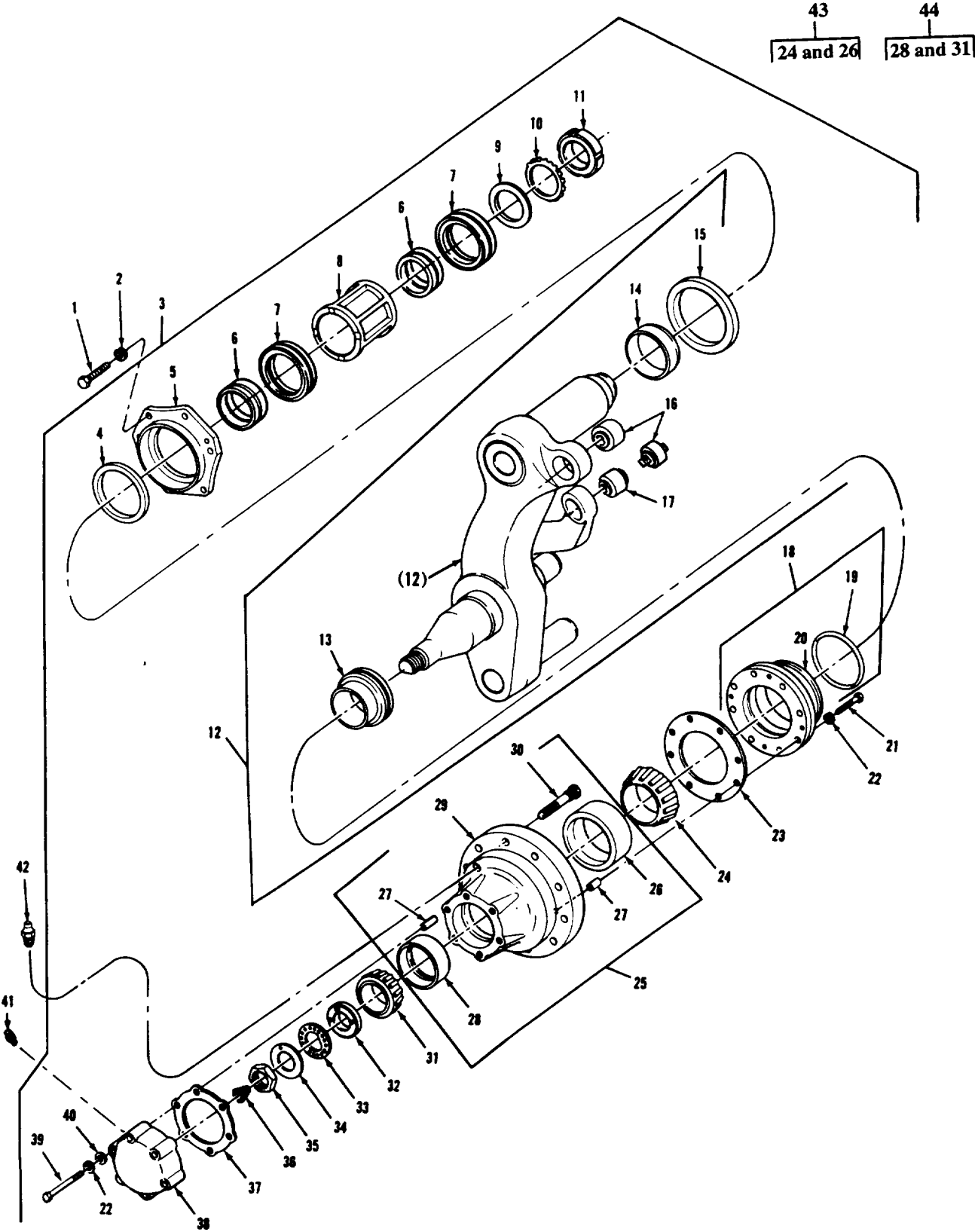
FIGURE 144. NO. 1 LEFT AND RIGHT HUB AND ARM ASSEMBLIES AND RELATED PARTS.
