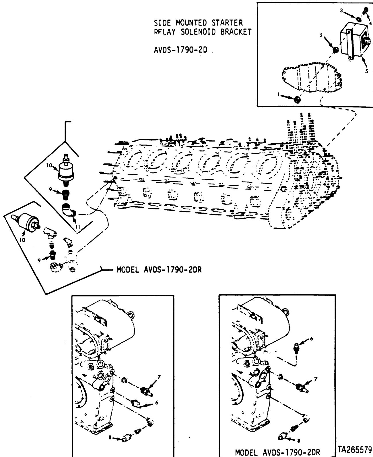
FIGURE 92. STARTER MODULE, OIL PRESSURE AND TEMPERATURE SWITCHES, TRANSMITTERS AND RELATED PARTS.
