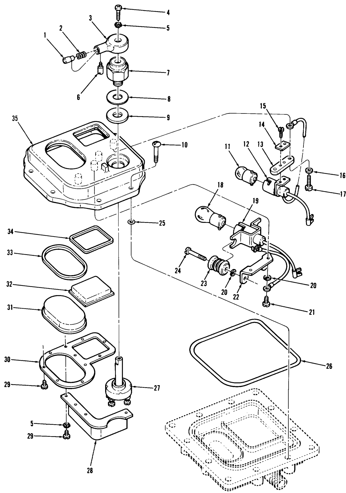
FIGURE 87. DRIVER'S DOME LIGHT COMPONENTS (ASSY P/N 7064671).
