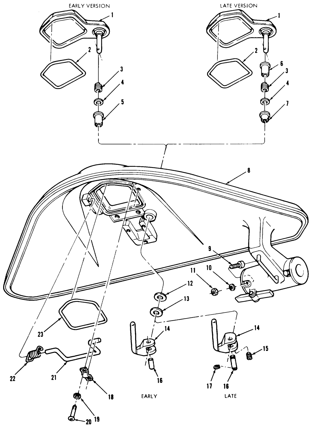
FIGURE 174. DRIVER'S HATCH COVER COMPONENTS, PASSIVE EQUIPPED VEHICLES (ASSY P/N 12252115, FIG. 1 OF 2) DOORS AND RELATED PARTS.
