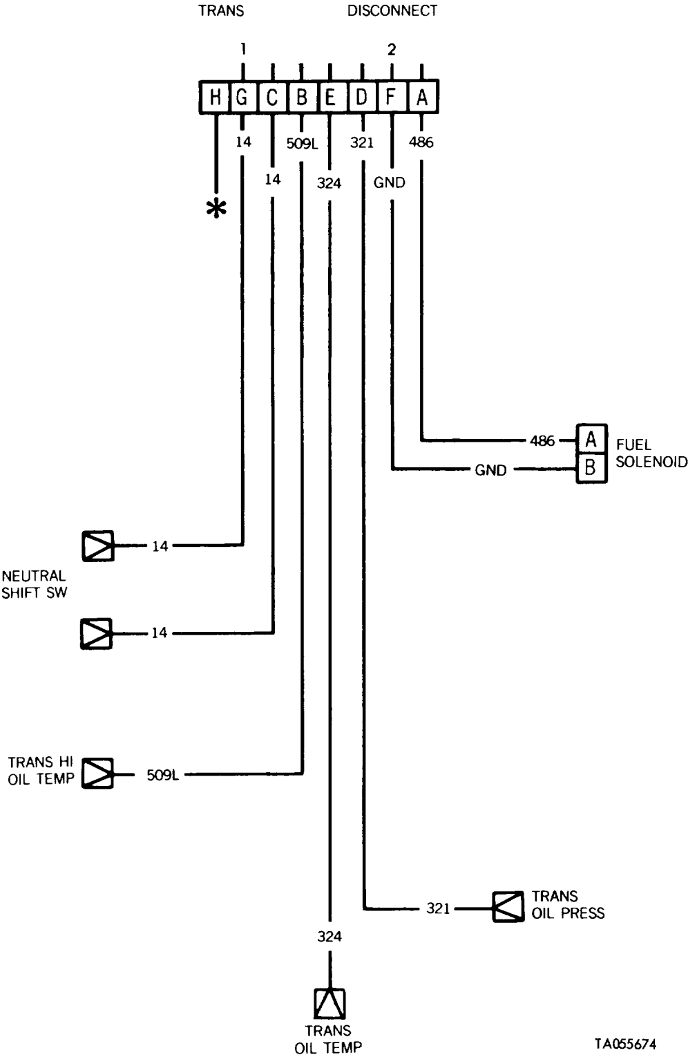
FIGURE 119. TRANSMISSION WIRING HARNESS.
