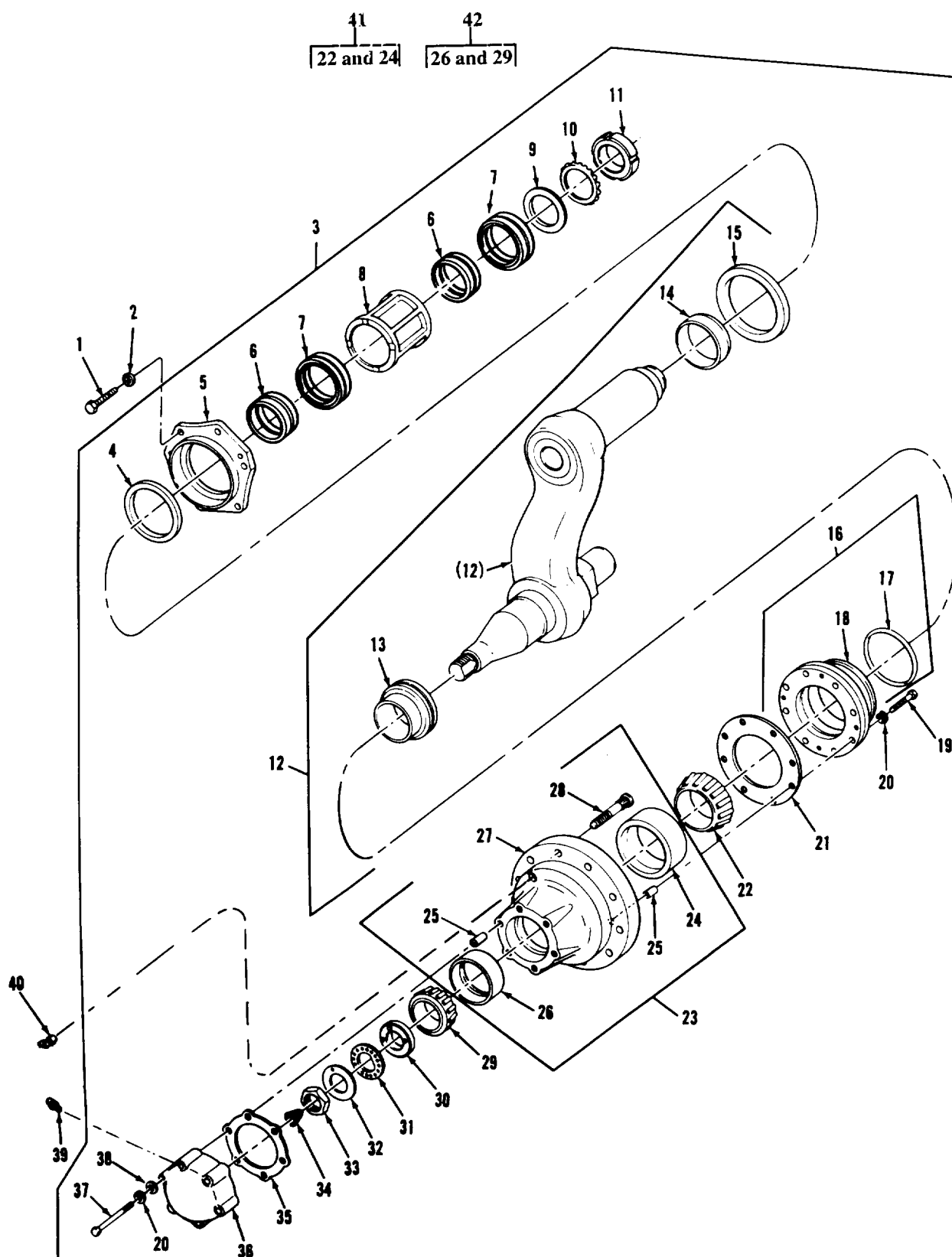
FIGURE 146. NO. 3 AND NO. 5 LEFT AND RIGHT HUB AND ARM ASSEMBLIES AND RELATED PARTS.
