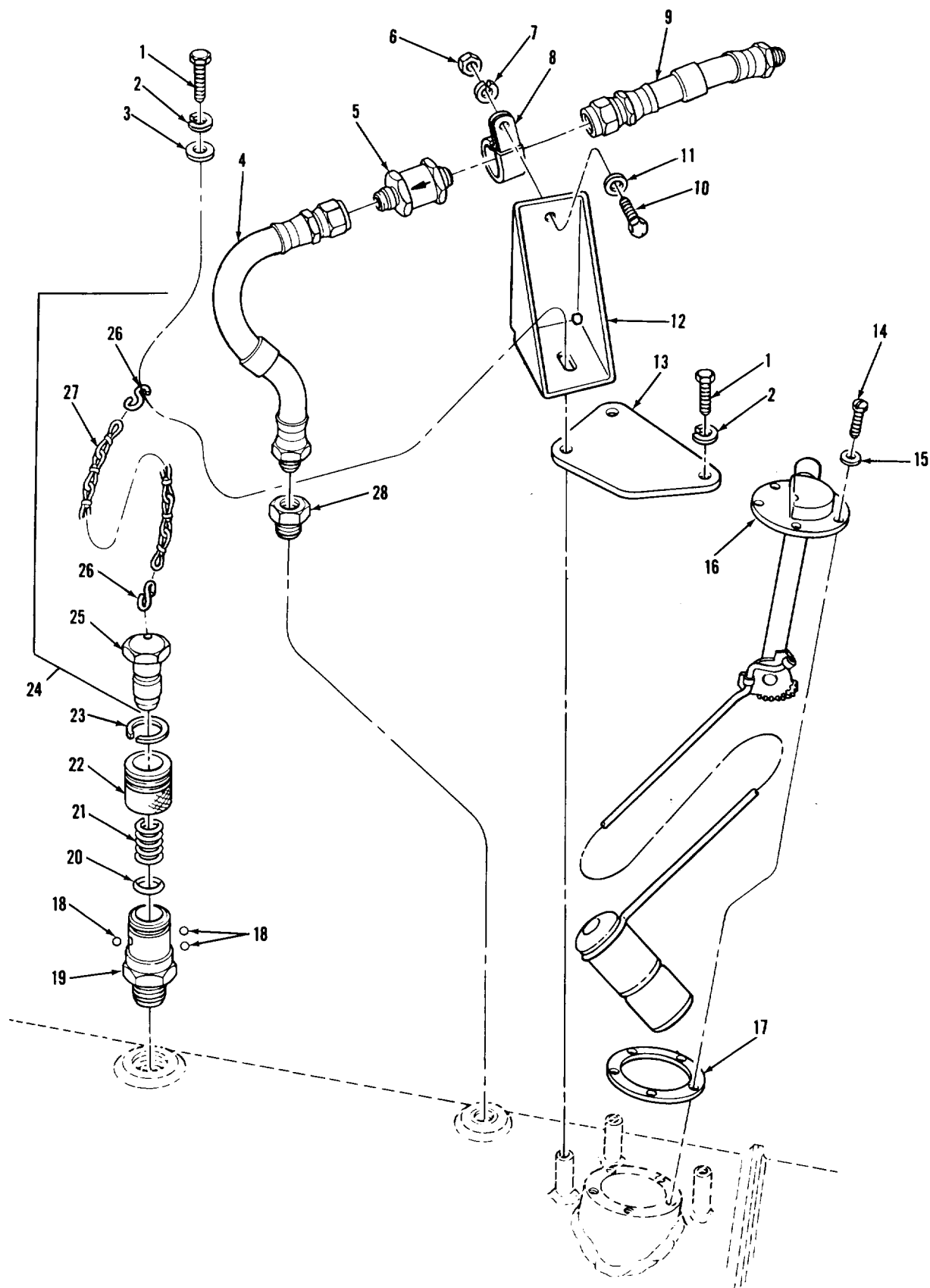
FIGURE 32. RIGHT FUEL TANK LIQUID QUANTITY TRANSMITTER AND RELATED PARTS.
