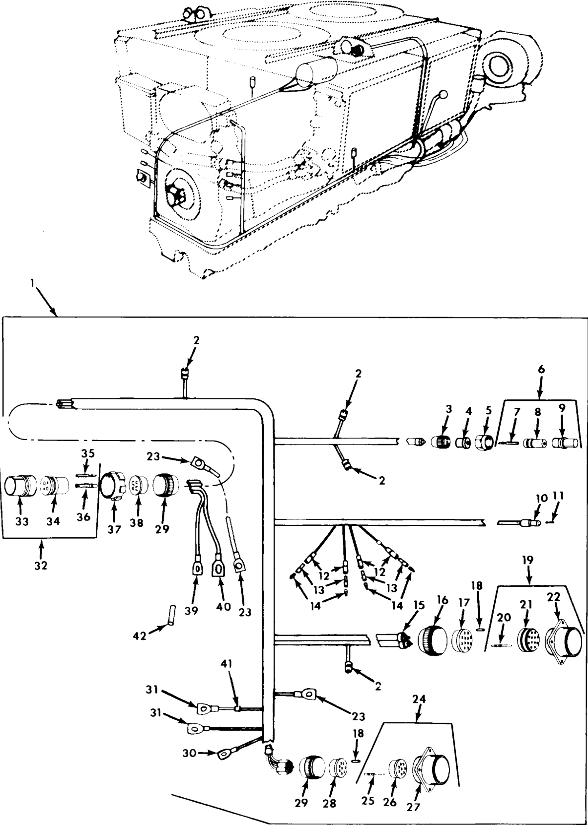
FIGURE 98. ENGINE WIRING HARNESS.
