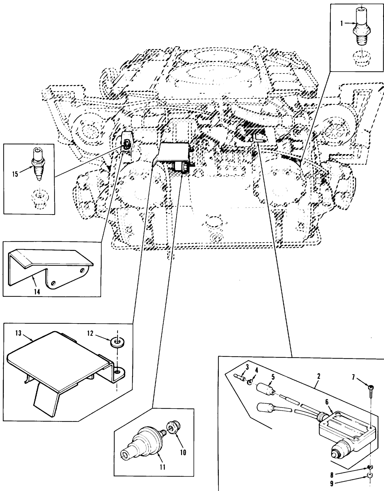
FIGURE 93. TRANSMISSION ELECTRICAL SYSTEM COMPONENTS (ASSY P/N 12270153).
