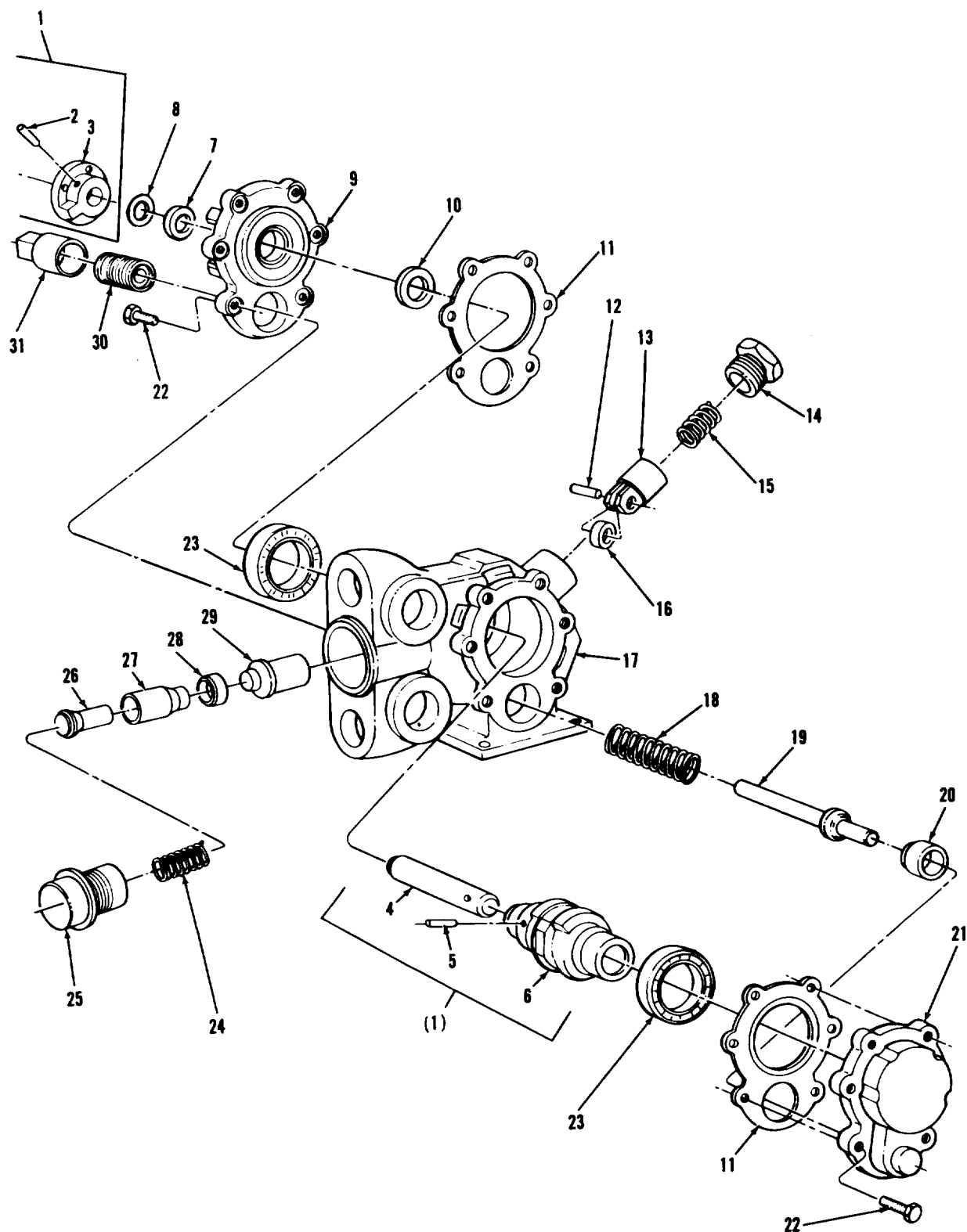
FIGURE 204. BULLDOZER SELECTOR HYDRAULIC PUMP CONTROL VALVE ASSEMBLY COMPONENTS (ASSY P/N 7323406).
