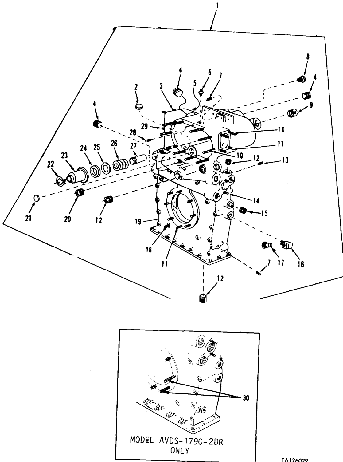
FIGURE 3. CRANKSHAFT DAMPER OIL FILTER HOUSING COMPONENTS (ASSY P/N 11684077 AND 11684077-1, FIG. 1 OF 3, OIL FILTER ELEMENT RETAINER, MOUNTING STUDS, AND RELATED PARTS
