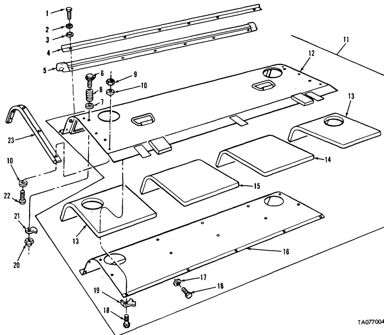
FIGURE 52. TRANSMISSION SHROUD ASSEMBLY, COMPONENTS, AND RELATED PARTS
