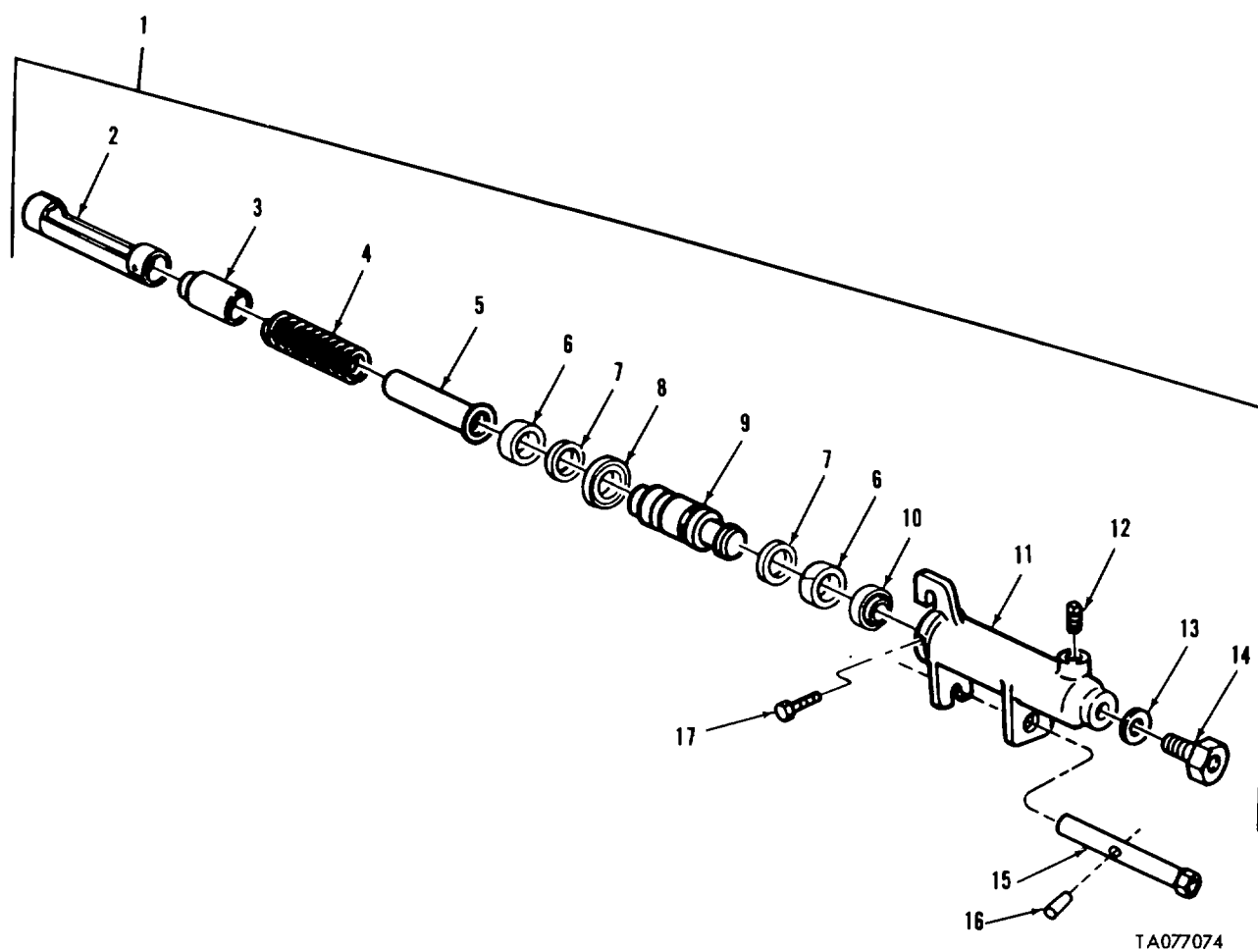
FIGURE 131. SLAVE TUBE CYLINDER ASSEMBLY AND COMPONENTS
