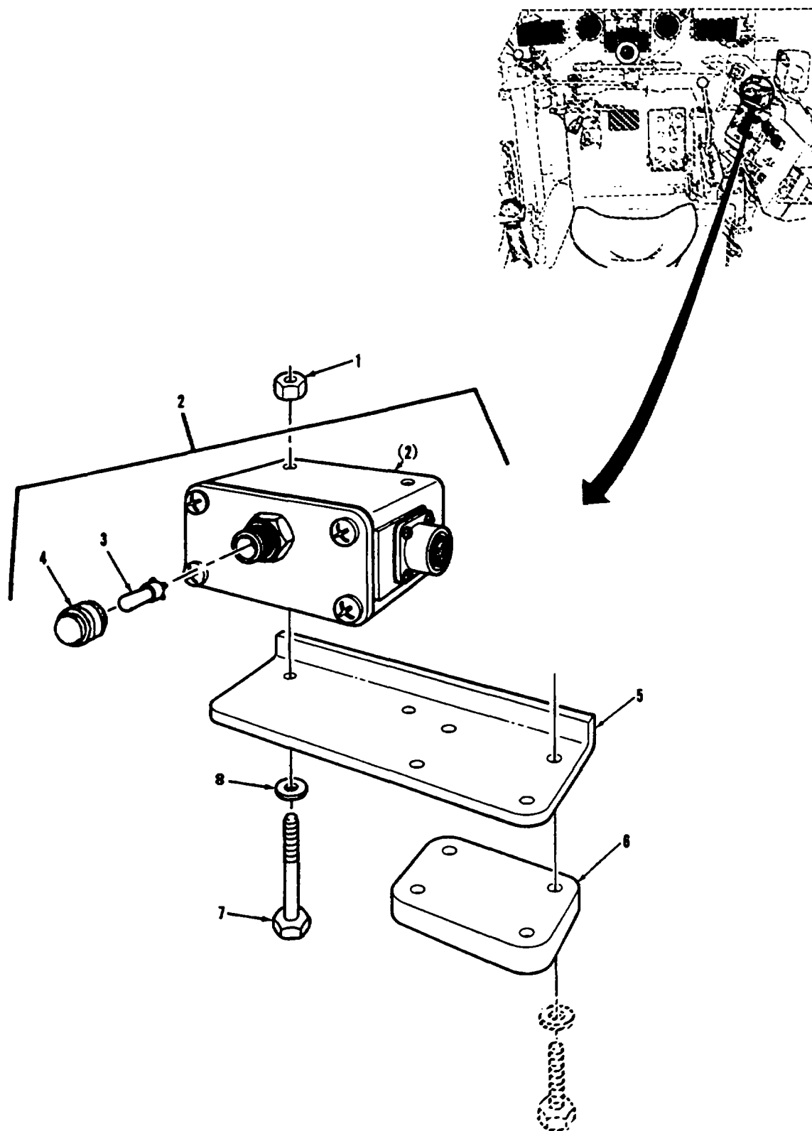
FIGURE 76. ENGINE DUST DETECTOR BOX ASSEMBLY, COMPONENTS, AND RELATED PARTS
