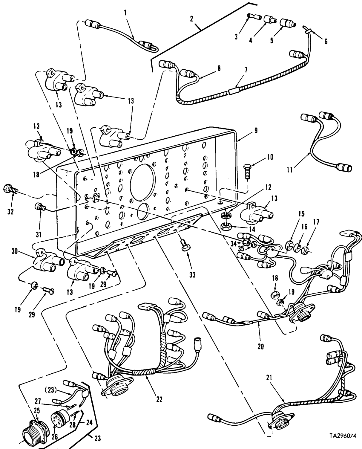
FIGURE 63. MASTER CONTROL PANEL ASSEMBLY COMPONENTS (ASSY P/N 12251969, FIG 2 OF 2, WIRING HARNESSSES, CIRCUIT BREAKERS AND RELATED PARTS)
