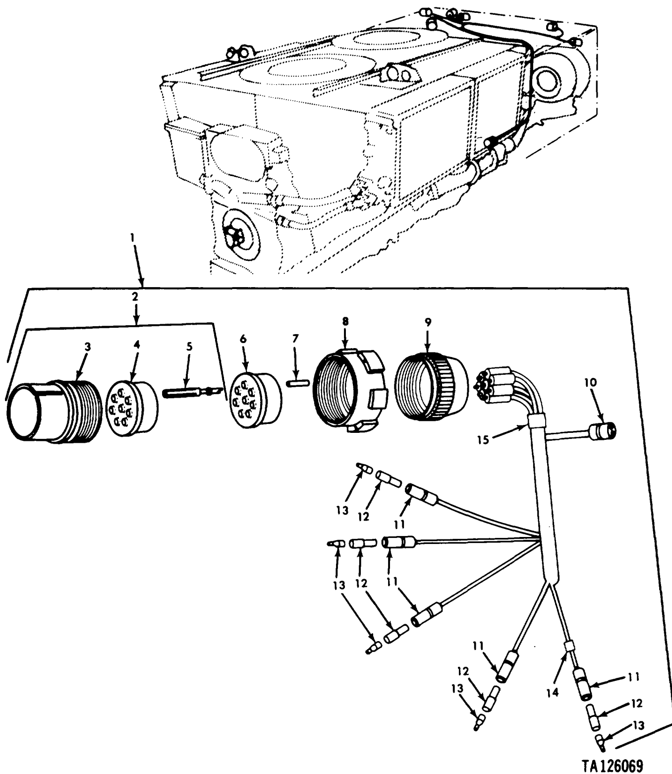
FIGURE 108. TRANSMISSION WIRING HARNESS AND COMPONENTS
