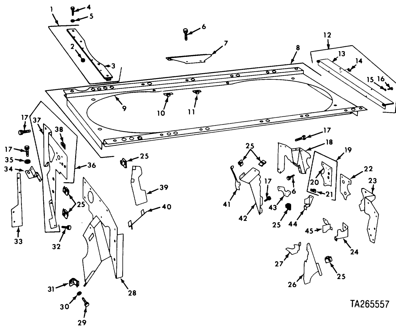
FIGURE 48. ENGINE SHROUDS AND RELATED PARTS
