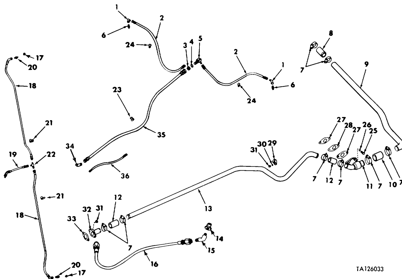
FIGURE 9. BREATHER TUBES, OIL SUPPLY HOSES, OIL COOLER VENT HOSES, AND RELATED PARTS
