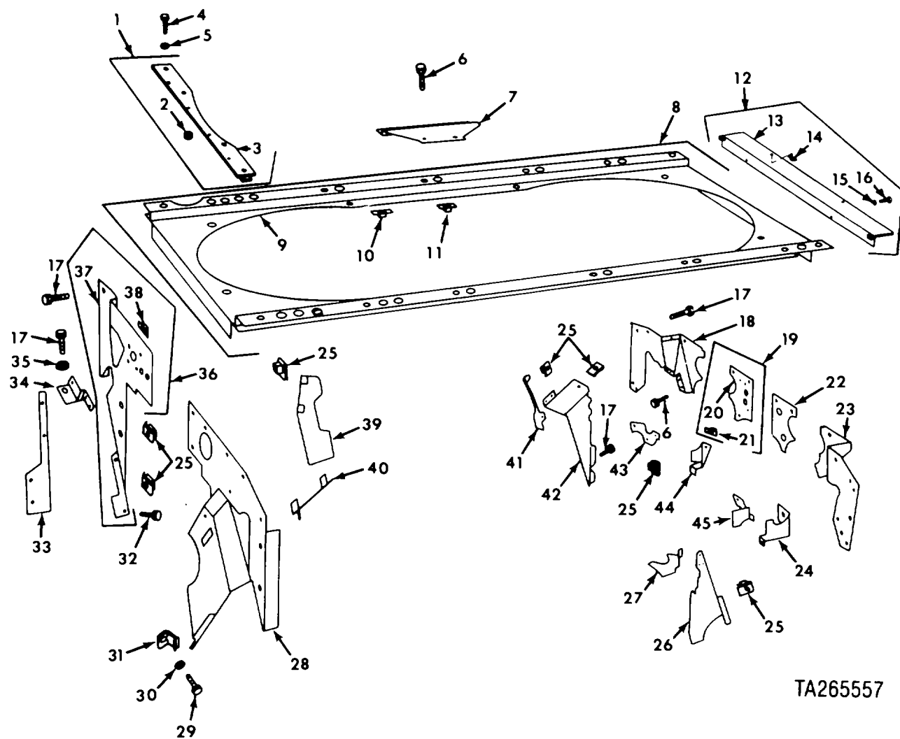
FIGURE 51. ENGINE SHROUD MOUNTING AND RELATED PARTS
