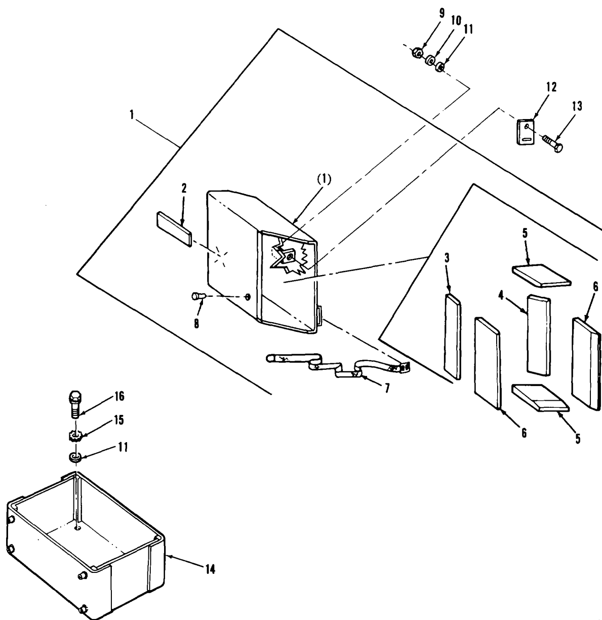
FIGURE 179. DRIVER'S PERISCOPE BOX ASSEMBLY, COMPONENTS, ODDMENT BOX, AND RELATED PARTS
