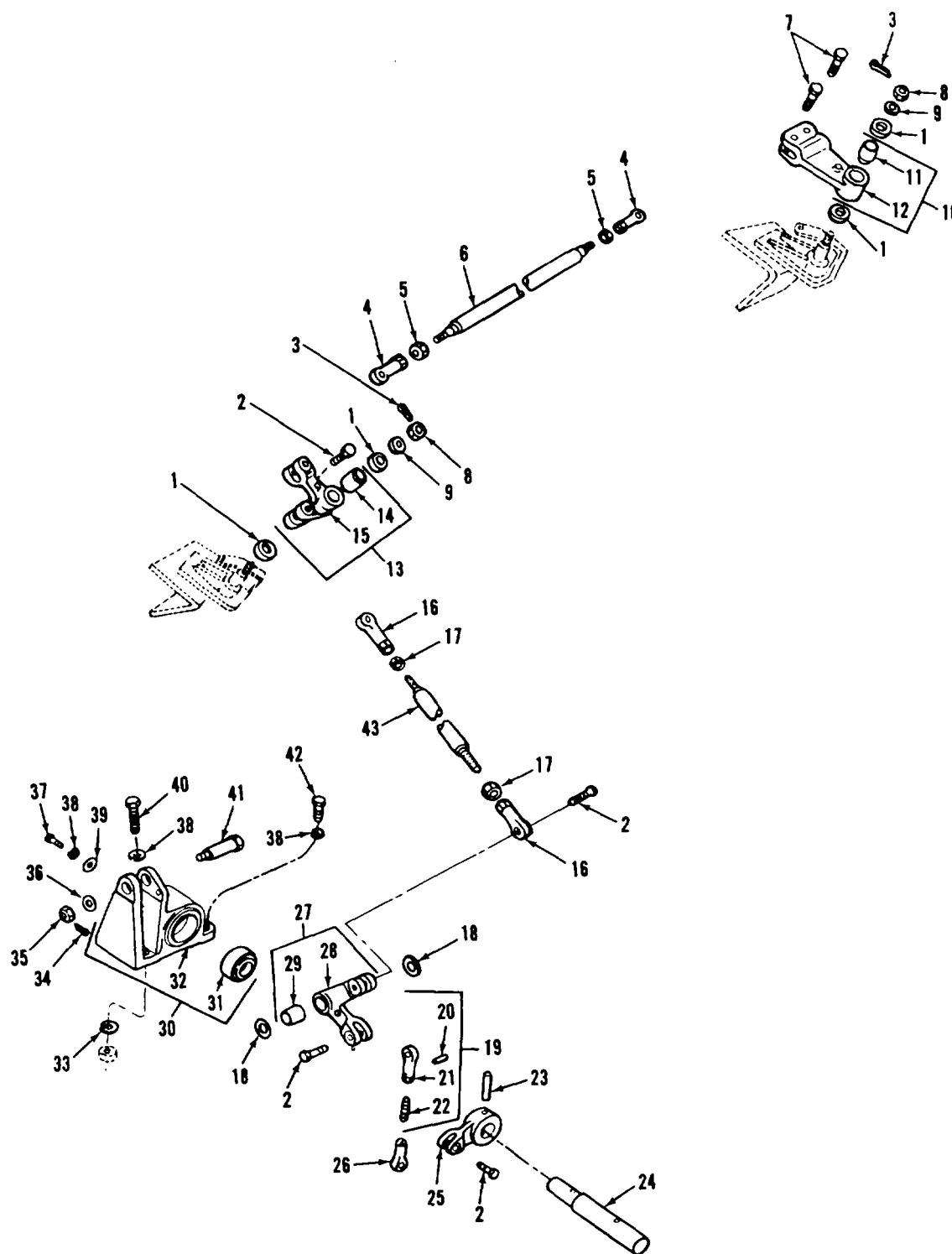
FIGURE 116. SHIFTING CONTROL LINKAGE AND RELATED PARTS (DRIVER'S COMPARTMENT)
