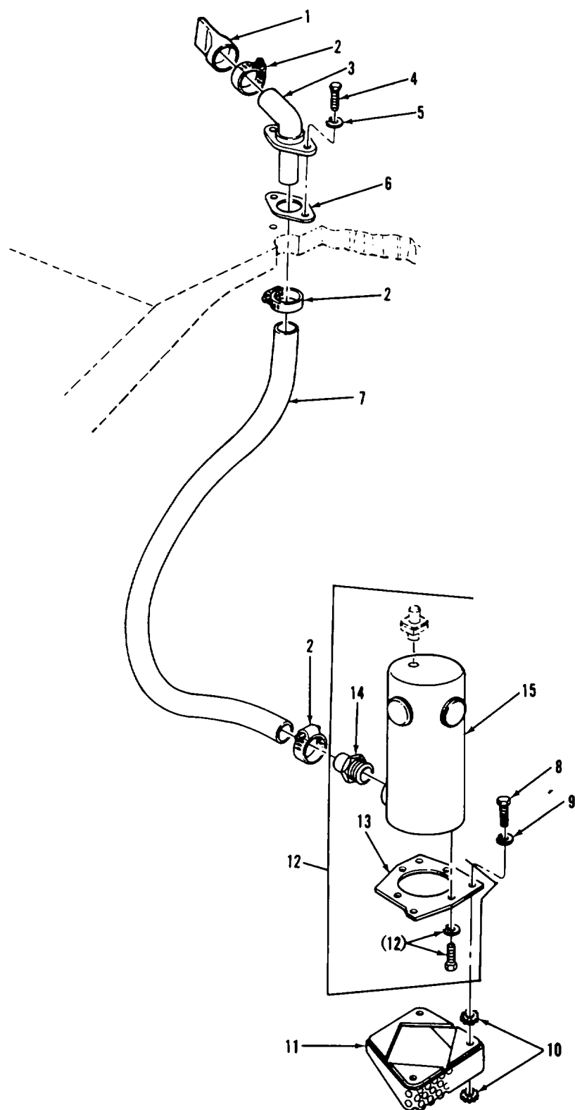
FIGURE 185. BILGE PUMP, COMPONENTS, AND RELATED PARTS
