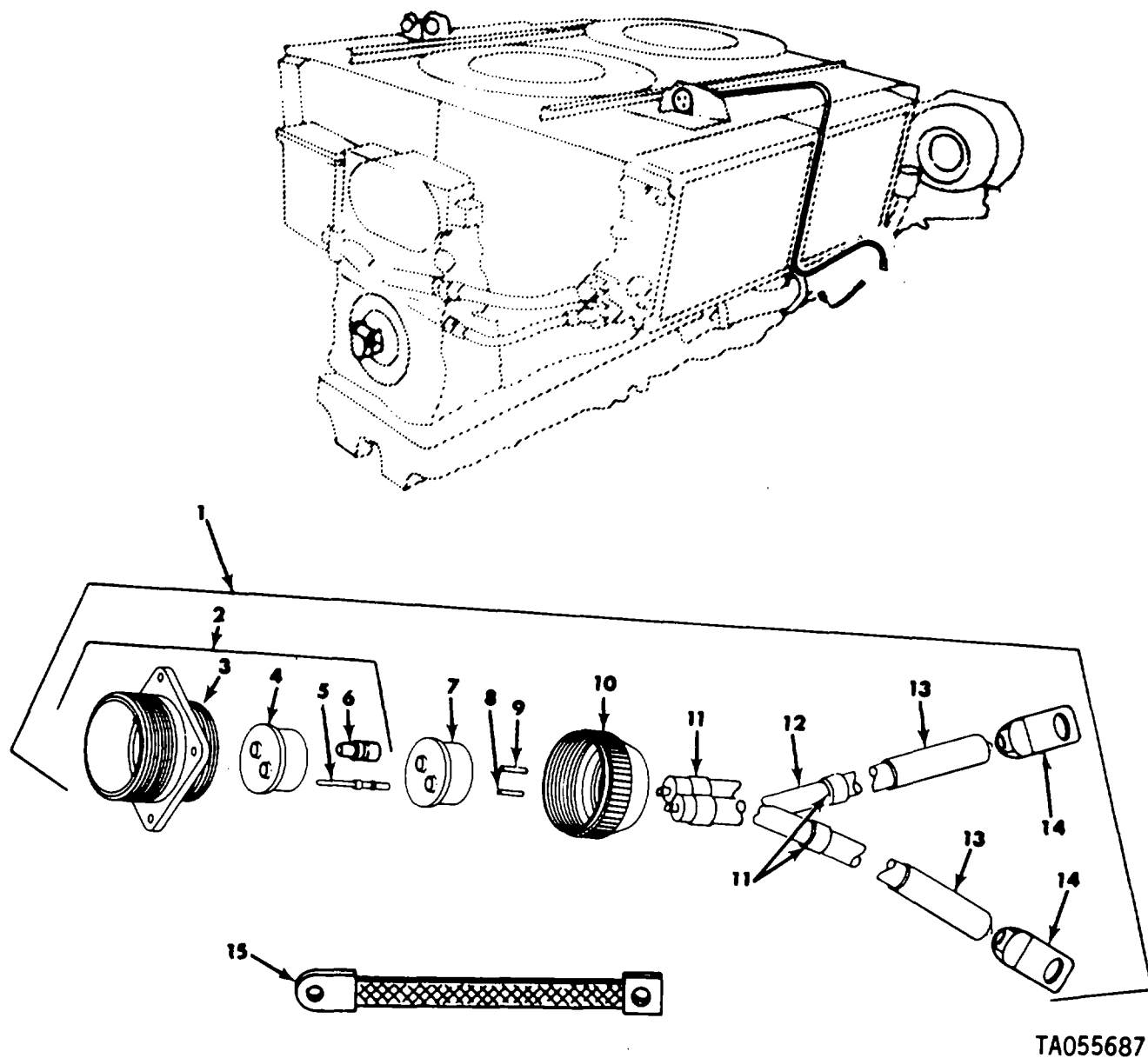
FIGURE 110. GENERATOR BLOWER LEAD ASSEMBLY AND COMPONENTS
