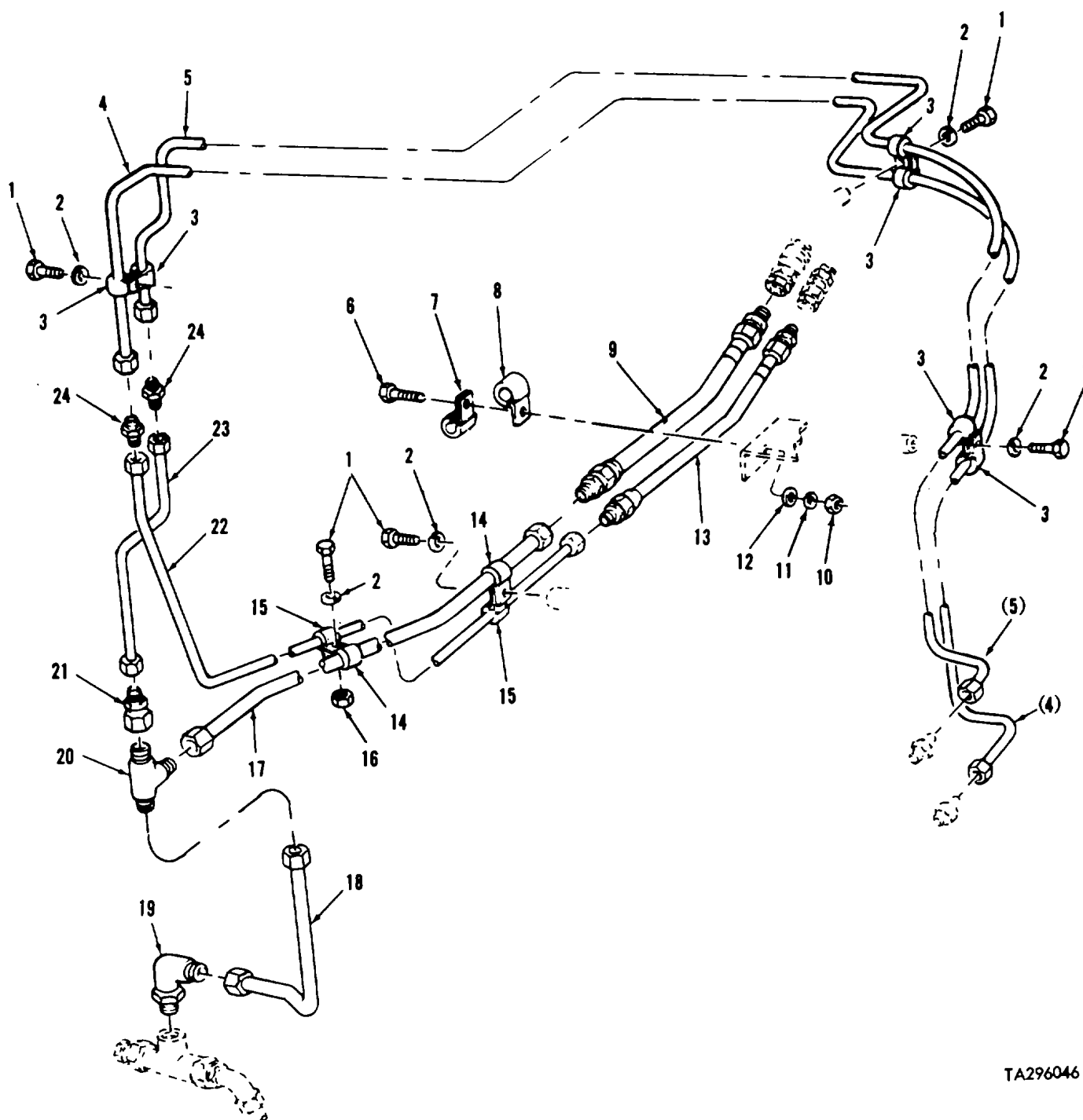
FIGURE 40. REAR PRIMER PUMP FUEL SUPPLY LINES AND RELATED PARTS
