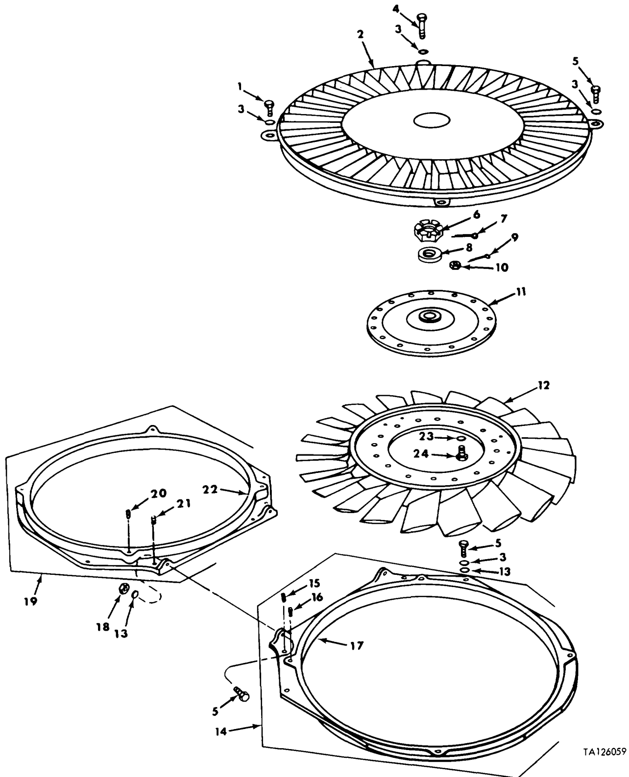
FIGURE 54. ENGINE COOLING FANS, VANES AND HOUSINGS AND RELATED PARTS
