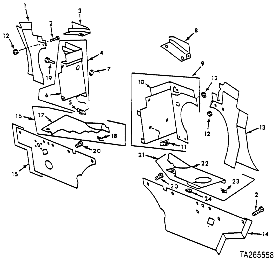
FIGURE 49. TURBOSUPERCHARGER AND TRANSMISSION SHROUDS AND RELATED PARTS
