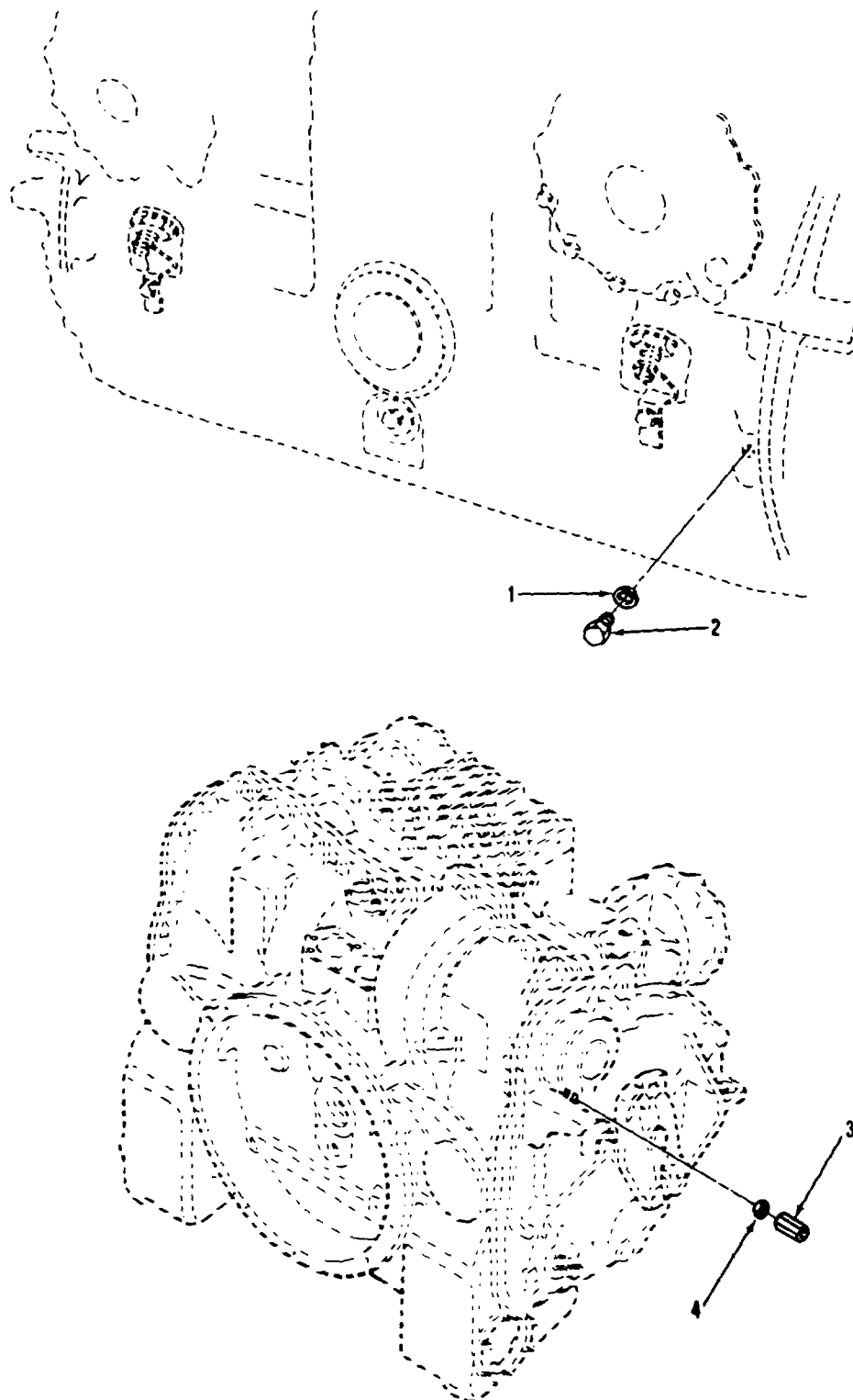
FIGURE 124. TRANSMISSION ASSEMBLY BRAKE ADJUSTING PARTS
