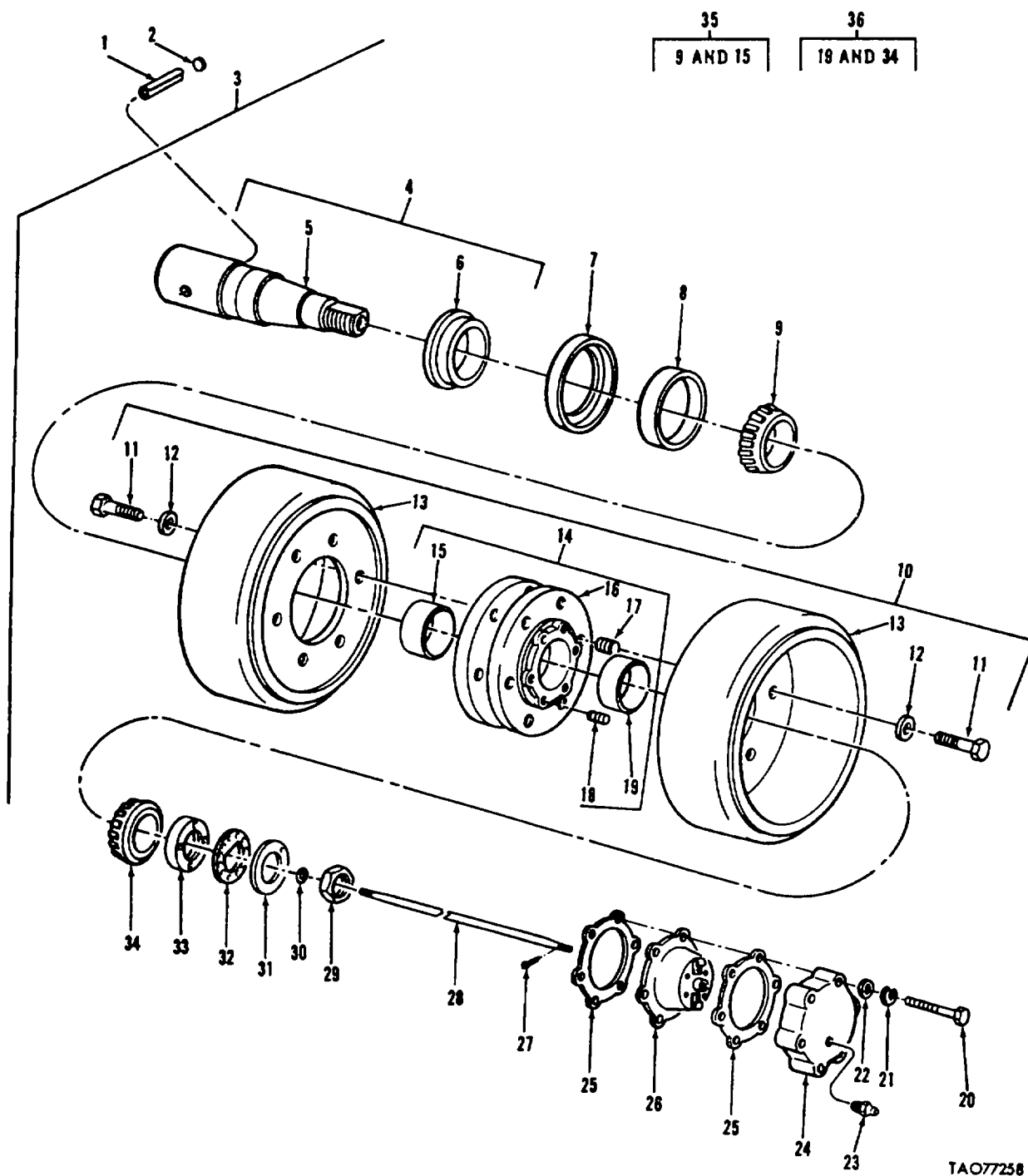
FIGURE 140. NO. 1 LEFT TRACK SUPPORT ROLLER ASSEMBLY, COMPONENTS, AND RELATED PARTS
