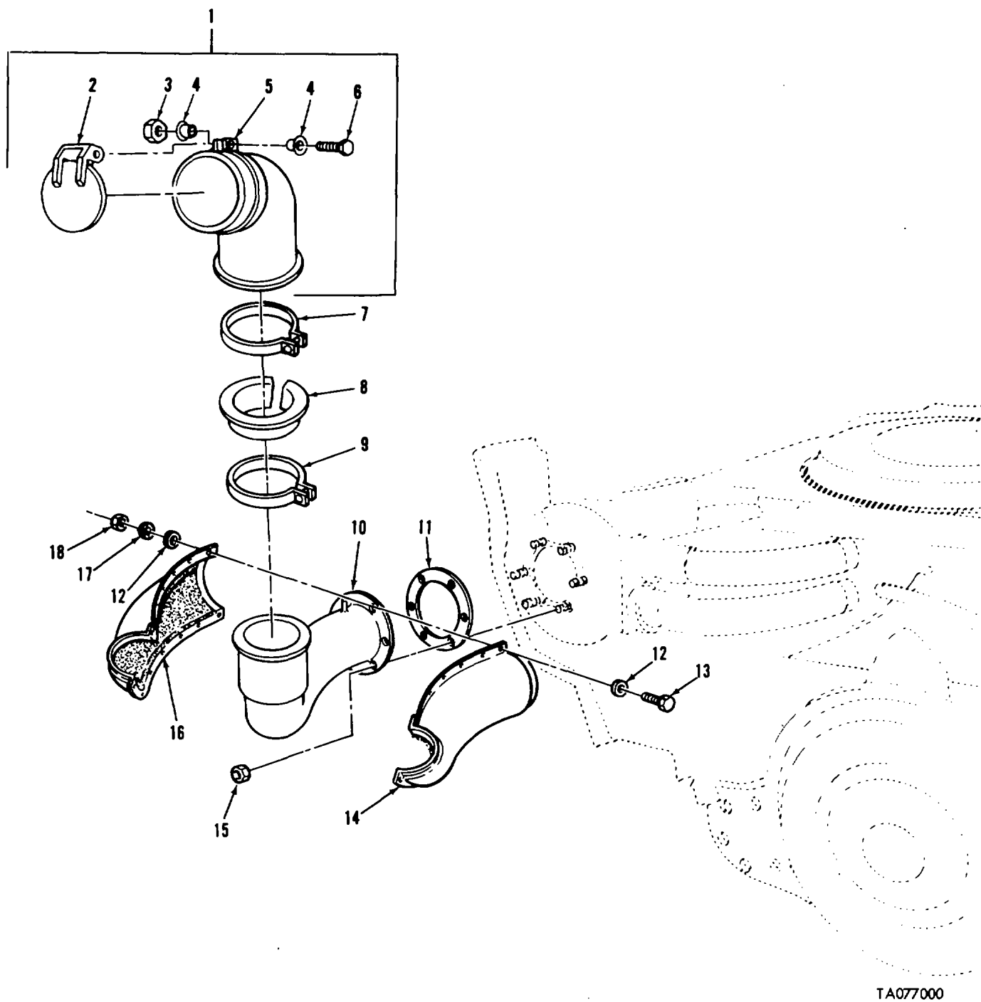
FIGURE 46. ENGINE EXHAUST PIPES AND RELATED PARTS
