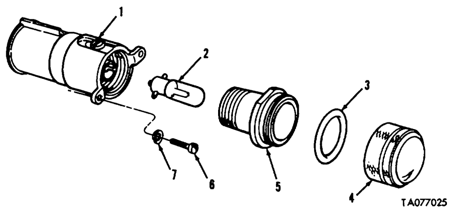
FIGURE 77. POWER PLANT MASTER WARNING LIGHT AND RELATED PARTS
