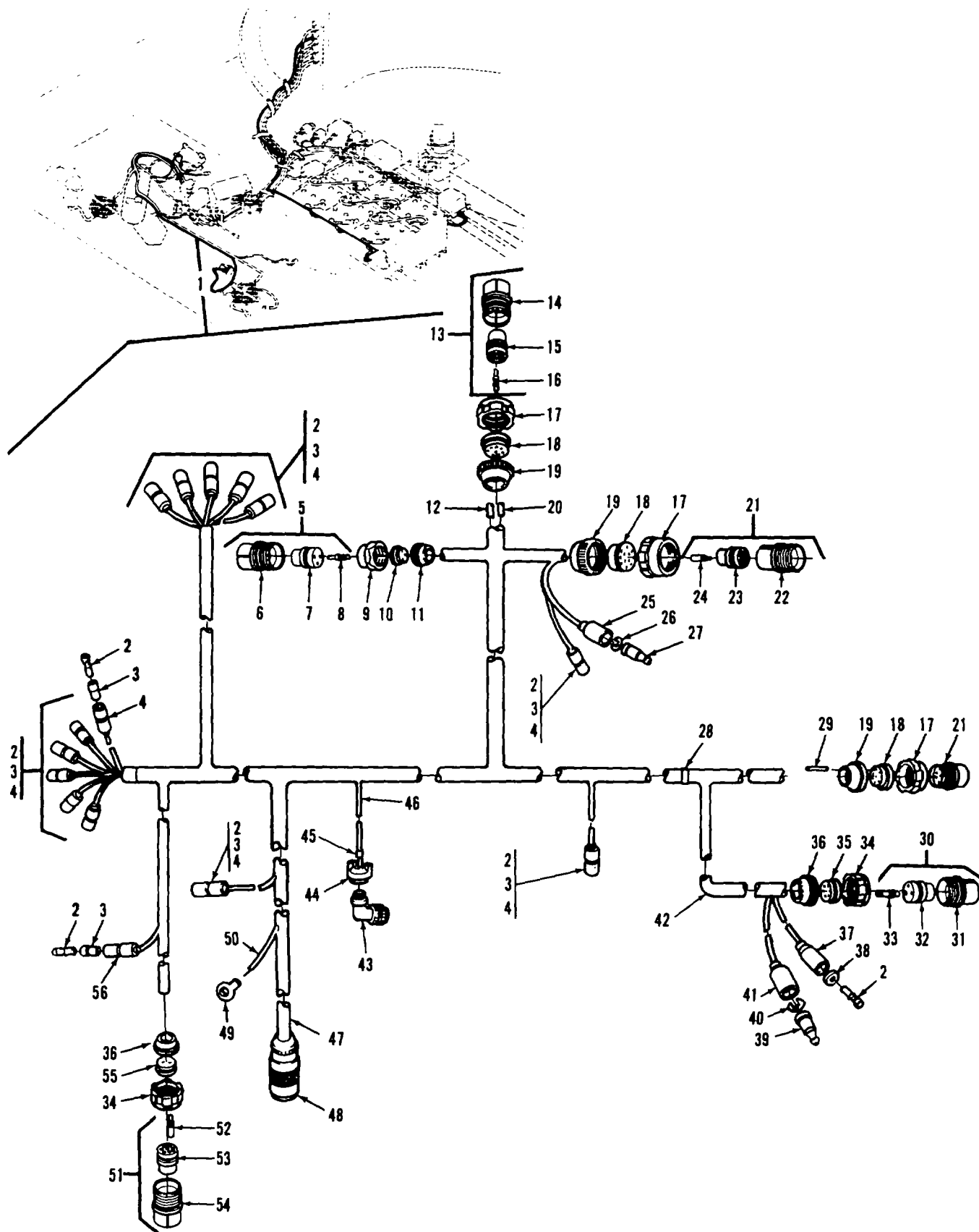
FIGURE 96. FRONT ACCESSORY WIRING HARNESS ASSEMBLY AND COMPONENTES
