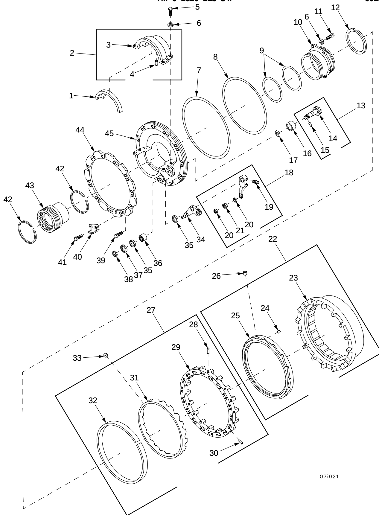
Figure 24. Left Output Reduction Mounting Saddles
