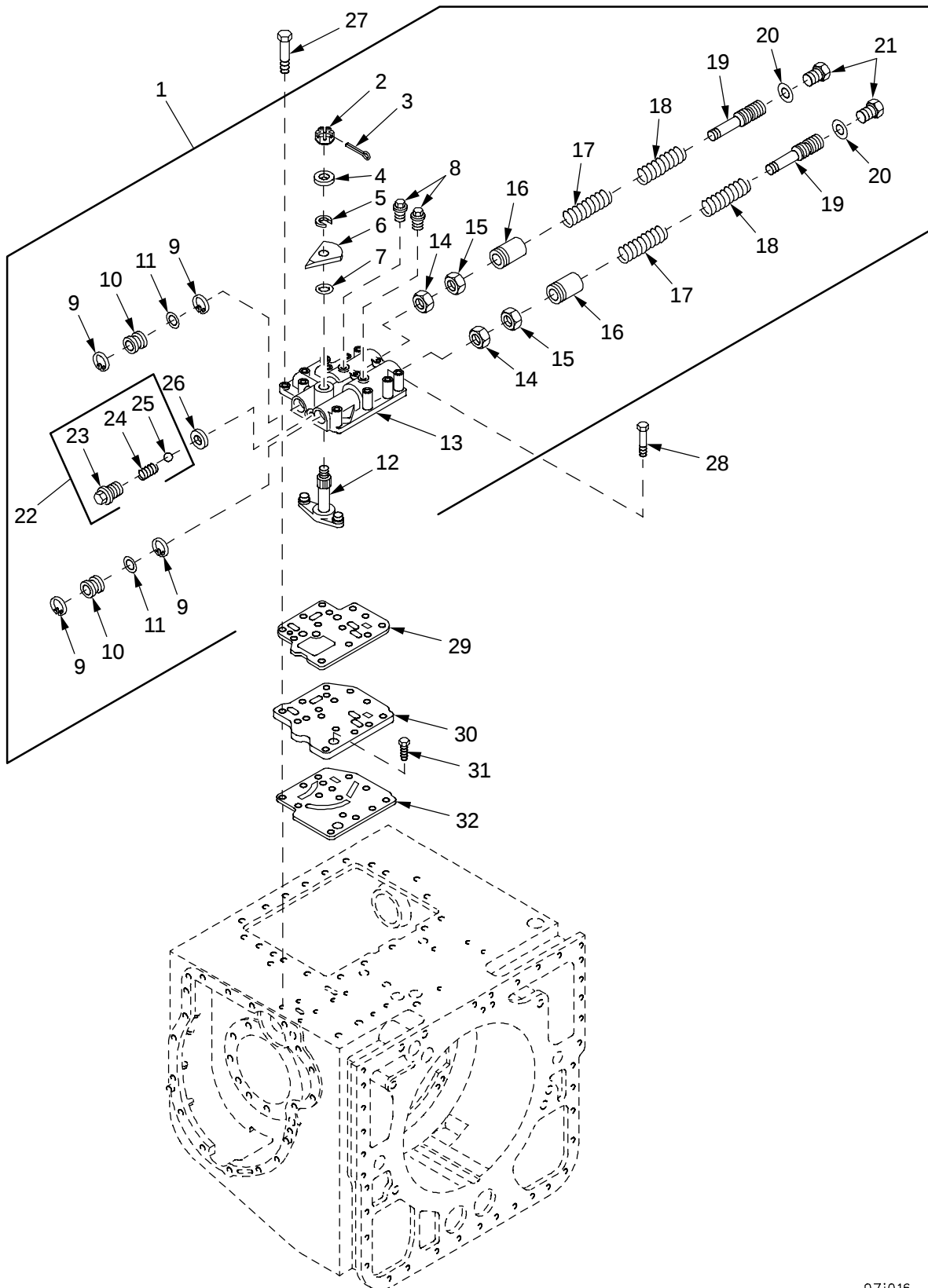
Figure 17. Transmission Steering Control Valve
