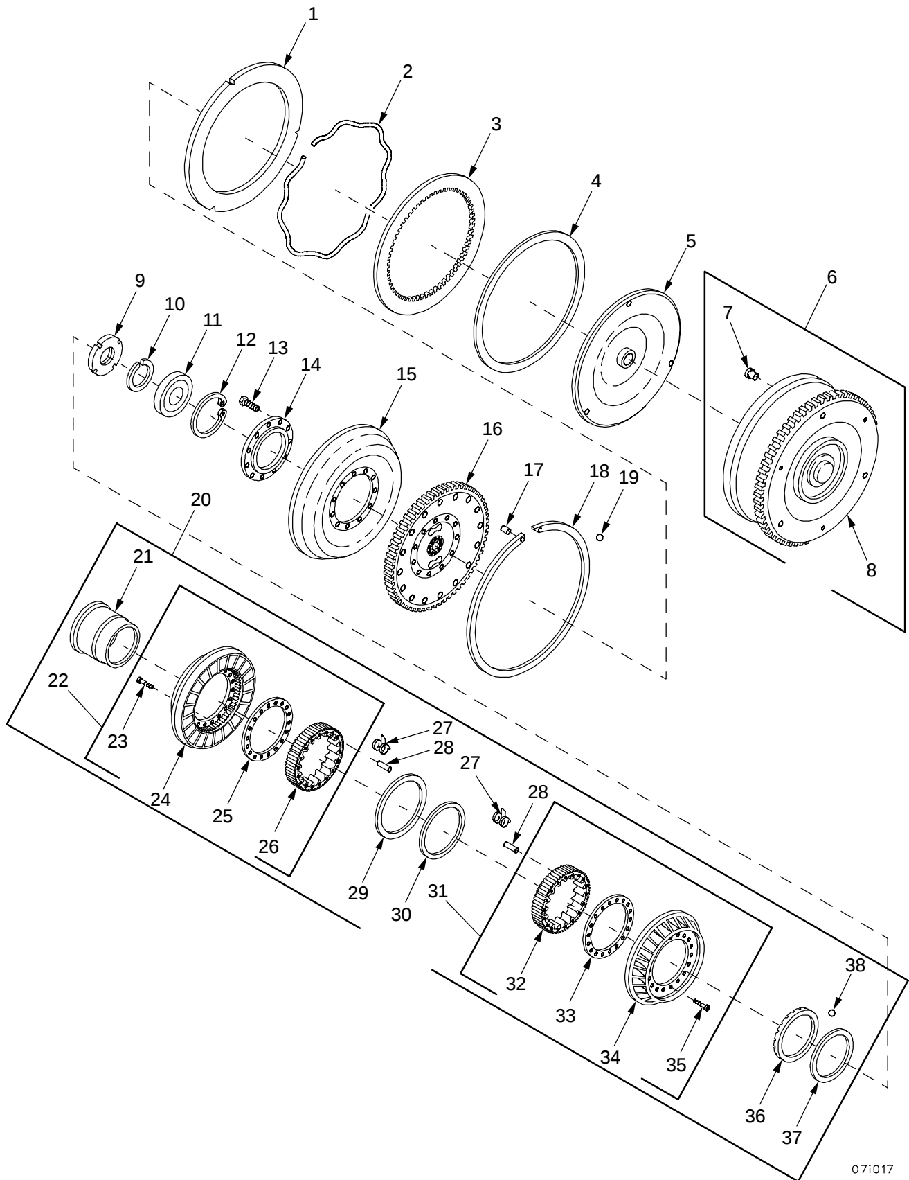
Figure 1. Torque Converter Positive Clutch and Stator
