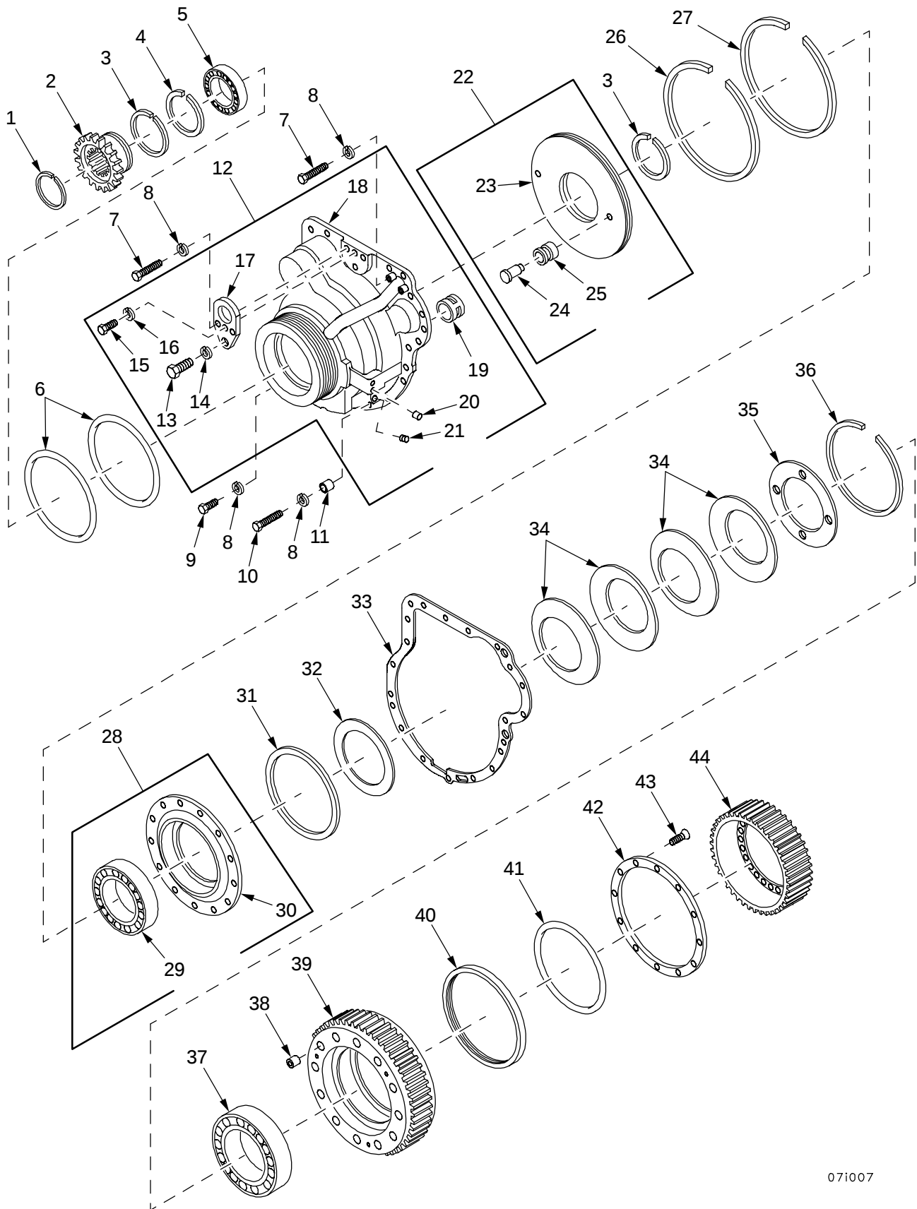
Figure 20. Right Steering Clutch
