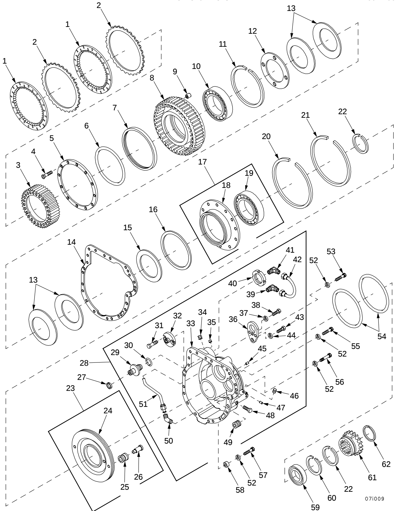
Figure 23. Left Steering Clutch and Drive Gear
