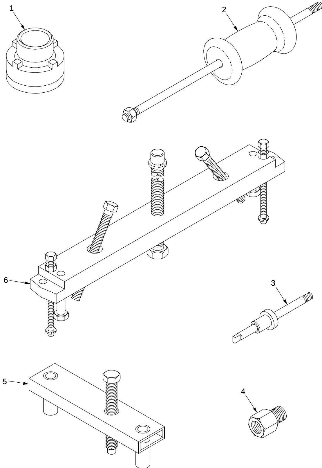
Figure 34. Special Tools
