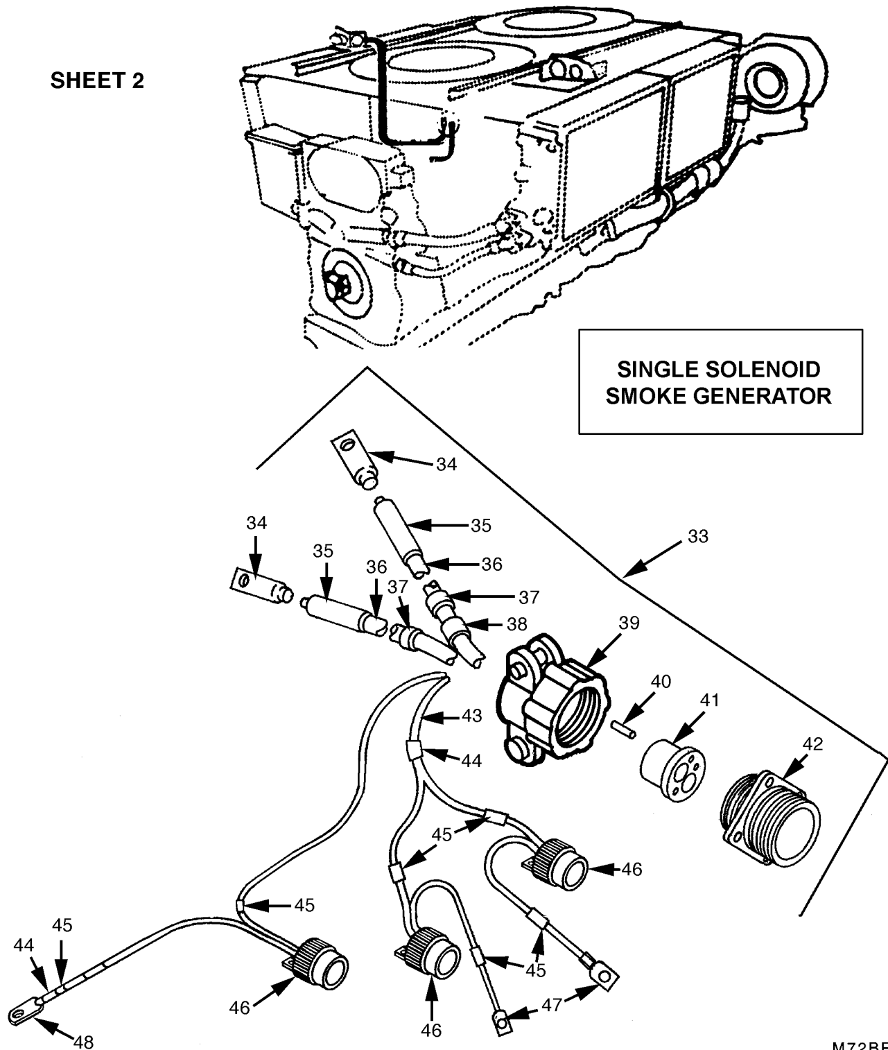
FIGURE 72. STARTER/SMOKE GENERATOR AND DUST DETECTOR WIRING HARNESS (MODELS AVDS-1790-2CA AND AVDS-1790-2DA; SHEET 2 OF 2)
