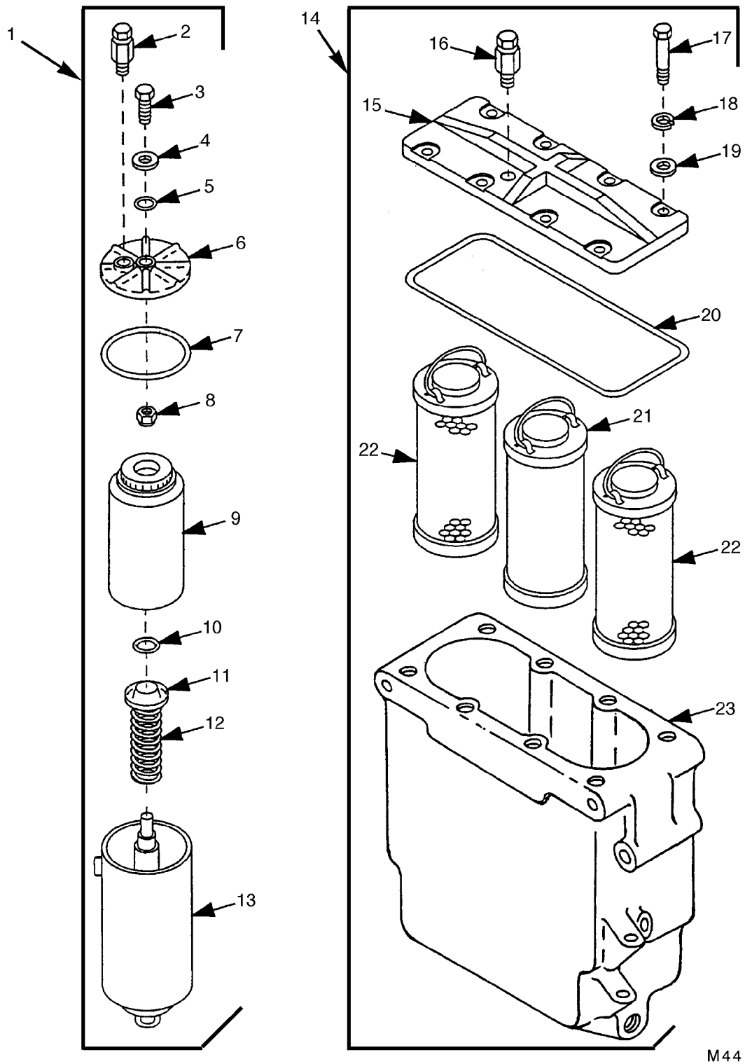
FIGURE 46. PRIMARY AND WATER SEPARATOR FUEL FILTER ASSEMBLIES
