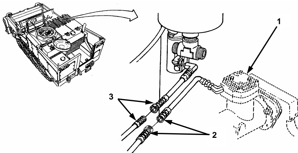
Figure 2-1. Quick-Disconnect Reinstall at Air Compressor
