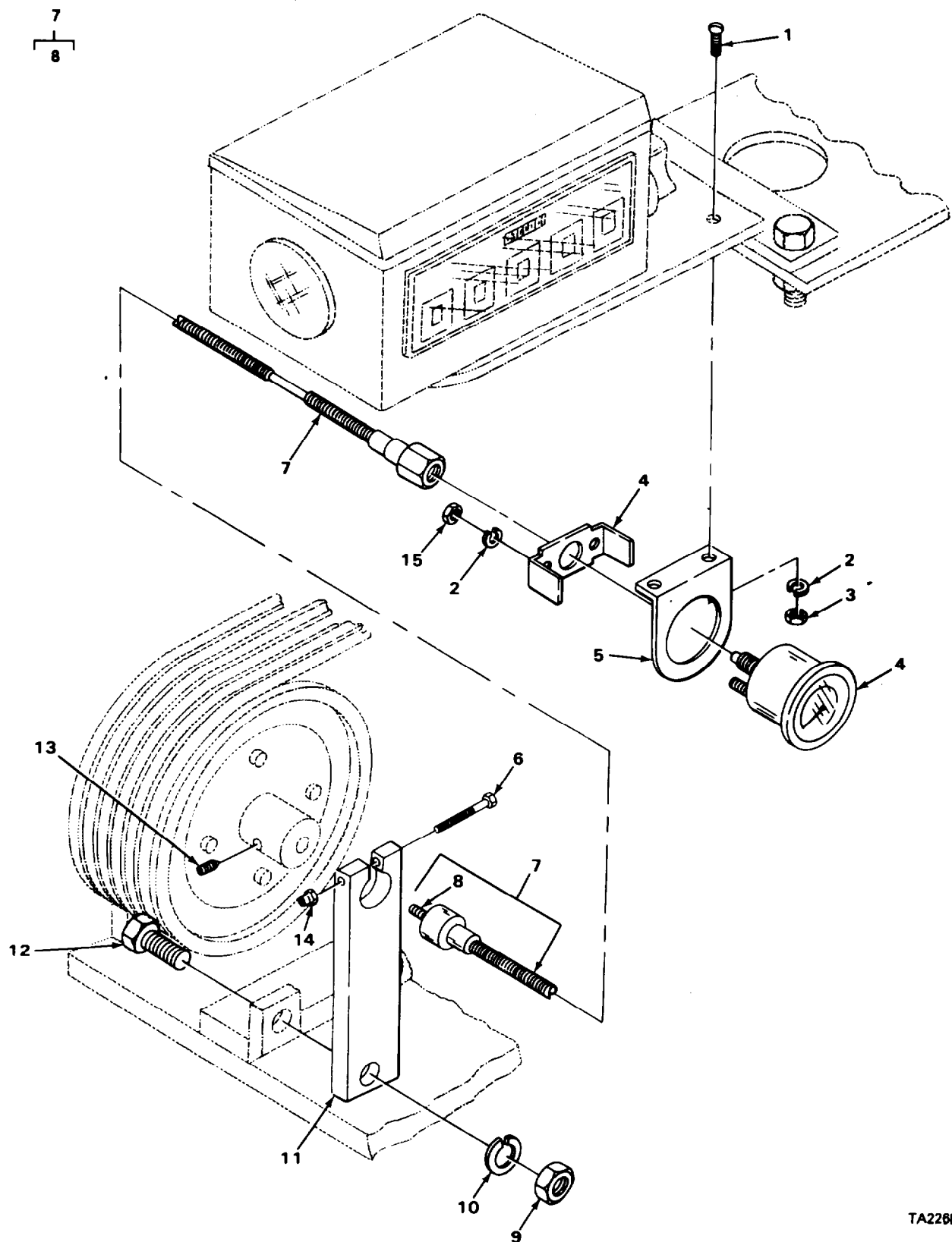
FIGURE 20. TACHOMETER.
