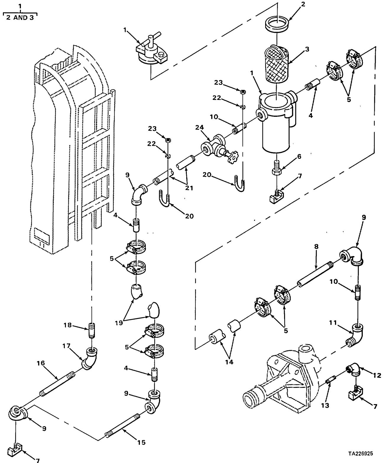
FIGURE 65. WATER SYSTEM LINES, TANK TO PUMP.
