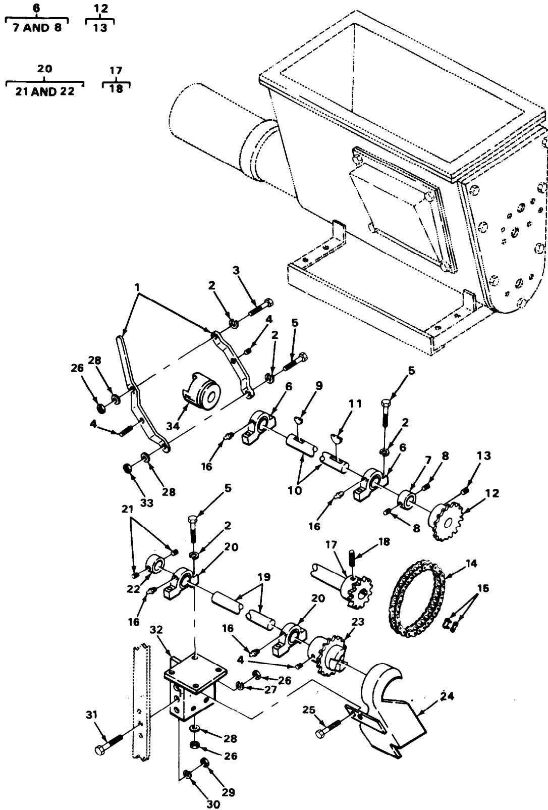
FIGURE 48. DRY ADMIX BIN DRIVE SYSTEM, BEARINGS AND SHAFT.
