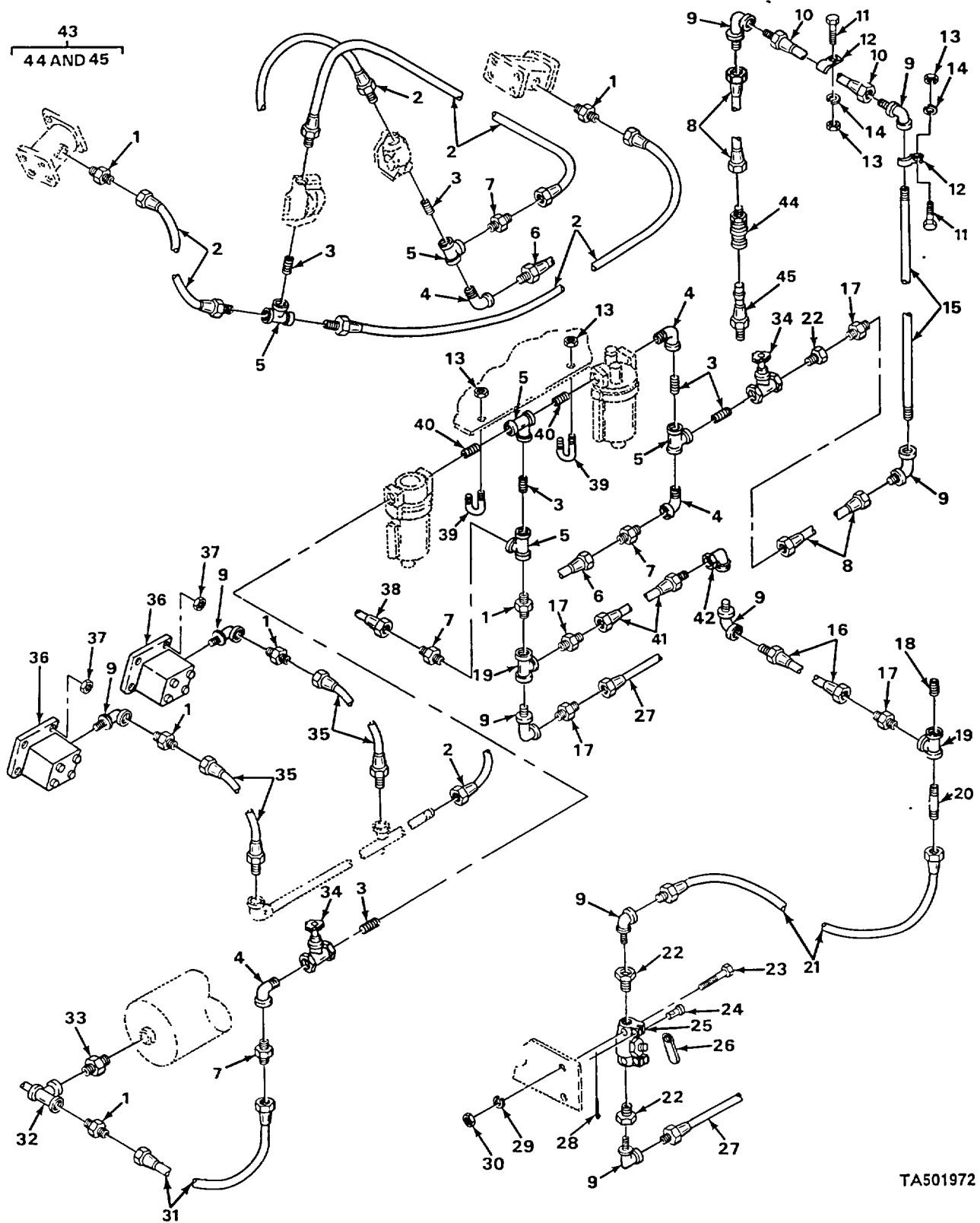
FIGURE 16. AIR SYSTEM LINES AND FITTINGS.
