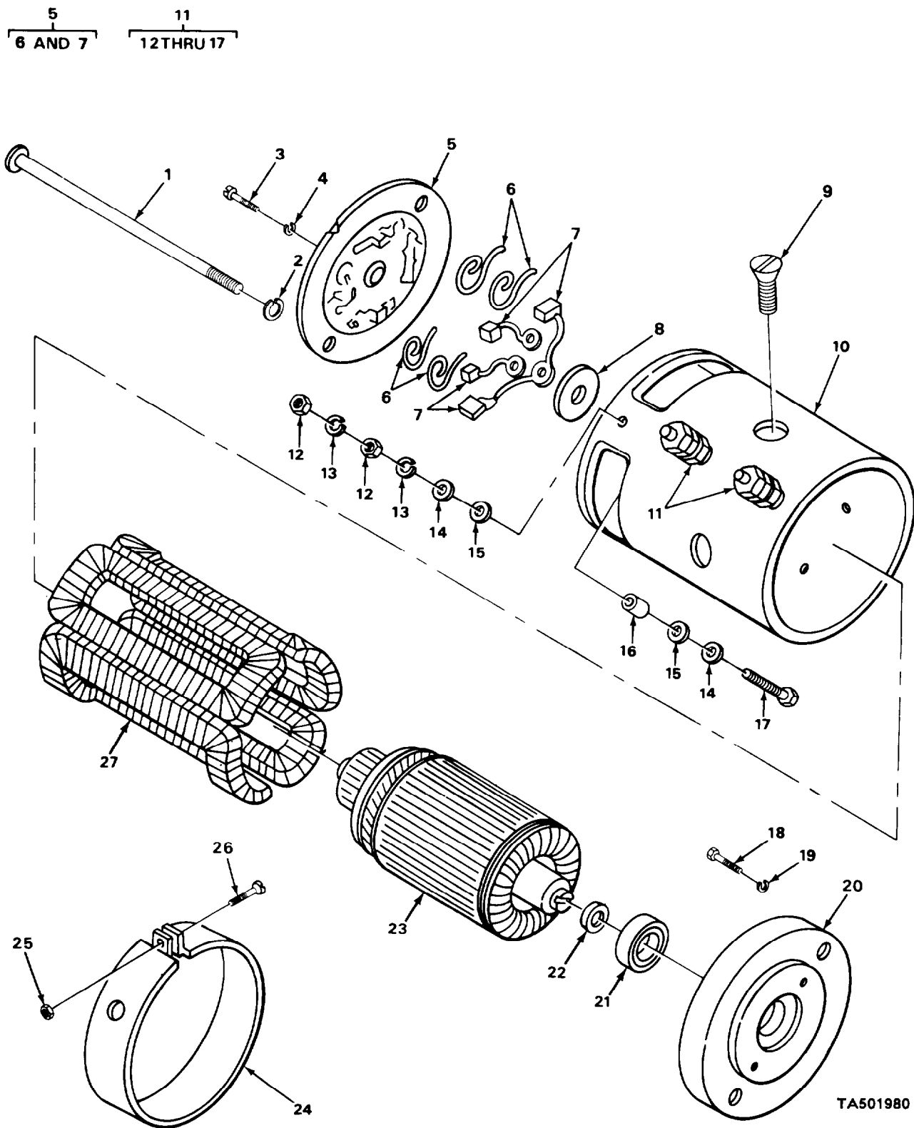
FIGURE 27. ELECTRIC WINCH MOTOR ASSEMBLY.
