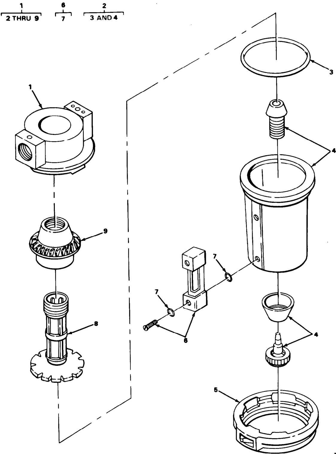
FIGURE 17. AIR SYSTEM FILTER.
