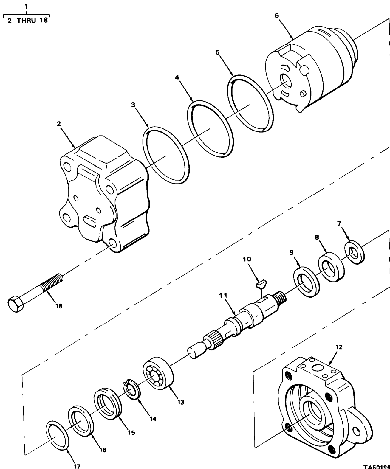
FIGURE 9. HYDRAULIC OIL PUMP ASSEMBLY.
