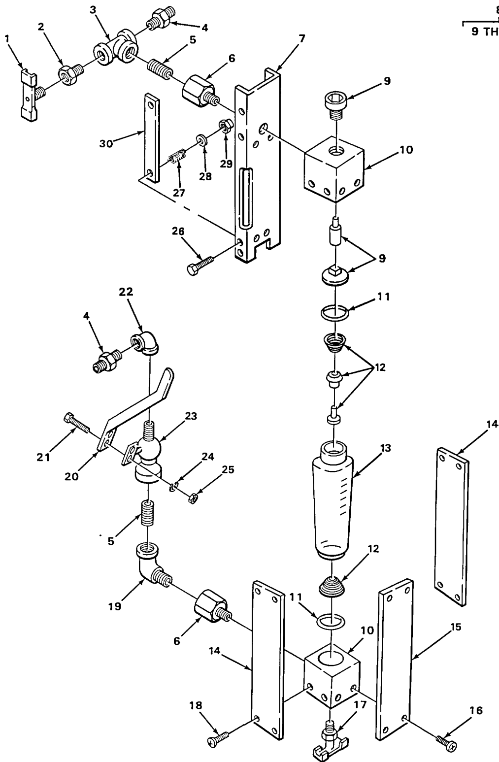
FIGURE 24. FLOW METER COMPONENT PARTS.
