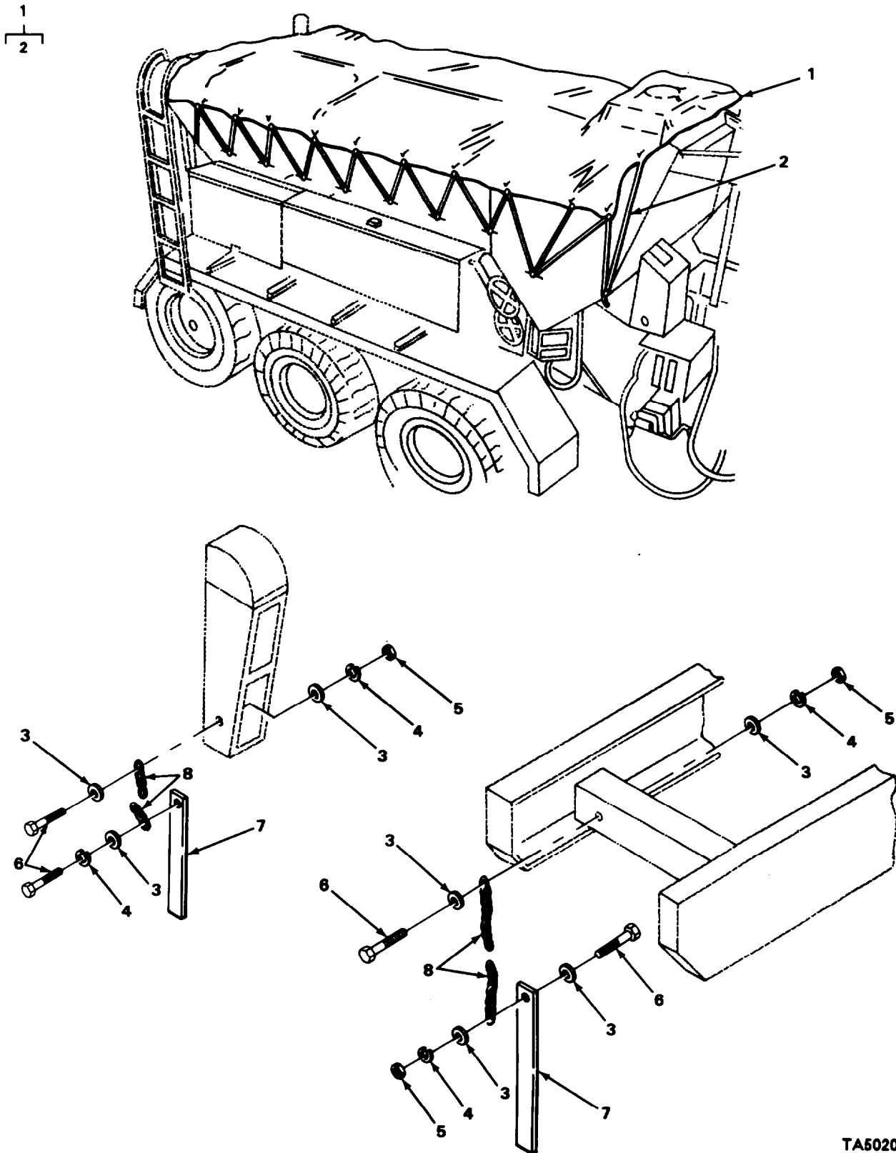
FIGURE 5. TARPAULIN AND GROUND STRAPS.
