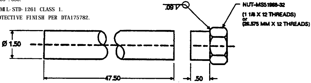
Figure E-8. PUSHROD DRIVER.
